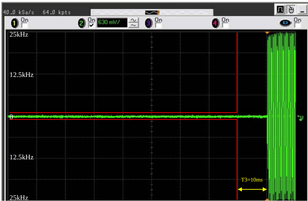
6I-4 – 467.775 MHz, 25 kHz Channel Spacing De-Key Decay Time
