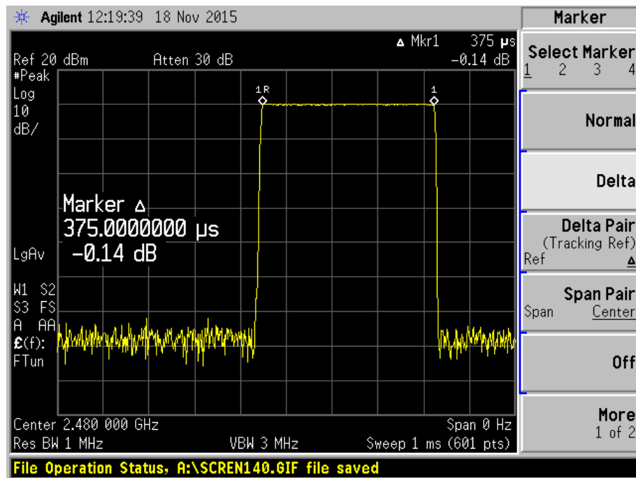
Plot 29 – Channel 78 (upper ch)
