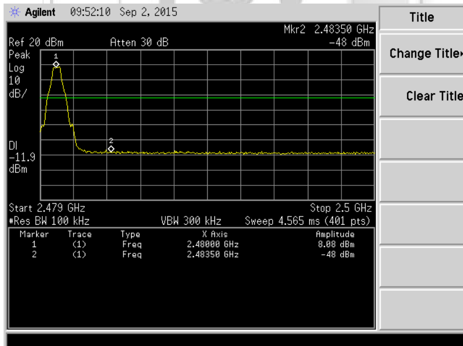
Plot 55 – Upper Band Edge at 2.4835GHz
