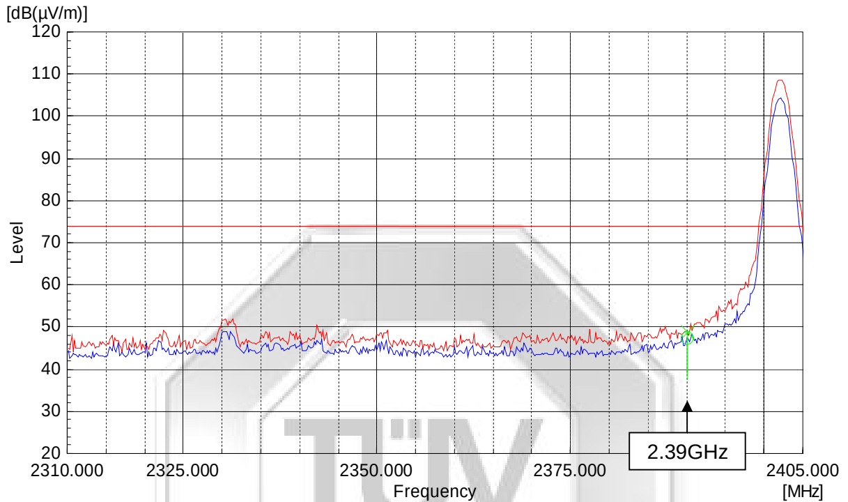
Plot 68 – Peak Plot at Lower Band Edge at 2.4000GHz
