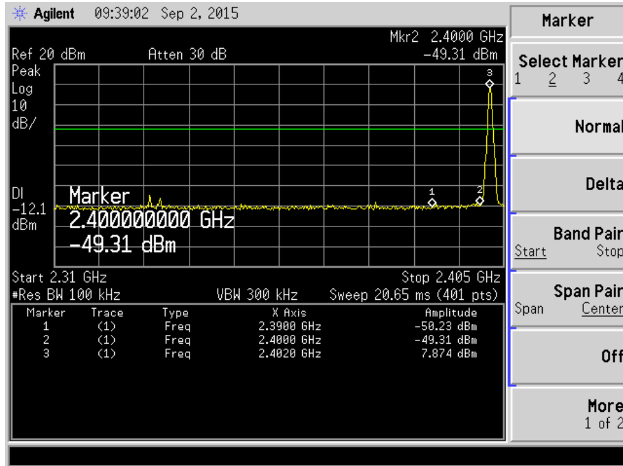
Plot 54 – Lower Band Edge at 2.4000GHz
