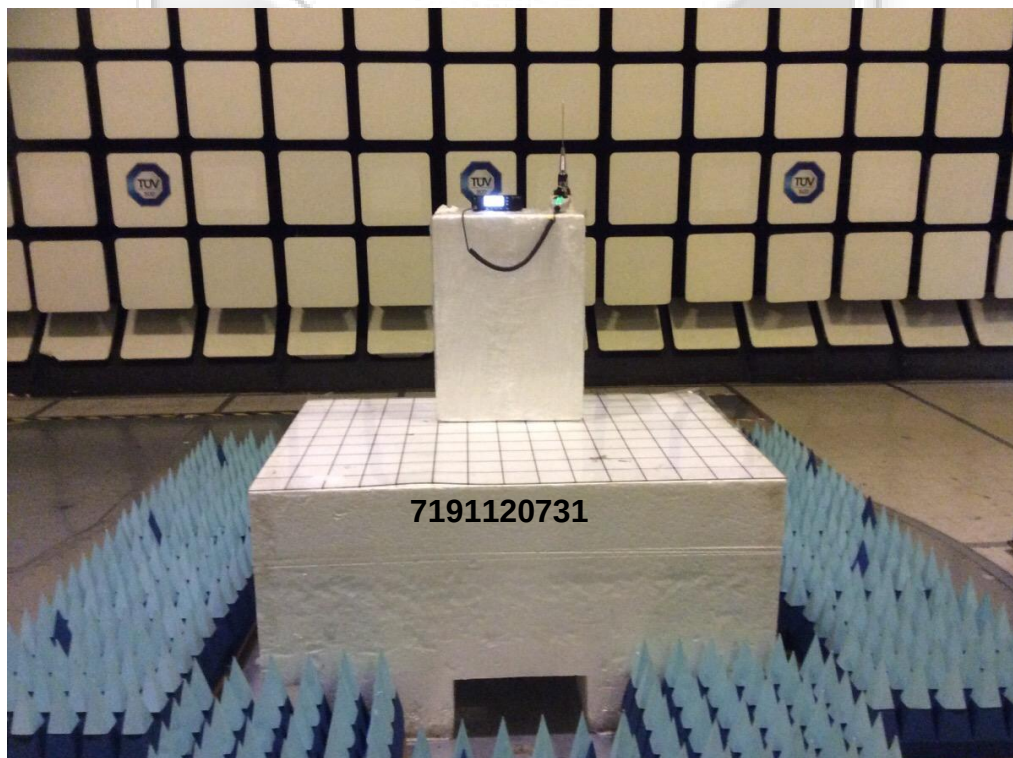
Band Edge Compliance (Radiated) Test Setup
