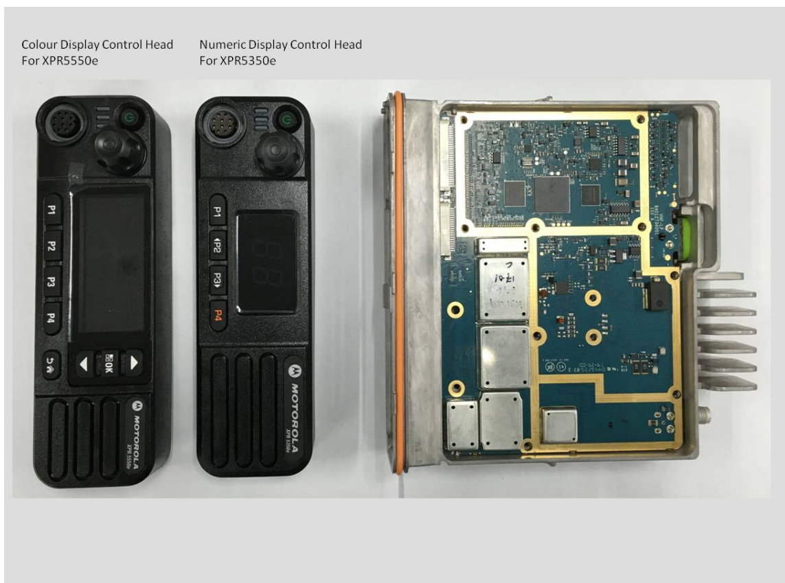
Chassis and control heads (Top)
