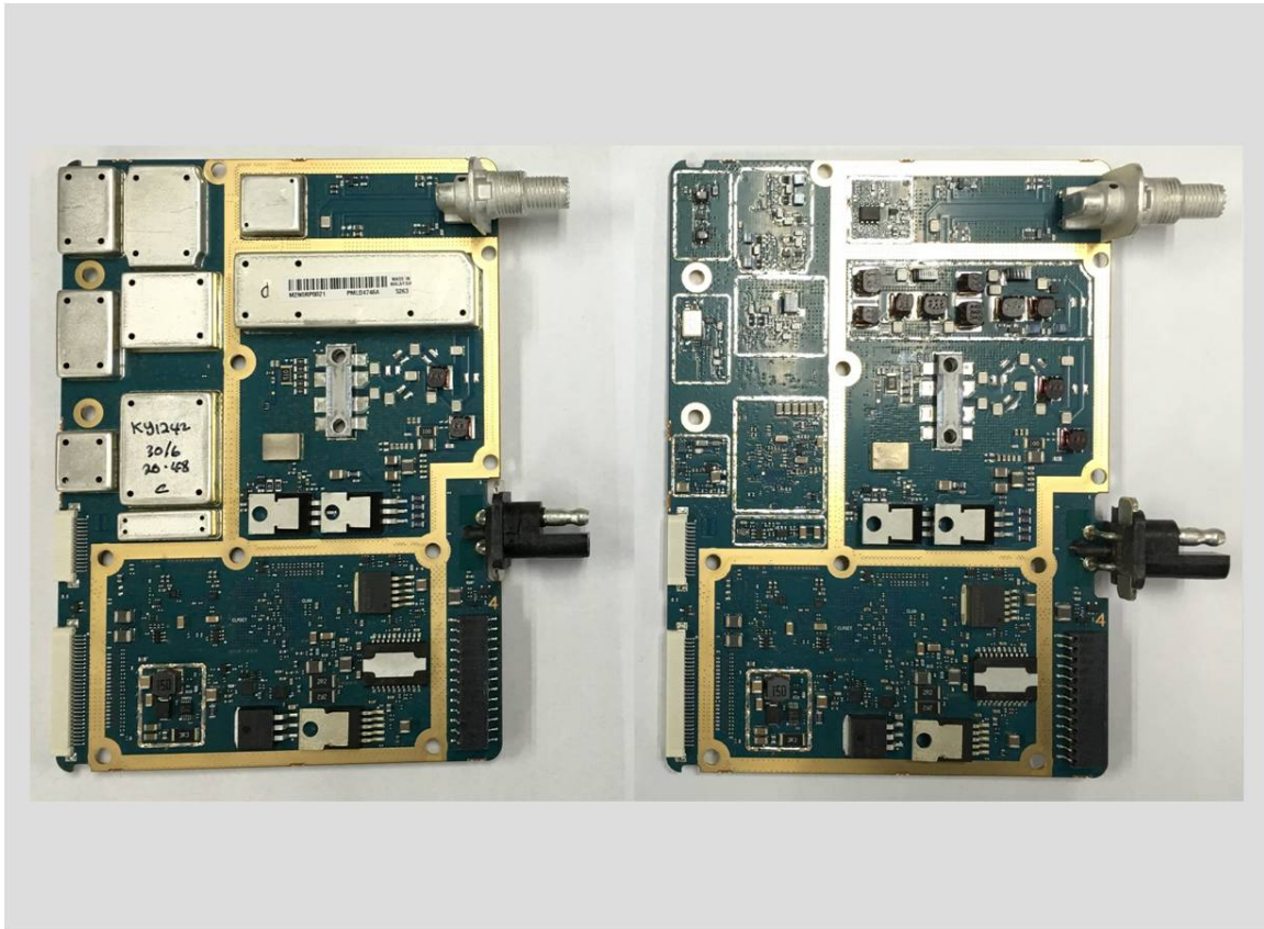
RF board with and without shields (Top)
