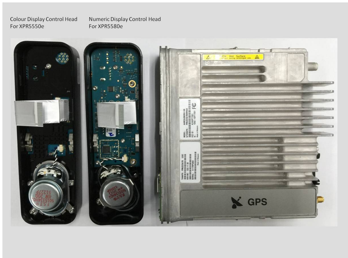
Chassis and control heads (Bottom)
