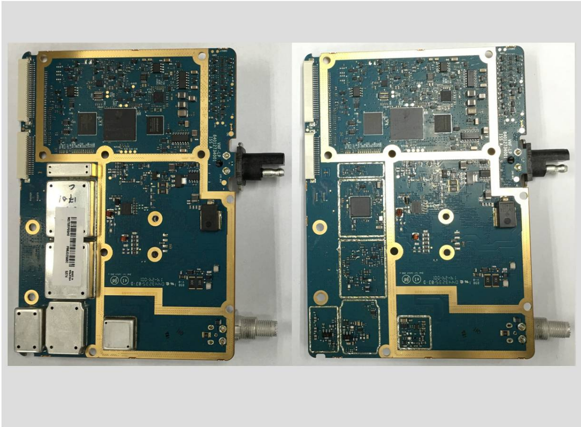
RF board with and without shields (Bottom)
