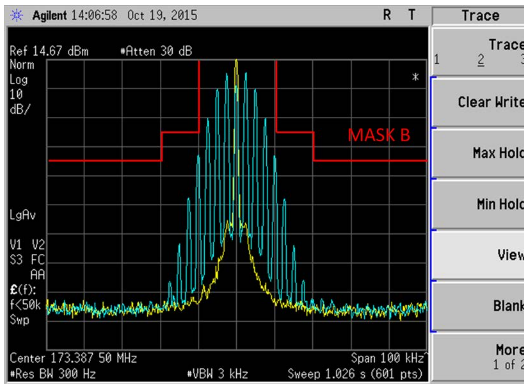
Figure 6E-16: 173.3875 MHz, 25 kHz Channel Spacing, 2500Hz Audio Modulation only, 16K0F3E Mask B (Not for FCC Review)
