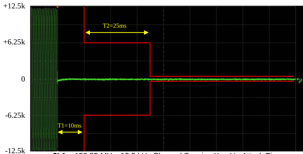
6I-1 – 158.55 MHz, 12.5 kHz Channel Spacing Key-Up Attack Time
