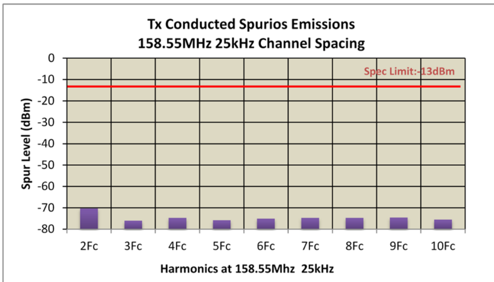
Figure 6F-5: 1W Harmonic of Carrier 158.55 MHz, 25 kHz Channel Spacing (Part 22, 80)
