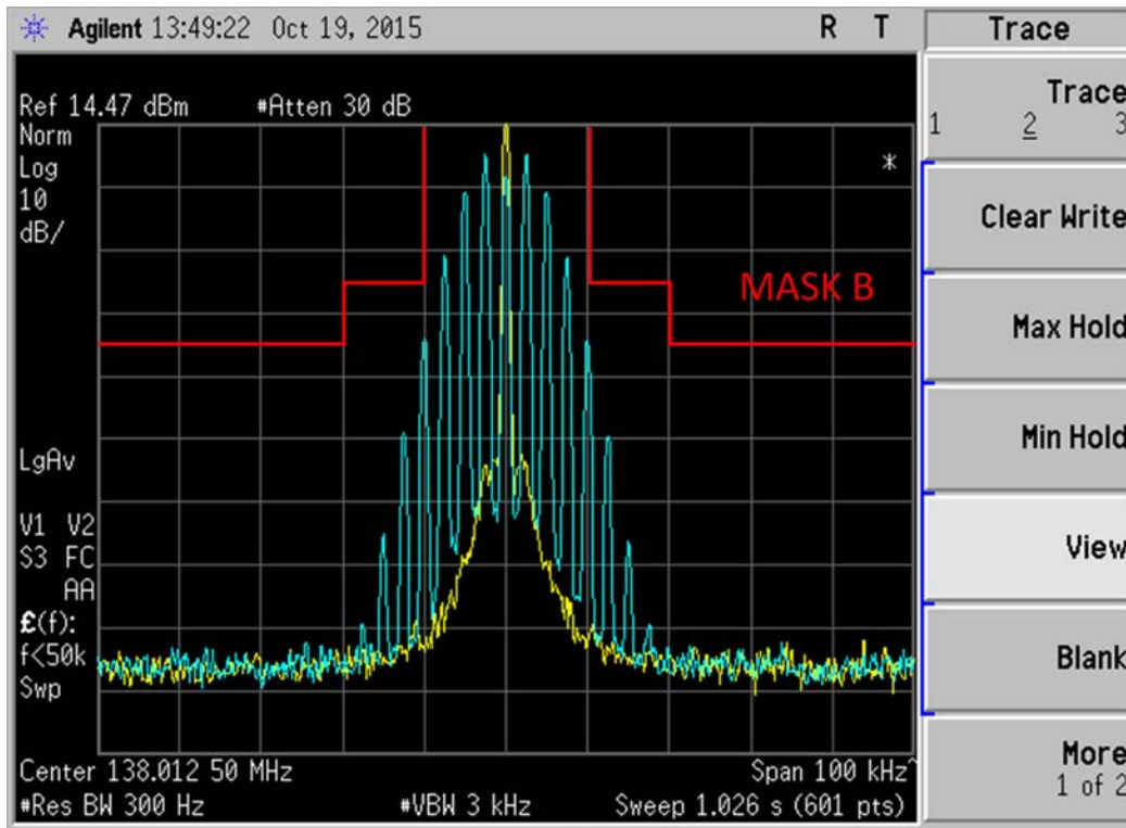
Figure 6E-13: 138.0125 MHz, 25 kHz Channel Spacing, 2500Hz Audio Modulation only, 16K0F3E Mask B (Not for FCC Review)
