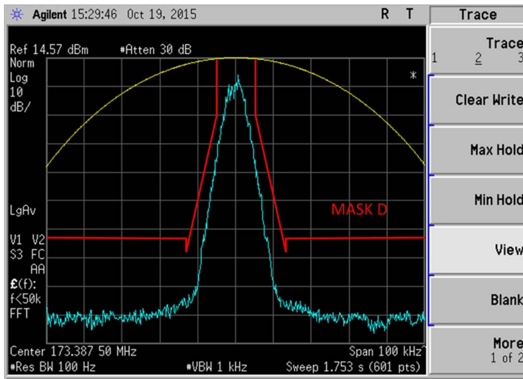
Figure 6E-10: 173.3875MHz, O.153 Test Pattern 4FSK Voice and Data Modulation, 7K60F1W Mask D
