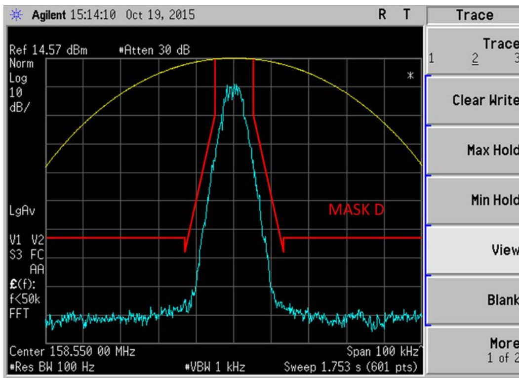
Figure 6E-8: 158.55 MHz, O.153 Test Pattern 4FSK Voice Modulation only, 7K60F1E Mask D
