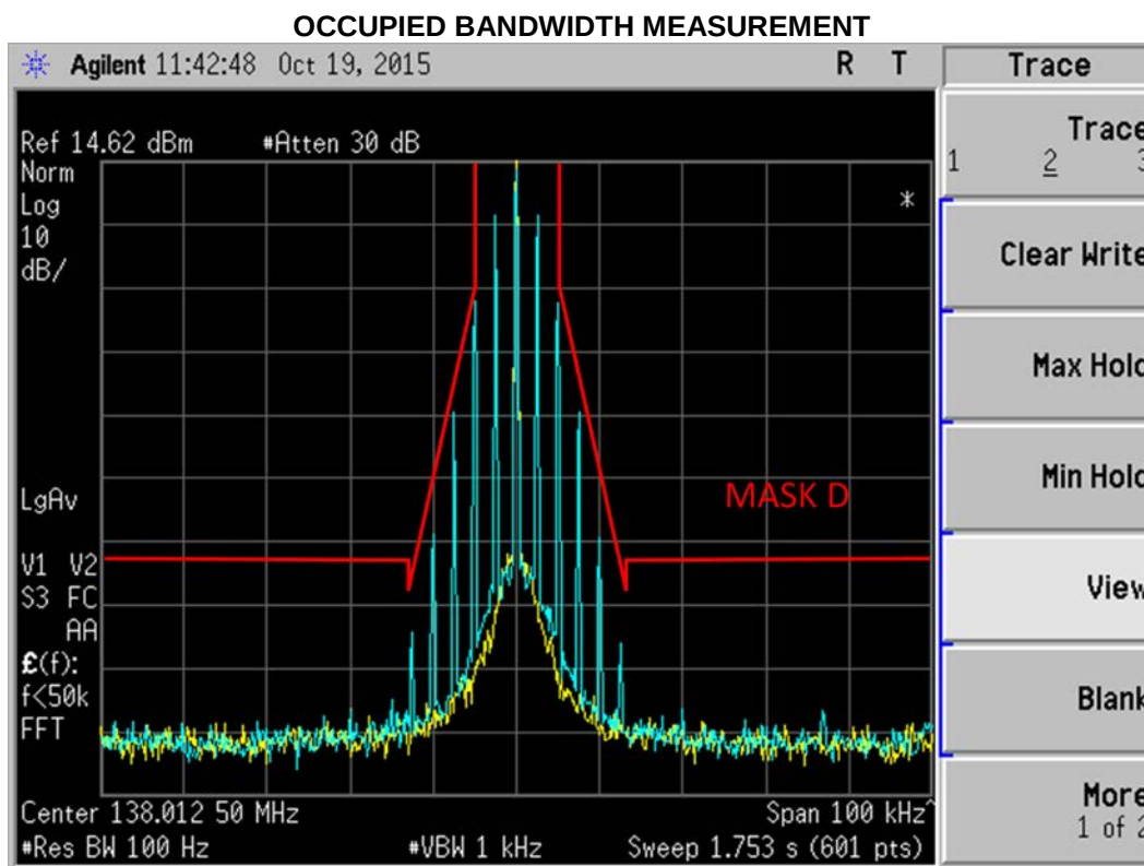
Figure 6E-1: 138.0125 MHz, 12.5 kHz Channel Spacing, 2500Hz Audio Modulation only, 11K0F3E Mask D (Not for FCC Review)
