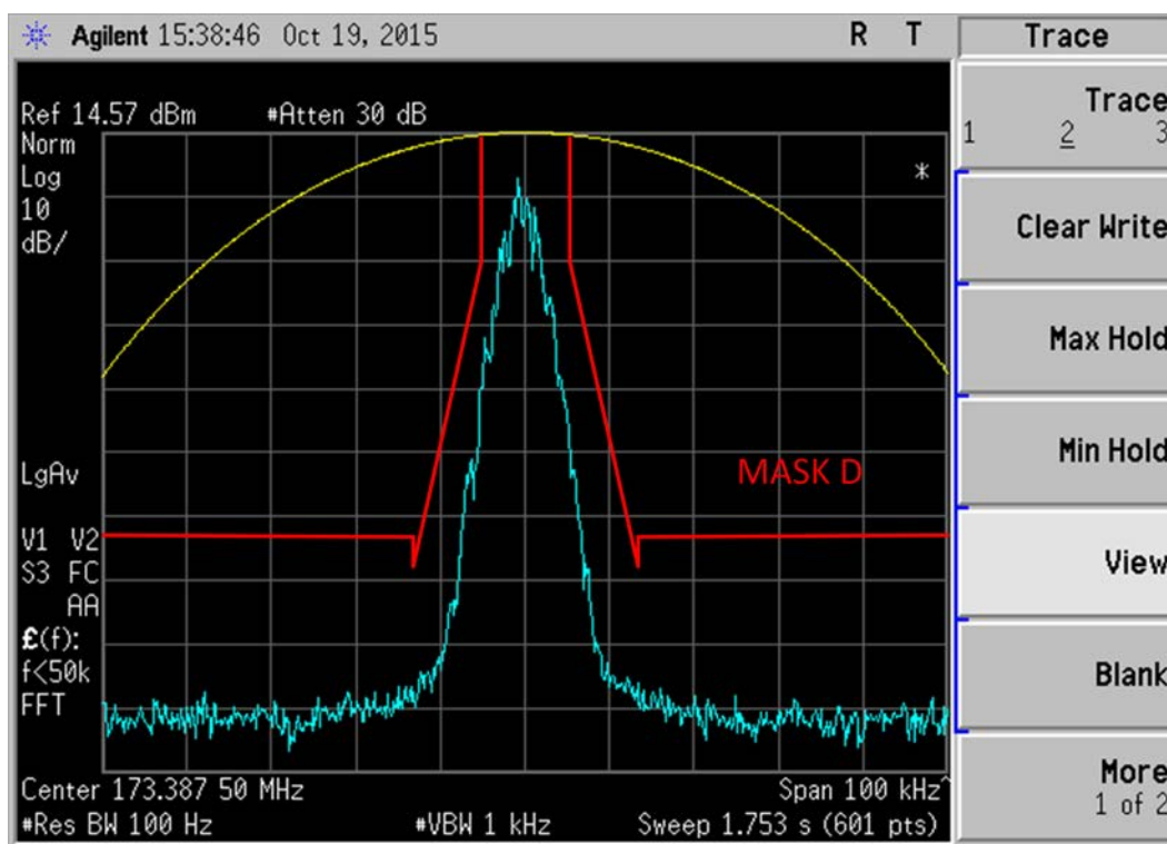
Figure 6E-11: 173.3875MHz, O.153 Test Pattern 4FSK Data Modulation only, 7K60F1D Mask D
