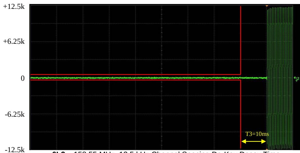
6I-2 – 158.55 MHz, 12.5 kHz Channel Spacing De-Key Decay Time
