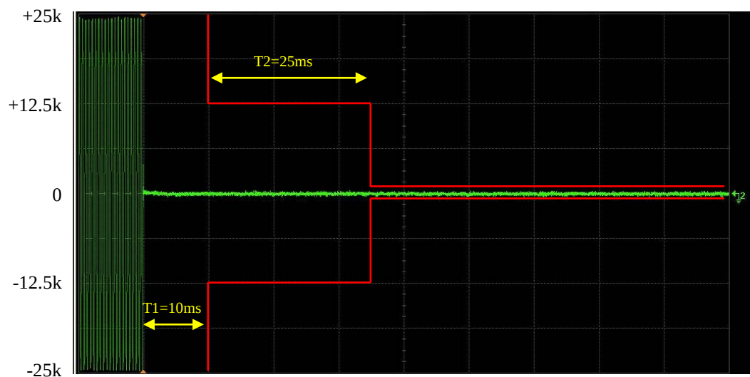
6I-3 – 158.55 MHz, 25 kHz Channel Spacing Key-Up Attack Time (Part 22, 80)
