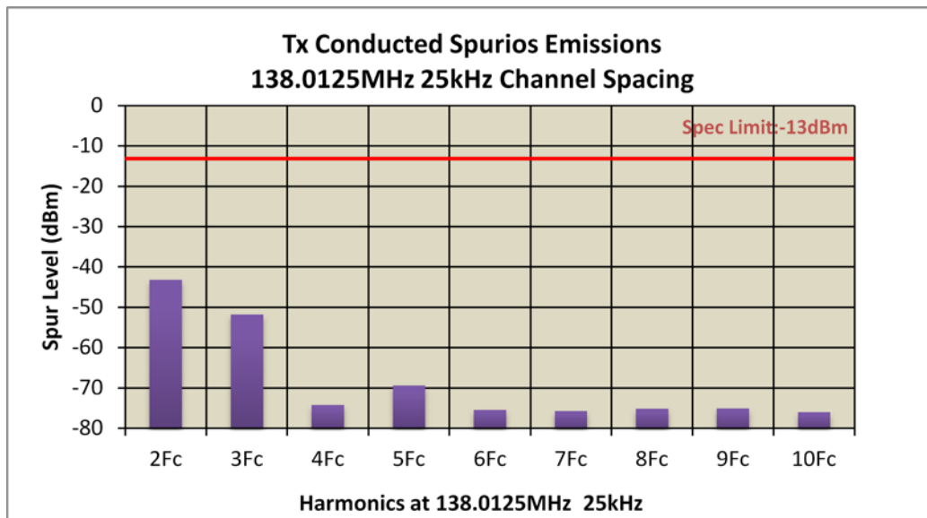
Figure 6F-1: 30 W Harmonic of Carrier 138.0125 MHz, 25 kHz Channel Spacing (Not for FCC Review)
