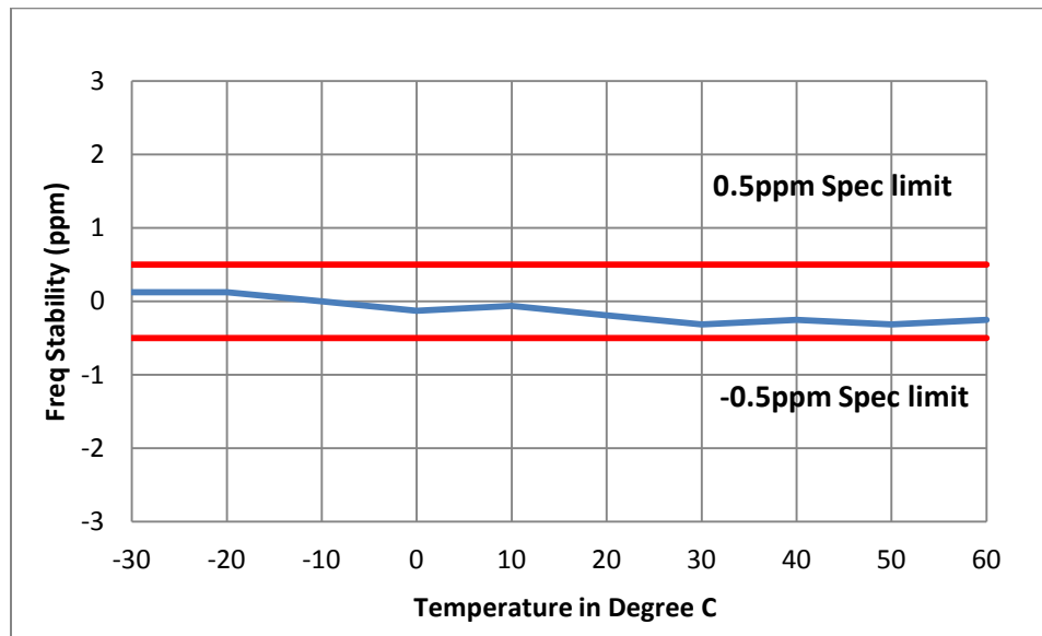
6H-1 – 158.55 MHz Frequency Stability vs. Temperature
