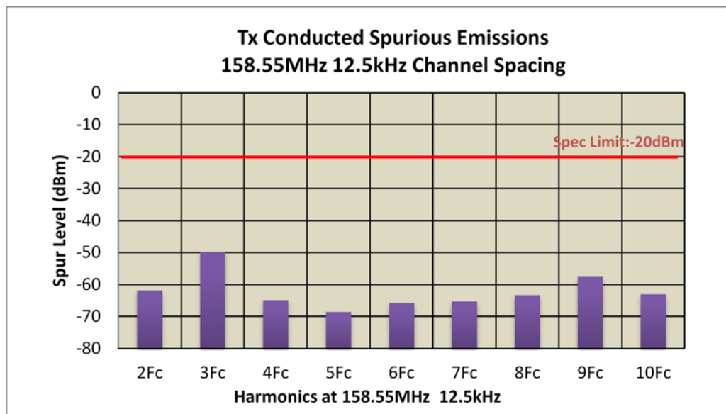
Figure 6F-8: 30 W Harmonic of Carrier 158.55 MHz, Digital 12.5 kHz Channel Spacing
