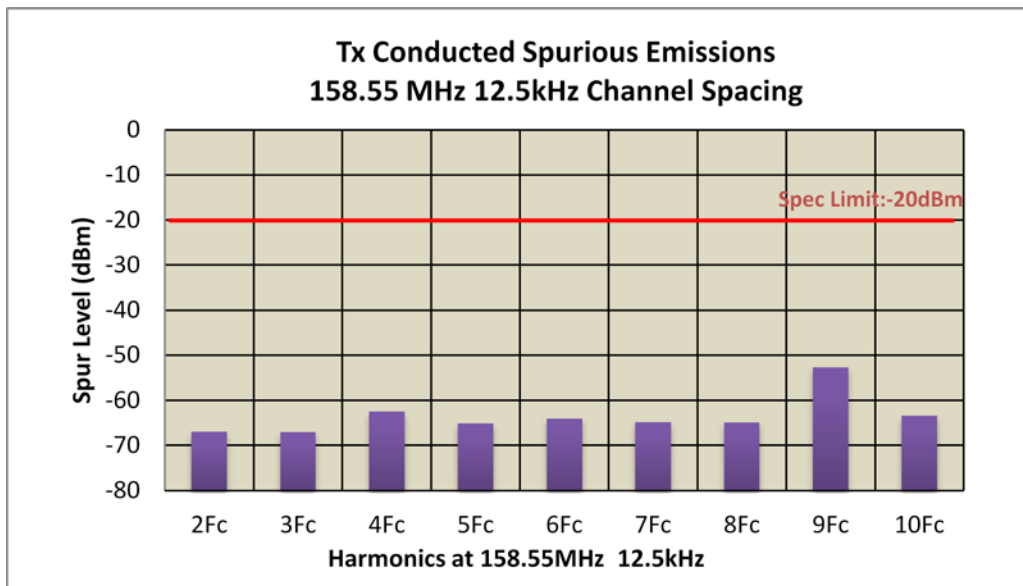
Figure 6F-11: 1W Harmonic of Carrier 158.55 MHz, Digital 12.5 kHz Channel Spacing
