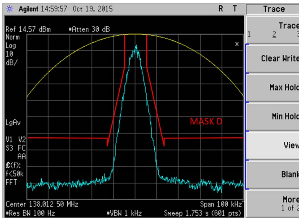
Figure 6E-2: 138.0125 MHz, O.153 Test Pattern 4FSK Voice and Data Modulation, 7K60F1W Mask D (Not for FCC Review)
