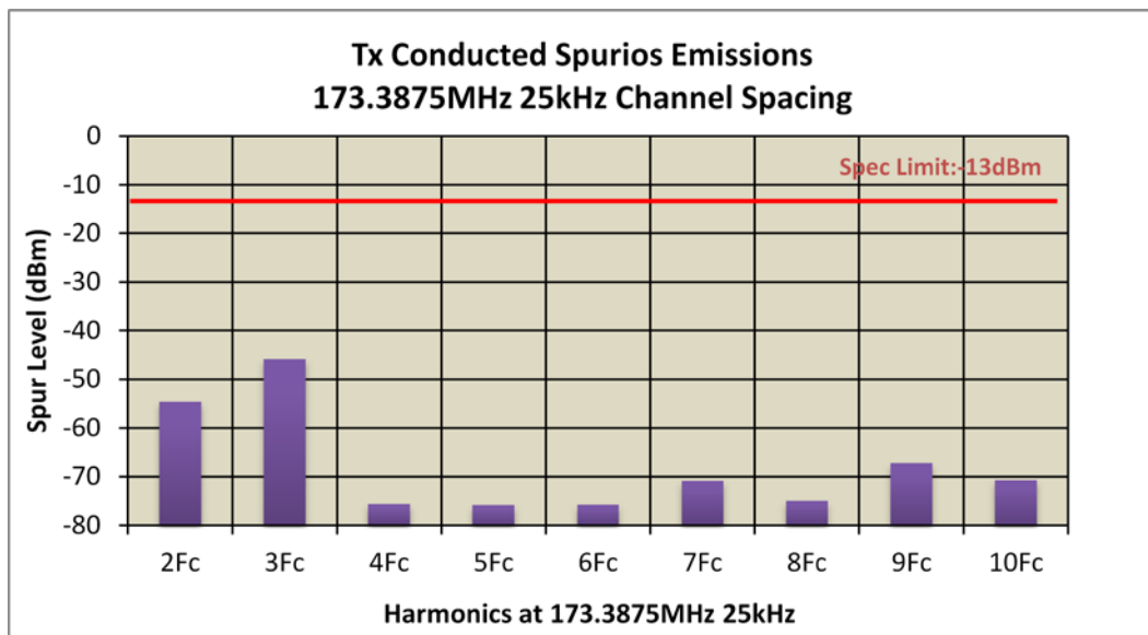
Figure 6F-4: 30 W Harmonic of Carrier 173.3875 MHz, 25 kHz Channel Spacing (Not for FCC Review)
