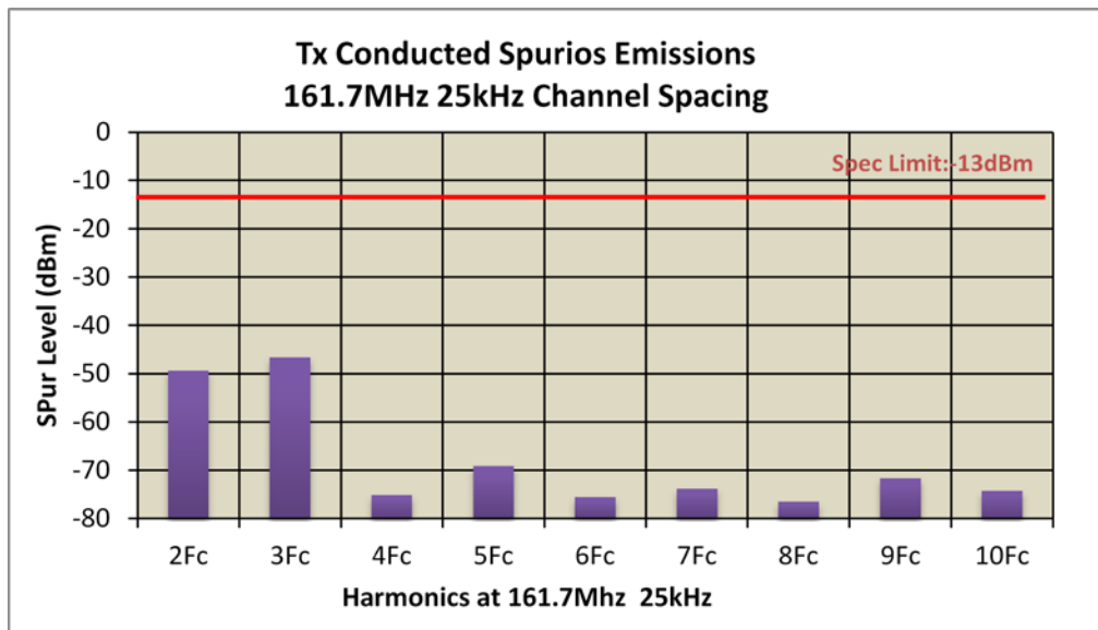
Figure 6F-3: 30 W Harmonic of Carrier 161.7 MHz, 25 kHz Channel Spacing (Part 74)
