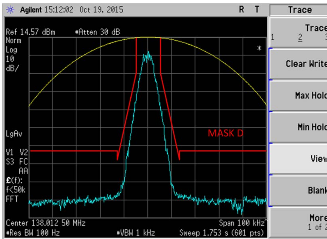
Figure 6E-4: 138.0125 MHz, O.153 Test Pattern 4FSK Voice Modulation only, 7K60F1E Mask D (Not for FCC Review)
