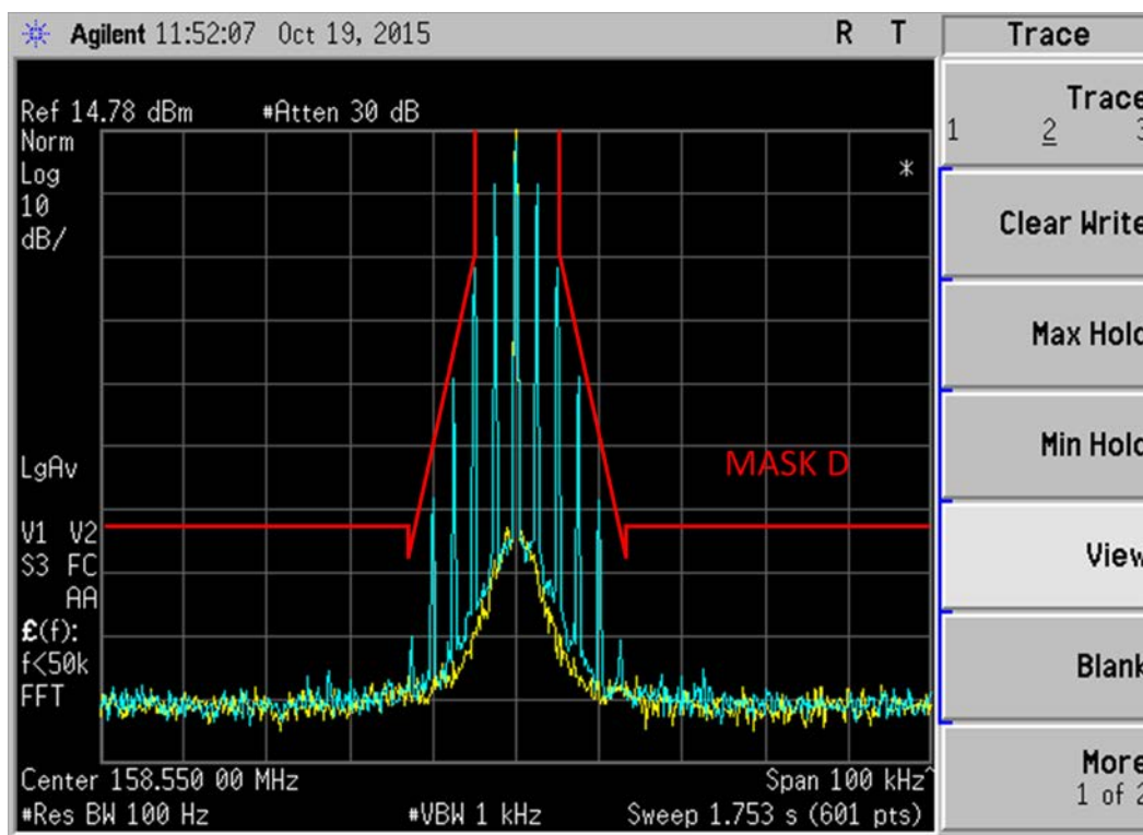
Figure 6E-5: 158.55 MHz, 12.5 kHz Channel Spacing, 2500Hz Audio Modulation only, 11K0F3E Mask D
