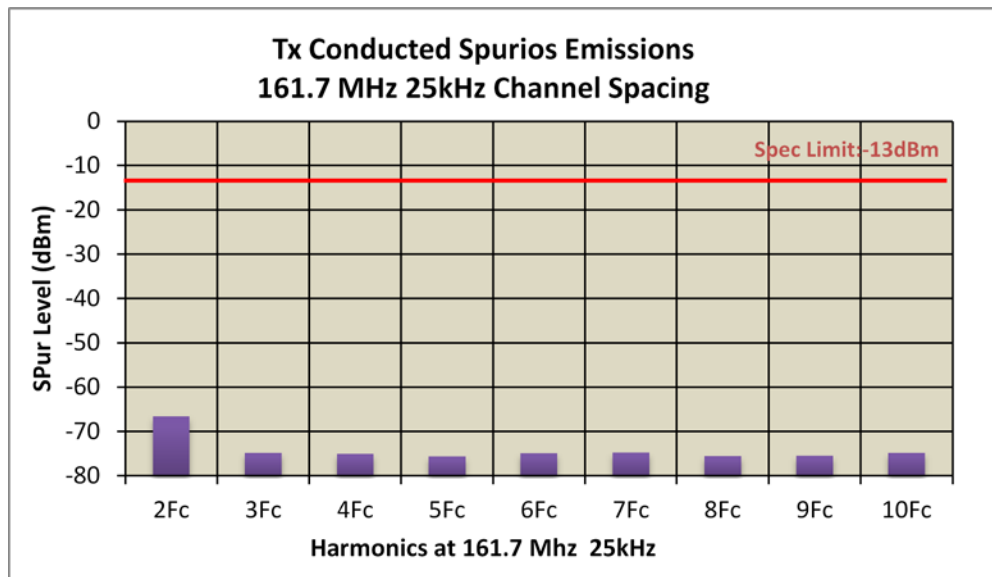
Figure 6F-6: 1W Harmonic of Carrier 161.7 MHz, 25 kHz Channel Spacing (Part 74)
