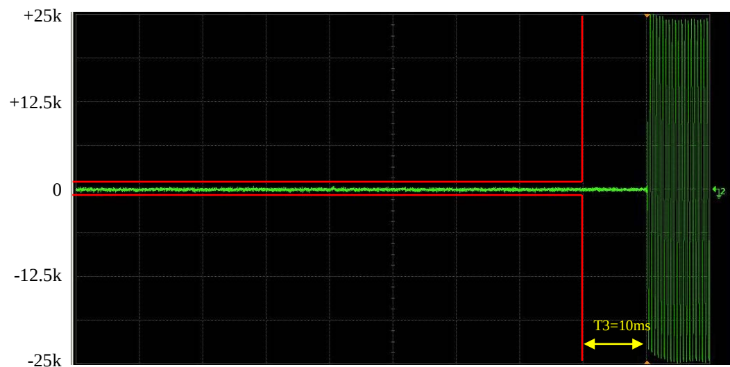
6I-4 – 158.55 MHz, 25 kHz Channel Spacing De-Key Decay Time (Part 22, 80)
