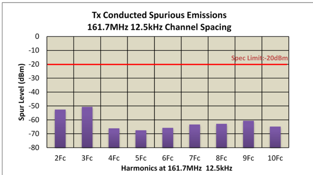
Figure 6F-9: 30 W Harmonic of Carrier 161.7 MHz, Digital 12.5 kHz Channel Spacing
