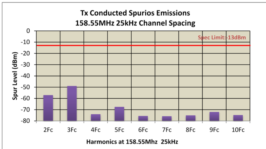
Figure 6F-2: 30 W Harmonic of Carrier 158.55 MHz, 25 kHz Channel Spacing (Part 22, 80)
