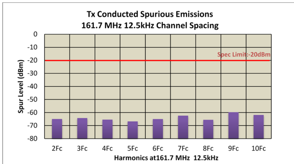
Figure 6F-12: 1W Harmonic of Carrier 161.7 MHz, Digital 12.5 kHz Channel Spacing
