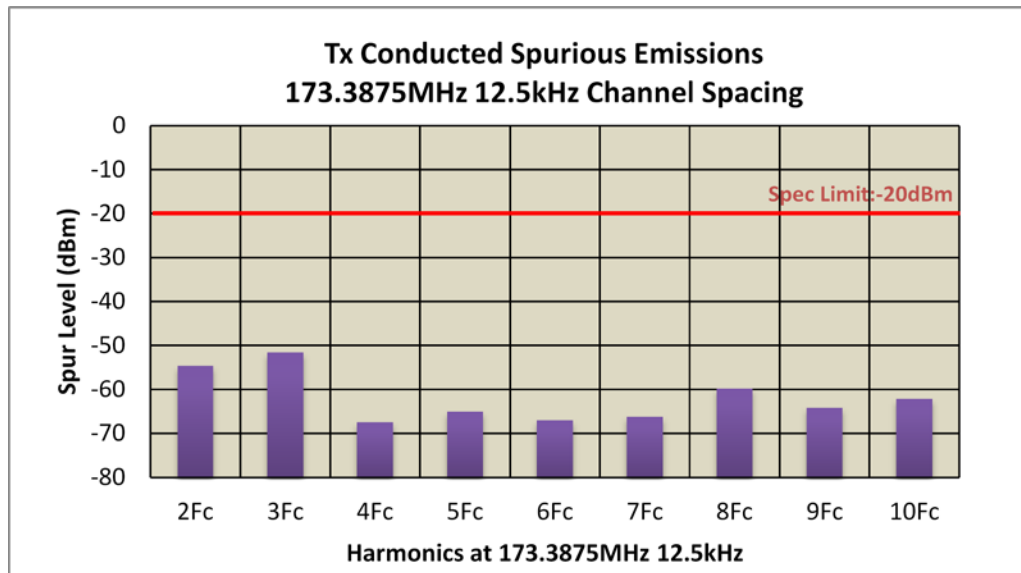
Figure 6F-10: 30 W Harmonic of Carrier 173.3875 MHz, Digital 12.5 kHz Channel Spacing
