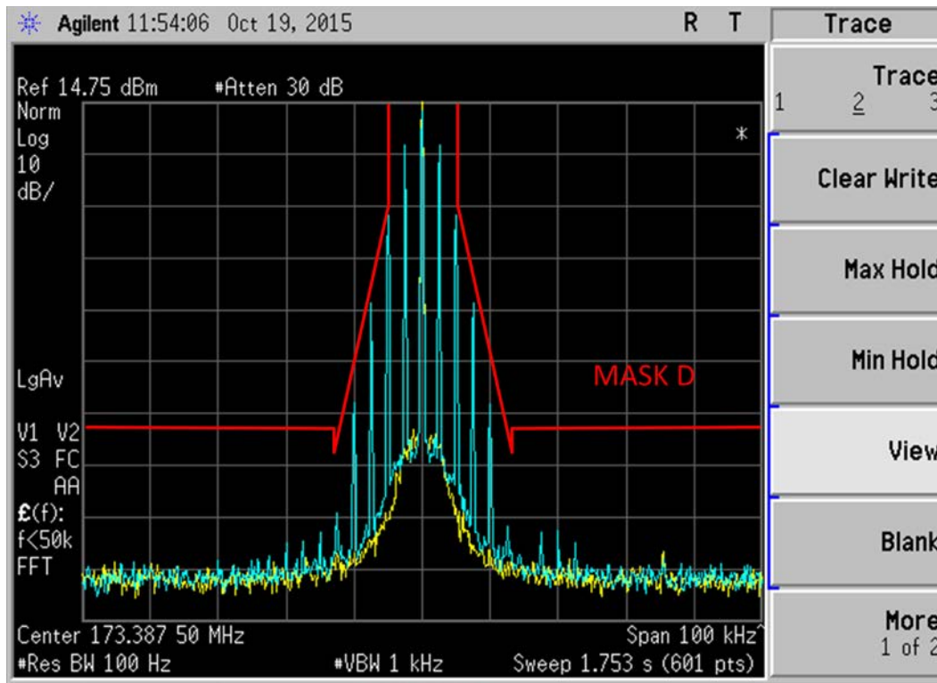
Figure 6E-9: 173.3875MHz, 12.5 kHz Channel Spacing, 2500Hz Audio Modulation only, 11K0F3E Mask D
