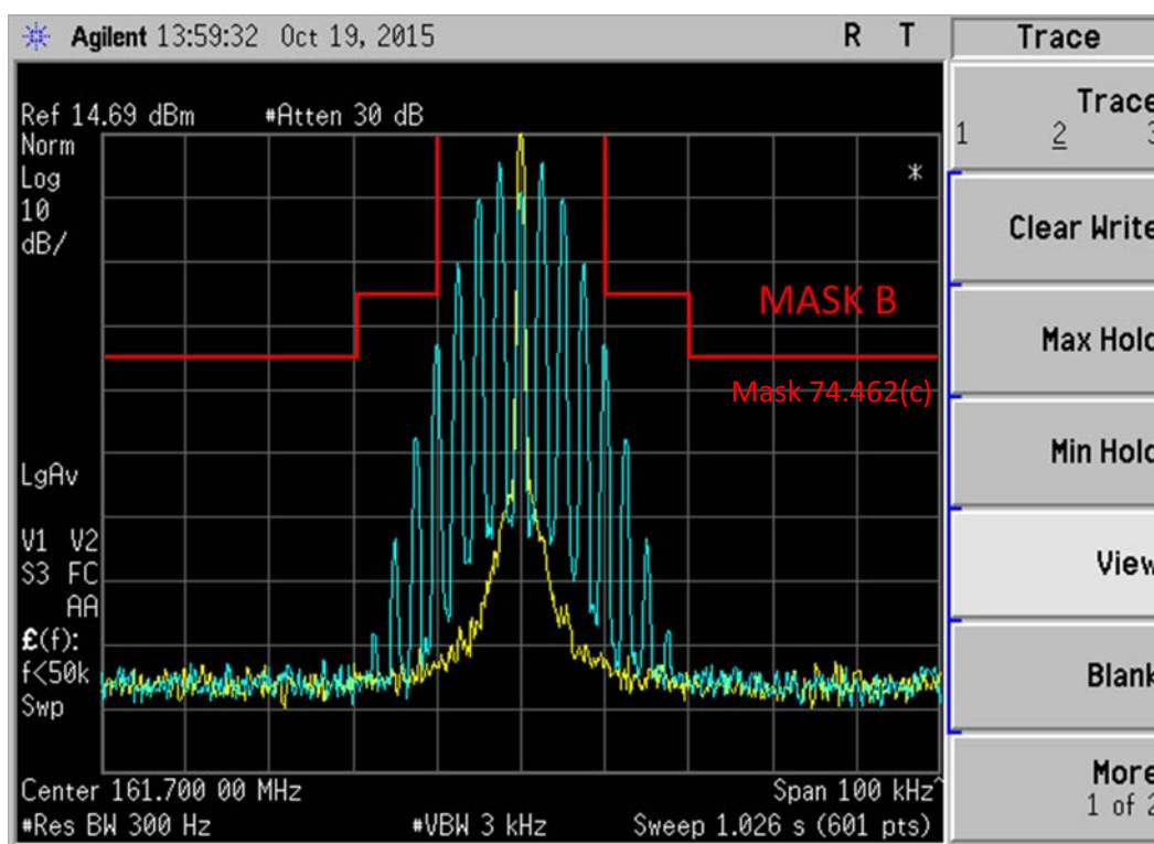
Figure 6E-15: 161.7 MHz, 25 kHz Channel Spacing, 2500Hz Audio Modulation only, 16K0F3E Mask B, Mask 74.462 (c) (Part 74)
