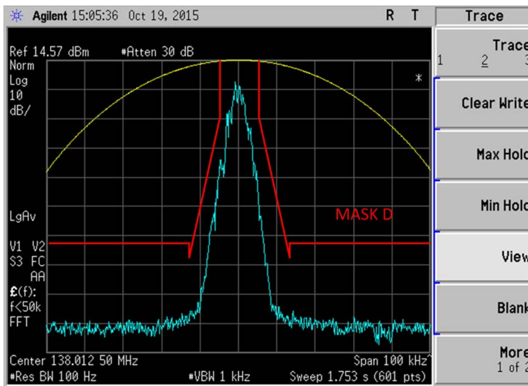
Figure 6E-3: 138.0125 MHz, O.153 Test Pattern 4FSK Data Modulation only, 7K60F1D Mask D (Not for FCC Review)
