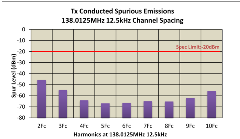
Figure 6F-7: 30 W Harmonic of Carrier 138.0125 MHz, Digital 12.5 kHz Channel Spacing (Not for FCC Review)
