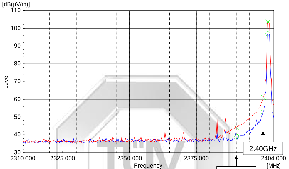
Plot 33 – Lower Band Edge at 2.4000GHz
