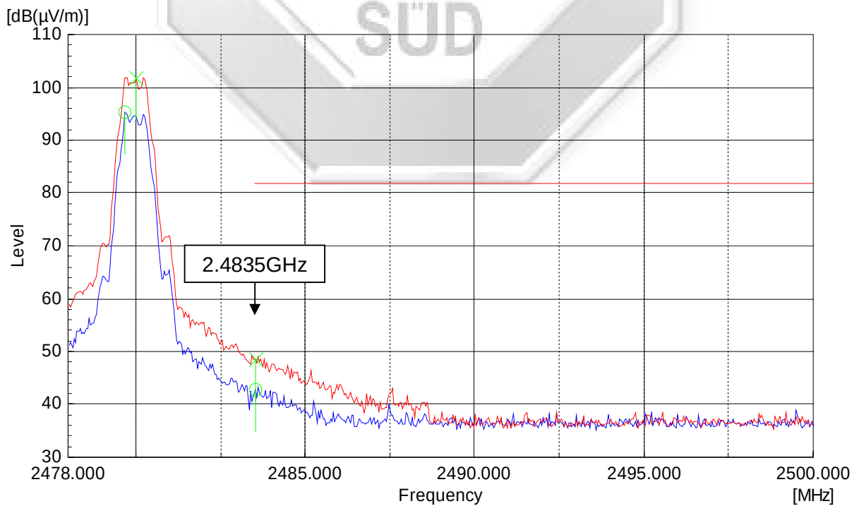
Plot 34 – Upper Band Edge at 2.4835GHz
