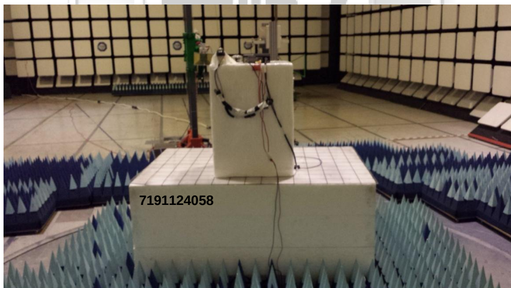
Radiated Emissions Test Setup (Rear View)
