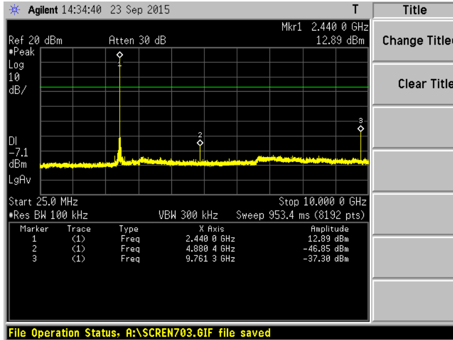
Plot 9 – Channel 19
