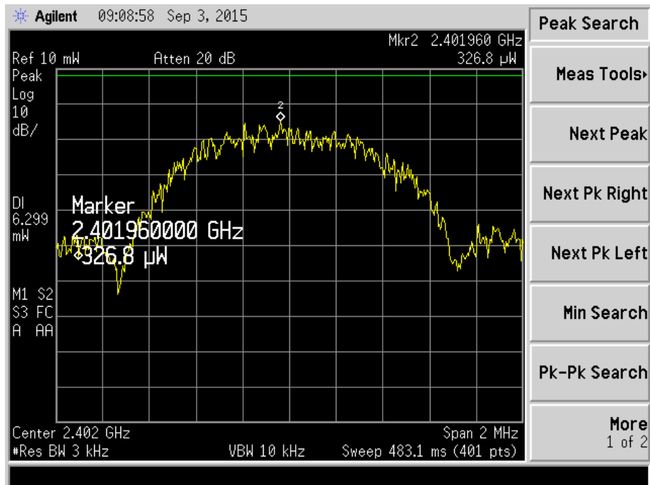
Plot 39 – Channel 0
