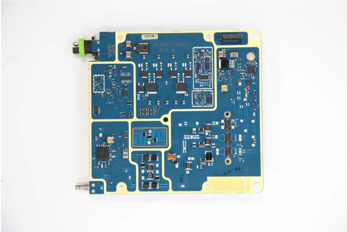
Exhibit 9A: Transmitter Board (Top)
