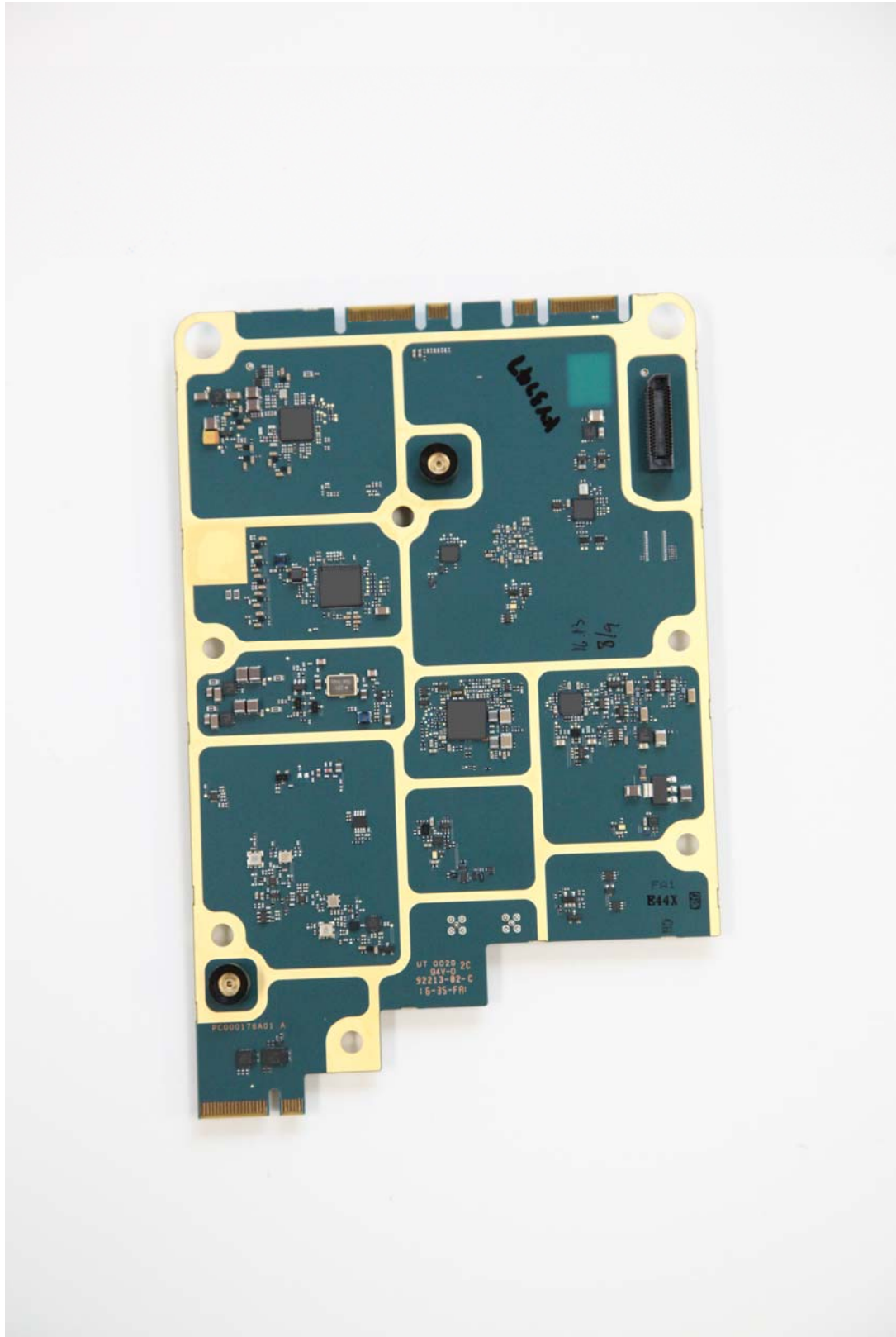
Exhibit 9D: Transceiver Board (Bottom)
