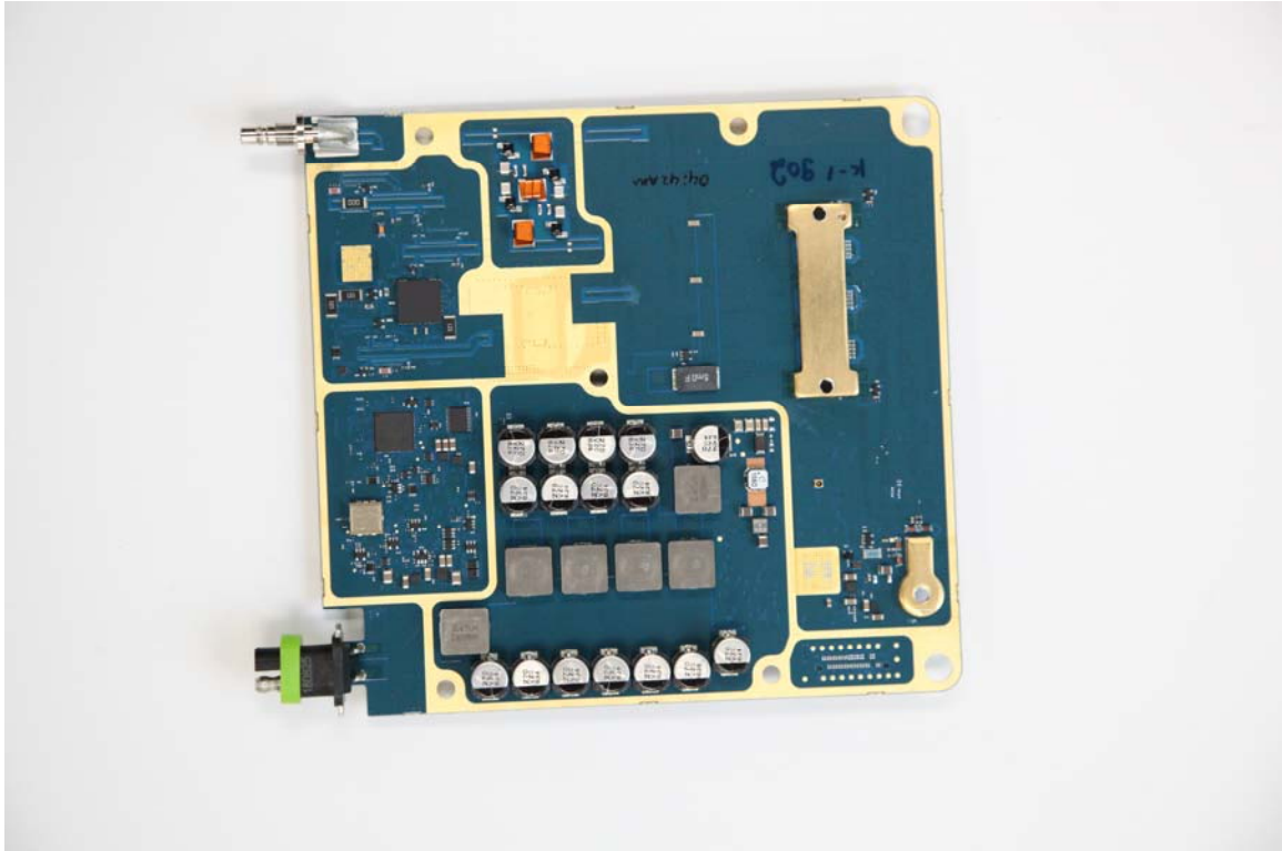
Exhibit 9B: Transmitter Board (Bottom)
