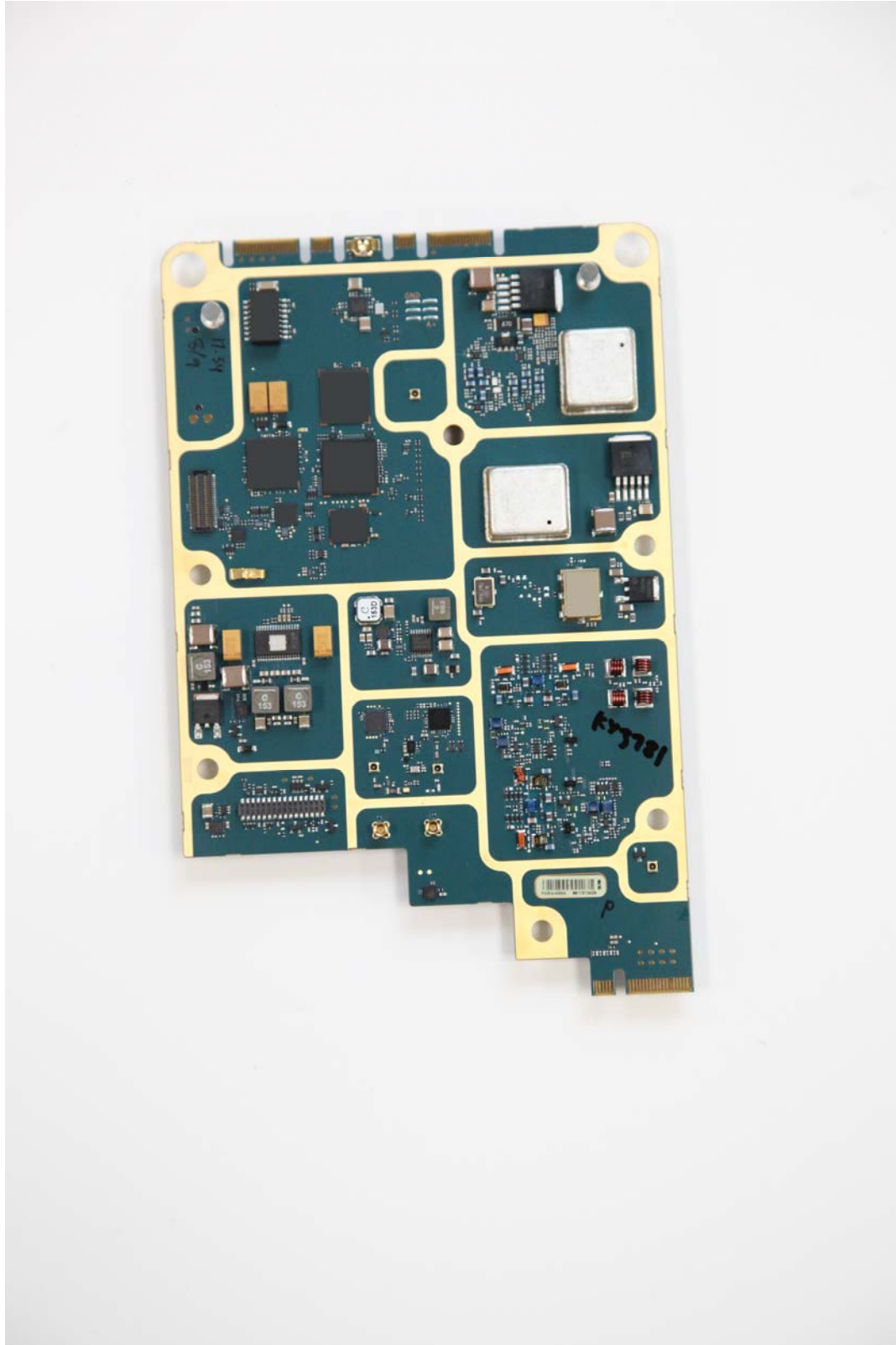
Exhibit 9C: Transceiver Board with Shields (Top)
