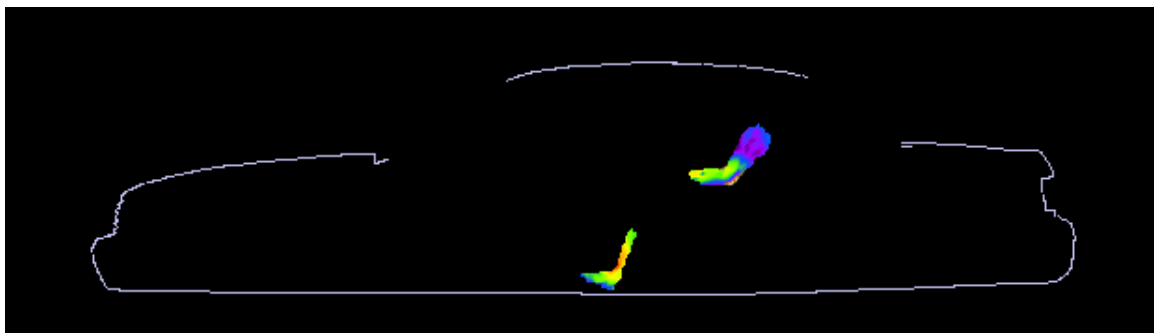
Figure 5. SAR distribution at 173.0125 MHz in the passenger model located on the side of the back seat, produced by the trunk-mount HAD4022A antenna. The contour plot is relative to the plane where the peak 1-g average SAR for this exposure condition occurs.
