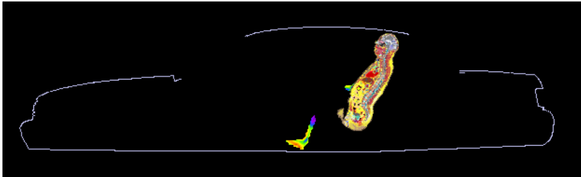
Figure 8. SAR distribution at 450.0125 MHz in the passenger model located on the center of the back seat, produced by the trunk-mount HAE6013A antenna. The contour plot is relative to the plane where the peak 1-g average SAR for this exposure condition occurs.
