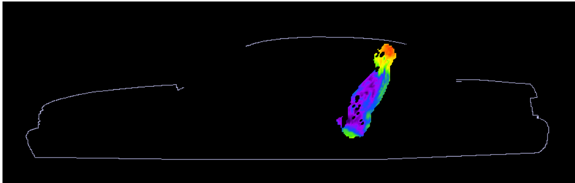
Figure 7. SAR distribution at 406.5 MHz in the passenger model located on the side of the back seat, produced by the trunk-mount HAE6013A antenna. The contour plot is relative to the plane where the peak 1-g average SAR for this exposure condition occurs.
