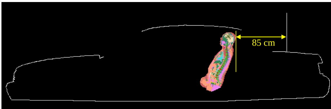
Figure 4: Passenger model exposed to a trunk-mount antenna: XFDTD geometry.
