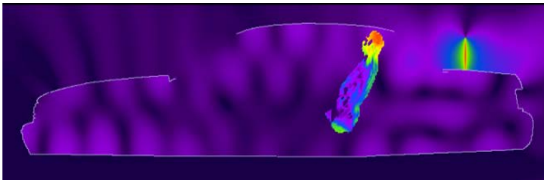
Figure 8. (a) E-field magnitude distribution corresponding to exposure condition of Figure 7, and (b) H-field magnitude distribution corresponding to exposure condition of Figure 7.
