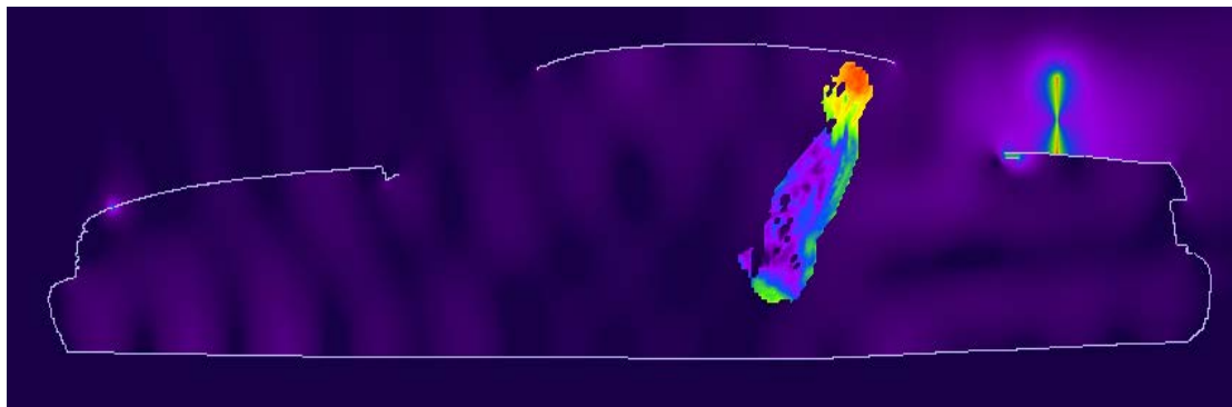
Figure 7. SAR distribution at 406.5 MHz in the passenger model located on the side of the back seat, produced by the trunk-mount HAE6013A antenna. The contour plot is relative to the plane where the peak 1-g average SAR for this exposure condition occurs.
