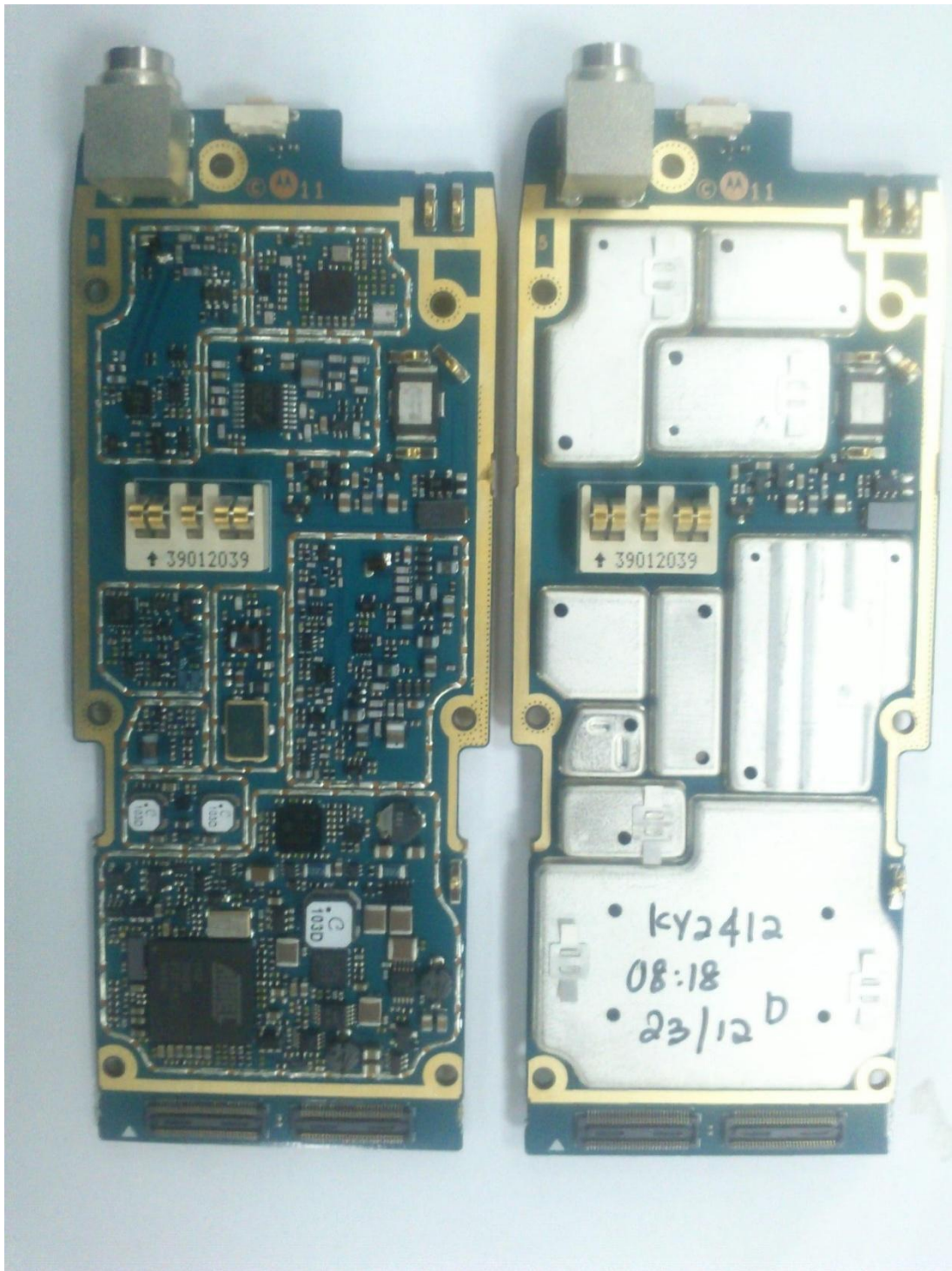
APX4000 VHF Board Without and With Shields (Bottom)
