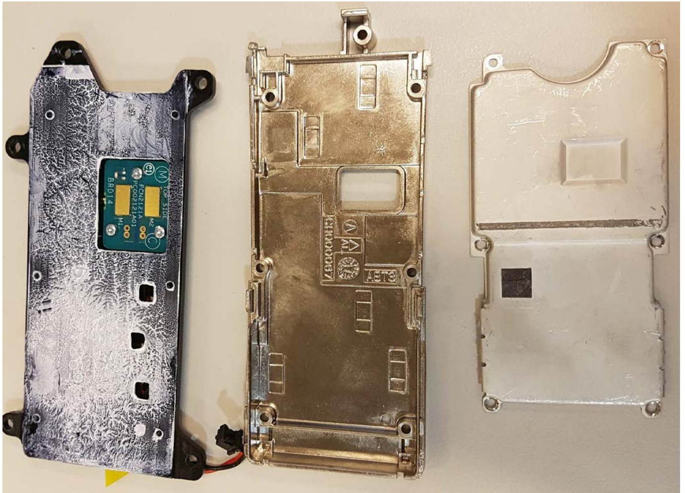
MC-EDGE APX4000 VHF Heatsink assembly view
