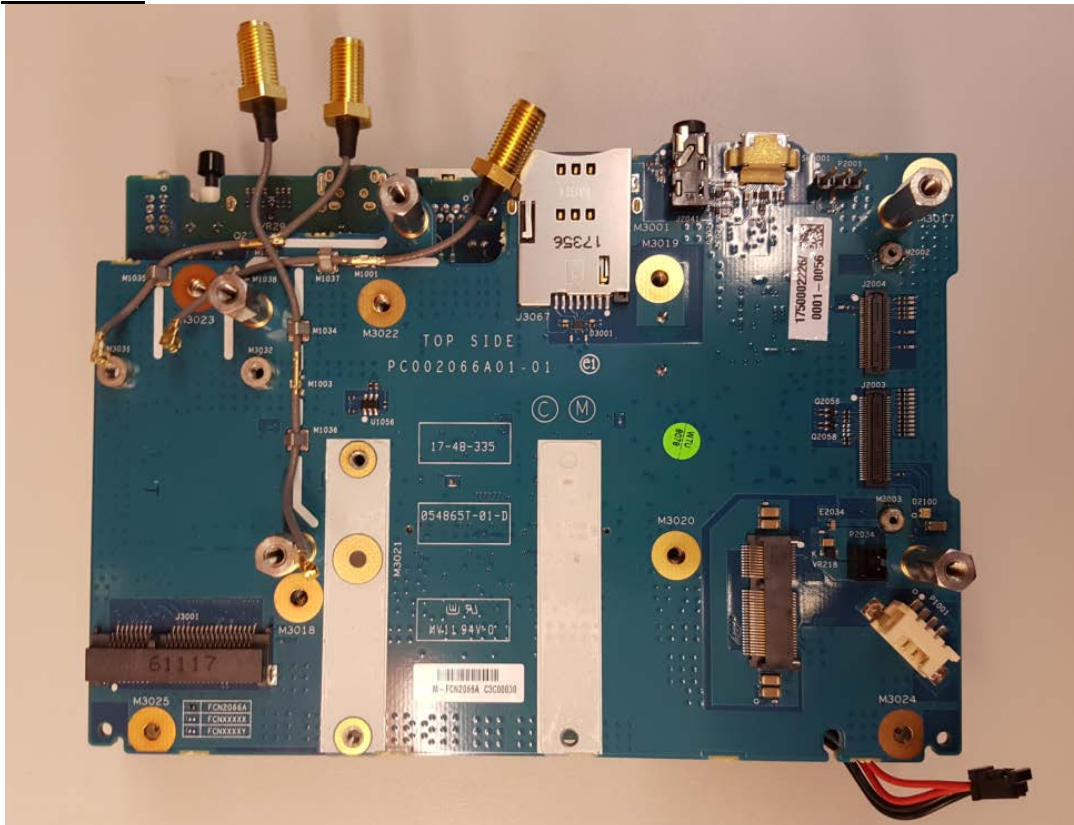
MC-EDGE Piggy Board Top View Without Front Panel (APX4000 VHF Removed)
