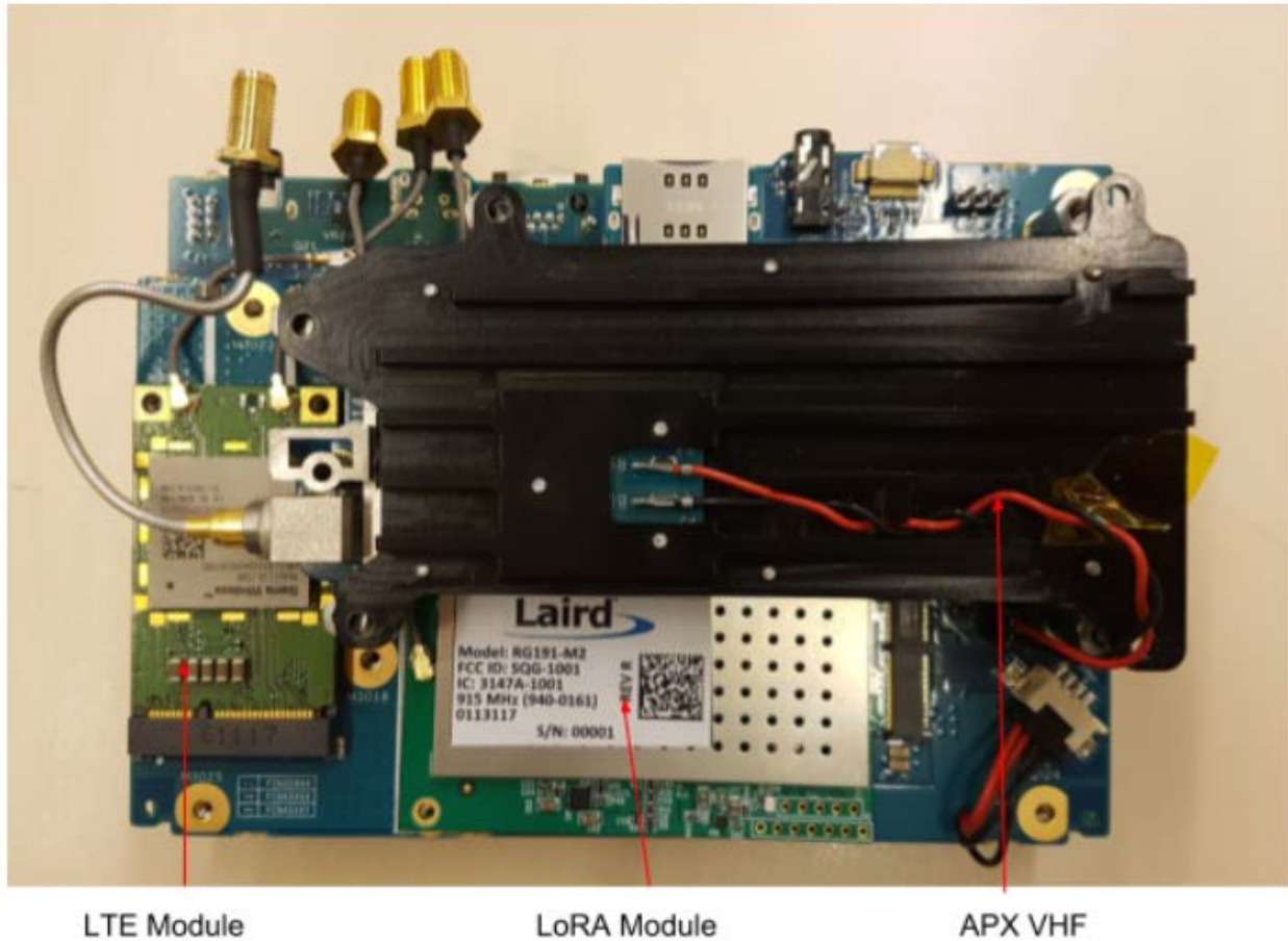
MC-EDGE Piggy Board Top View (APX4000 VHF Installed, with LORA and LTE) without Front Panel
