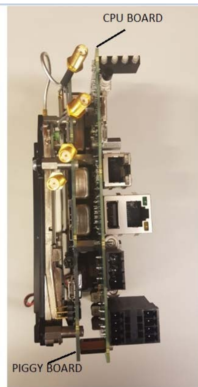
INTERNAL CPU & PIGGY BOARD (APX4000 VHF INSTALLED WITH LORA & LTE)
