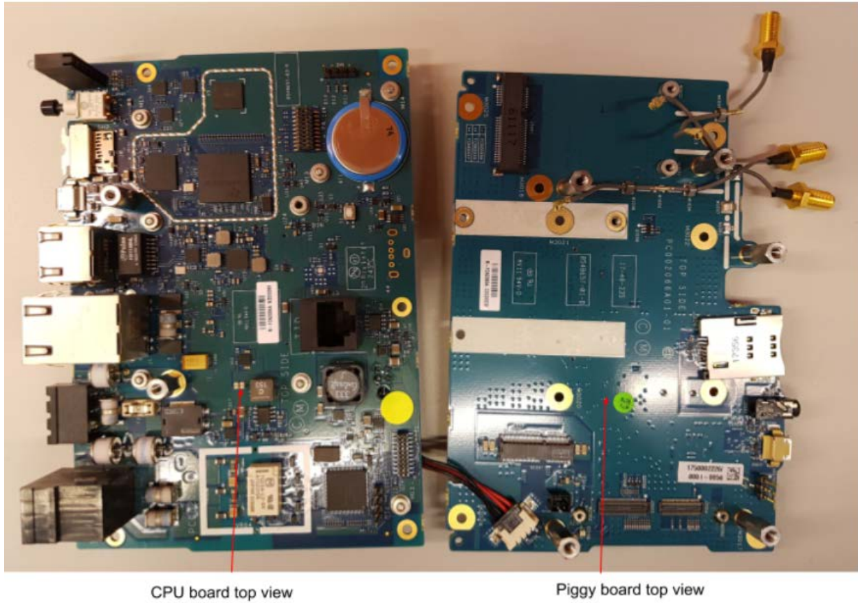
CPU Board Top View and Piggy Board Top View
