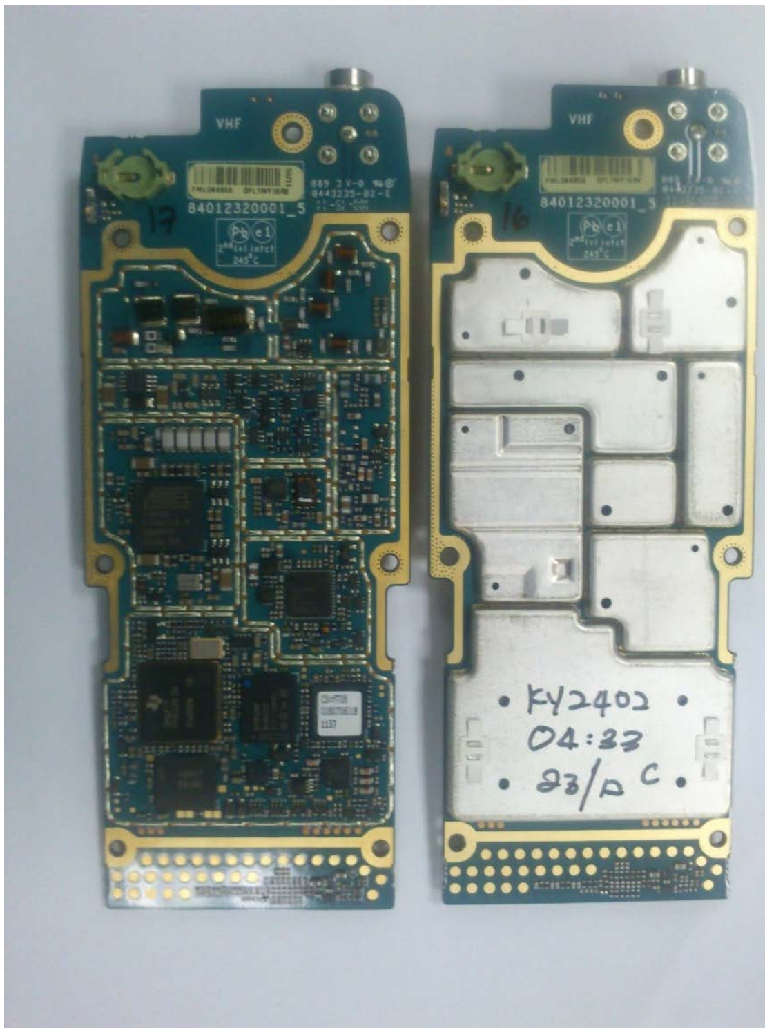
APX4000 VHF Board Without and With Shields (Top)
