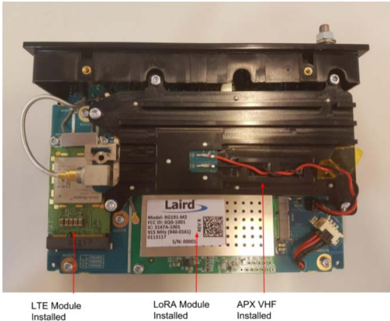
MC-EDGE Piggy Board Top View With Front Panel (APX4000 VHF Installed, with LORA and LTE)
