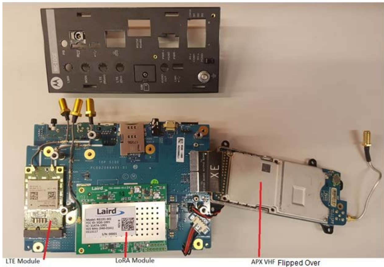
MC-EDGE Piggy Board Top View (APX4000 VHF Flipped over, with LORA and LTE) Without Front Panel
