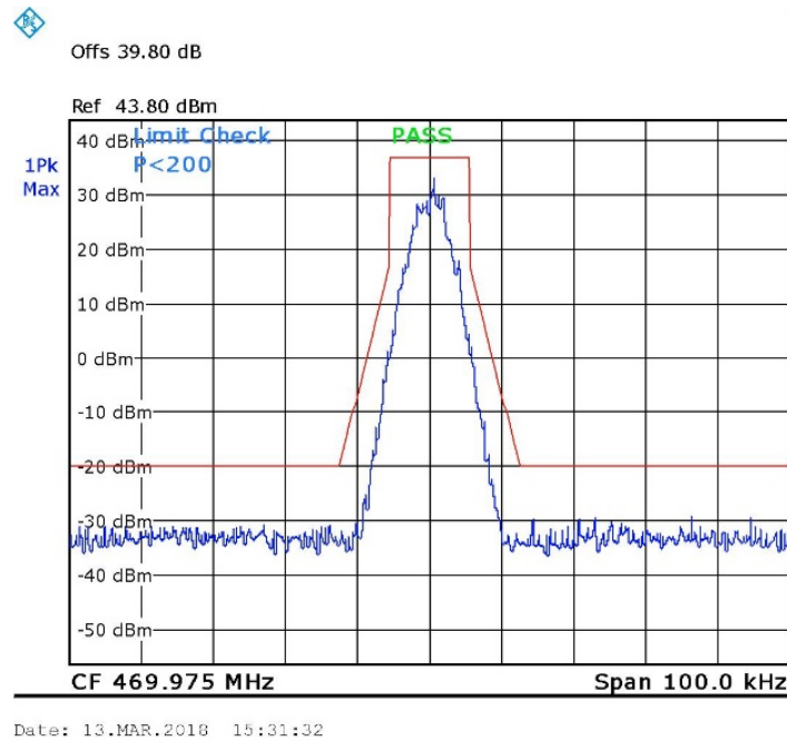
Figure 21. 469.975MHz, TDMA
