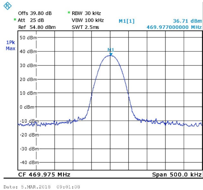
Figure 14. 469.975MHz, TDMA
