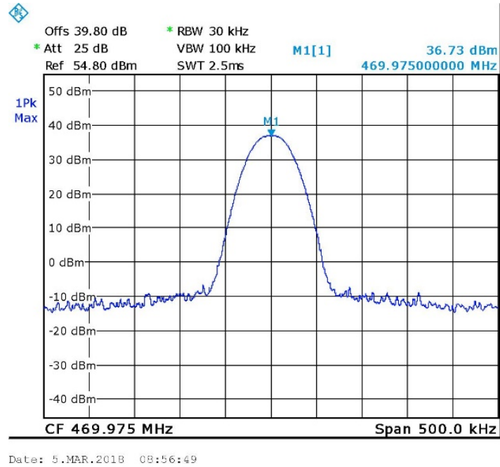
Figure 11. 469.975MHz, Digital
