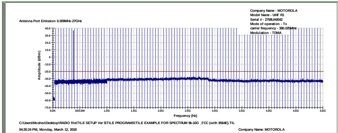
Figure 28 Spurious Emissions at Antenna Terminals 380.025MHz, TDMA
