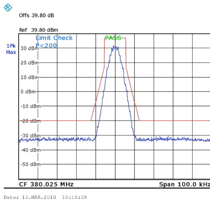
Figure 16. 380.025MHz, Digital
