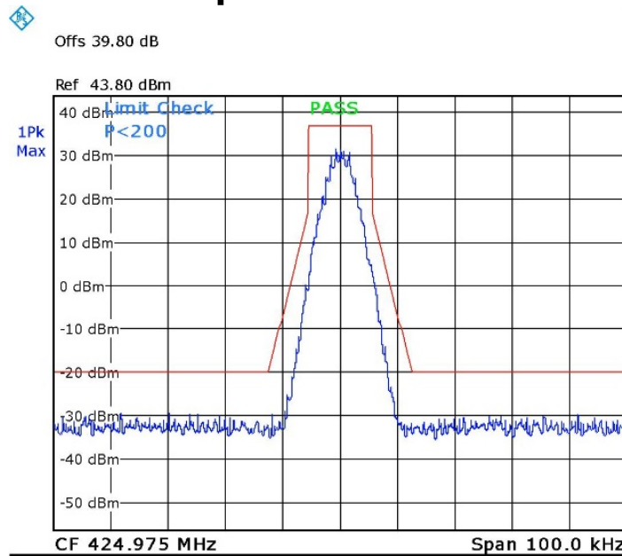
Figure 17. 424.975MHz, Digital
