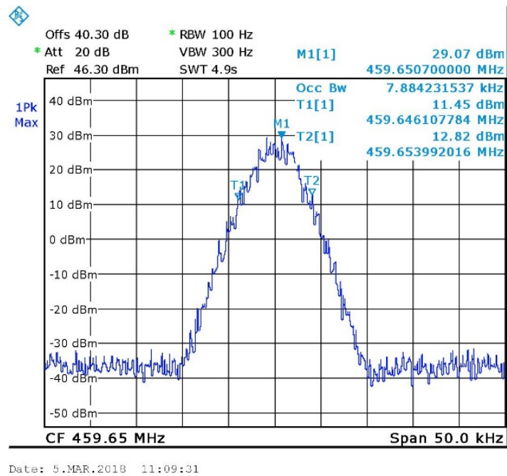
Figure 23. 99% Occupied BW, TDMA
