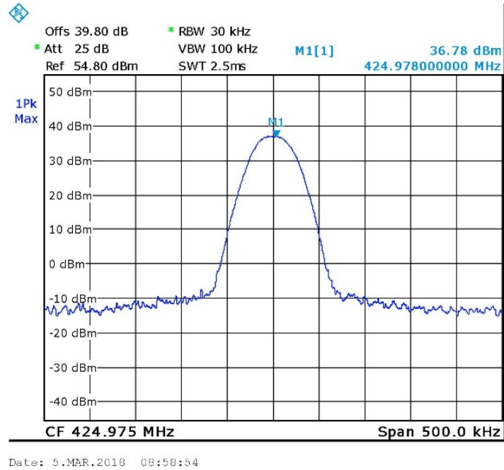
Figure 13. 424.975MHz, TDMA
