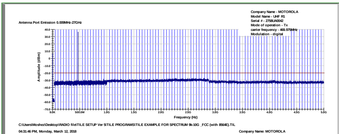
Figure 27 Spurious Emissions at Antenna Terminals 469.975MHz, Digital
