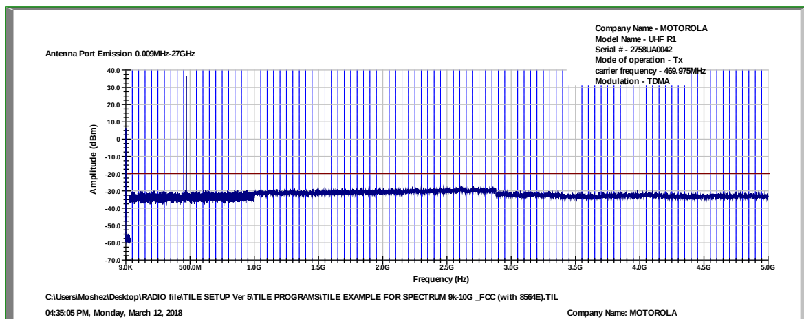
Figure 30 Spurious Emissions at Antenna Terminals 469.975MHz, TDMA
