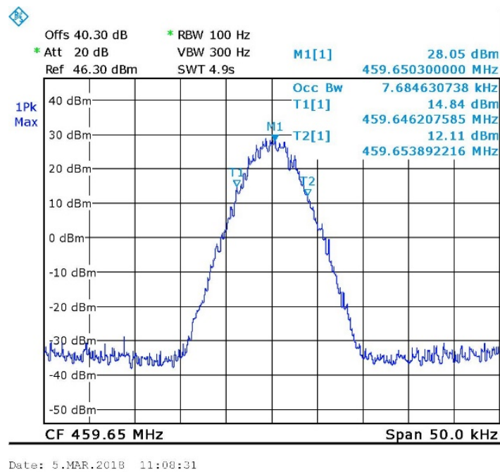
Figure 22. 99% Occupied BW, digital
