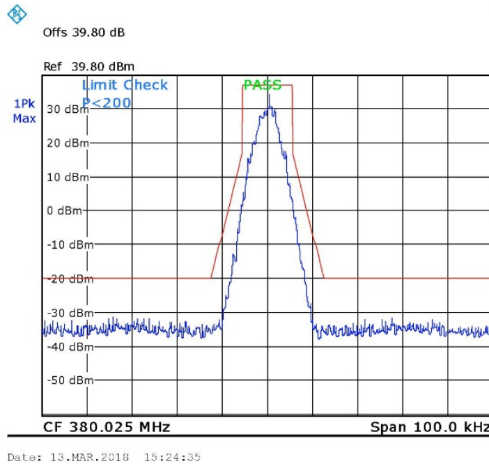
Figure 19. 380.025MHz, TDMA
