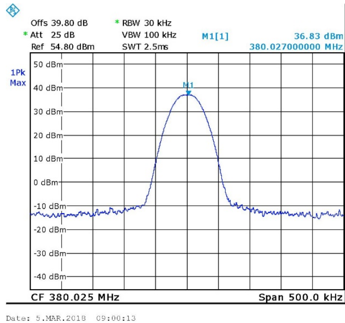
Figure 12. 380.025MHz, TDMA
