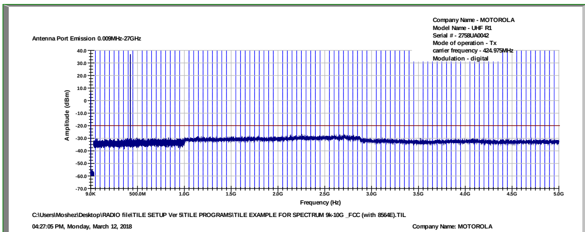
Figure 26 Spurious Emissions at Antenna Terminals 424.975MHz, Digital
