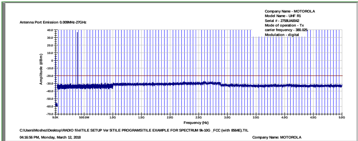
Figure 25 Spurious Emissions at Antenna Terminals 380.025MHz, Digital
