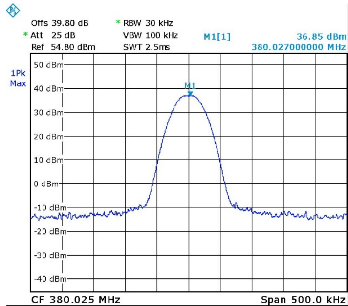
Figure 9. 380.025MHz, Digital
