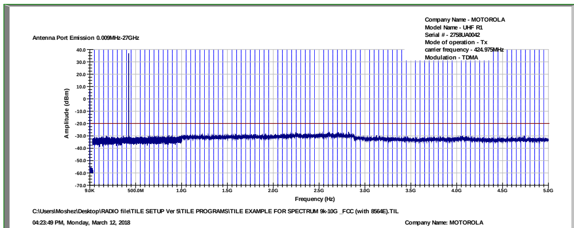
Figure 29 Spurious Emissions at Antenna Terminals 424.975MHz, TDMA
