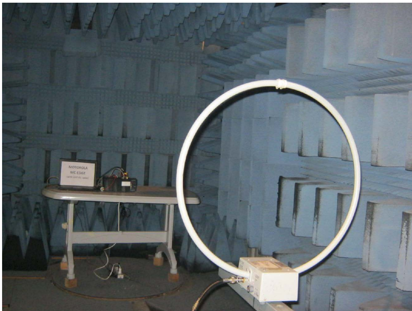
Figure 7 – 1 Radiated Emission Test 0.009-30MHz
