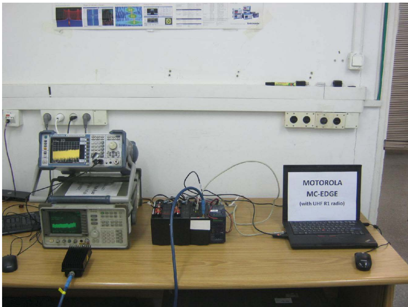
Figure 7 - 5 Conducted Emission Terminal Port Test
