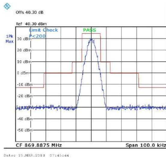
Figure 32. 869.8875MHz, Digital
