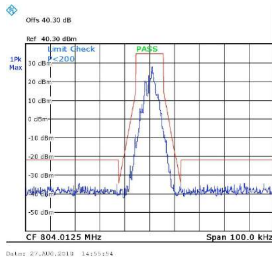
Figure 43. 804.0125MHz, Digital
