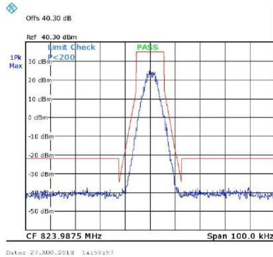
Figure 51. 823.9875MHz, TDMA
