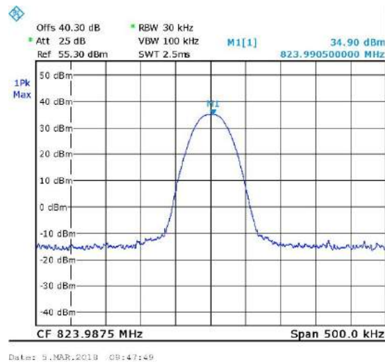
Figure 14. 823.9875MHz, Digital
