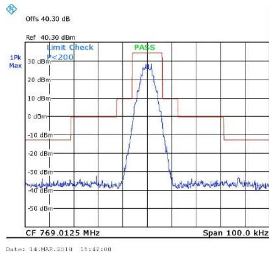
Figure 26. 769.0125MHz, Digital
