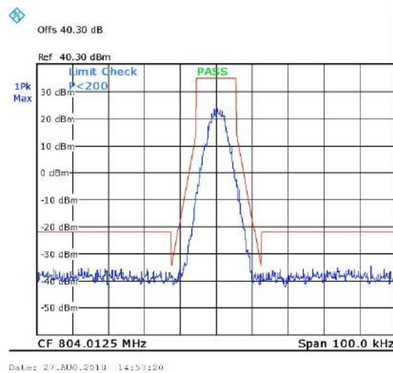
Figure 50. 804.0125MHz, TDMA
