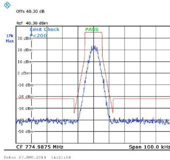
Figure 48. 774.9875MHz, TDMA
