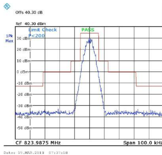
Figure 30. 823.9875MHz, Digital
