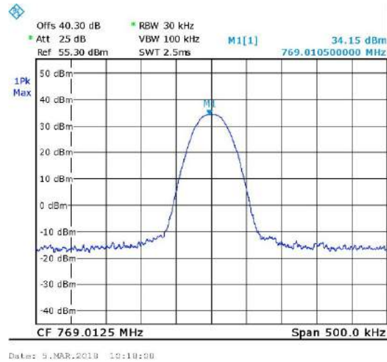
Figure 18. 769.0125MHz, TDMA
