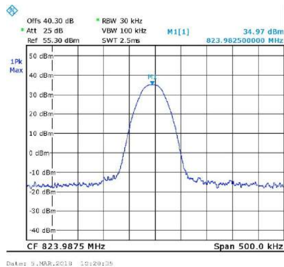
Figure 22. 823.9875MHz, TDMA
