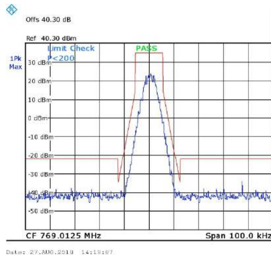
Figure 47. 769.0125MHz, TDMA
