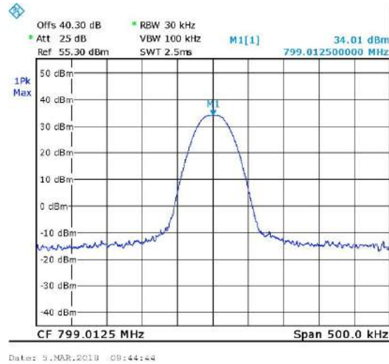
Figure 12. 799.0125MHz, Digital
