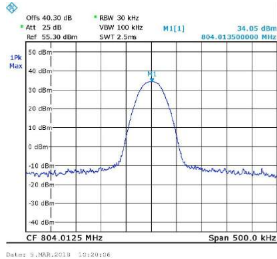
Figure 21. 804.0125MHz, TDMA
