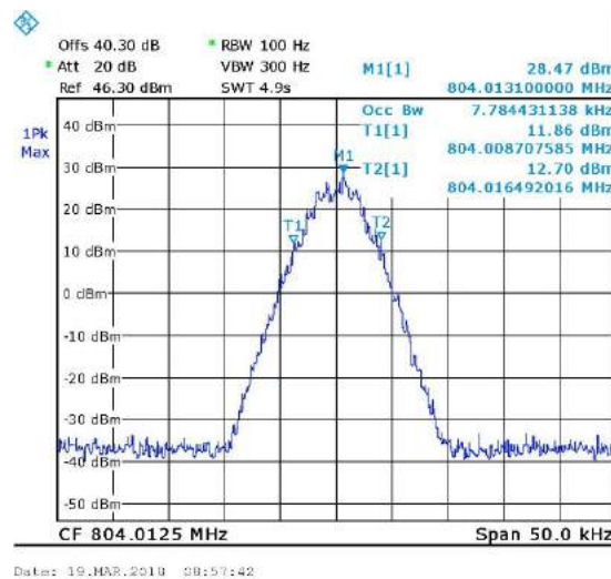
Figure 55. 99% Occupied BW, TDMA
