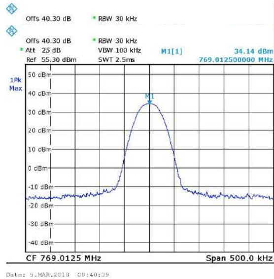
Figure 10. 769.0125MHz, Digital
