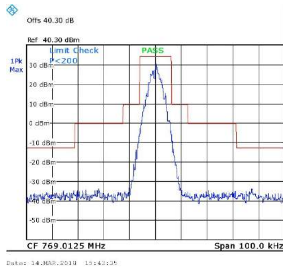
Figure 33. 769.0125MHz, TDMA
