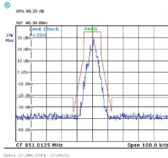
Figure 45. 851.0125MHz, Digital
