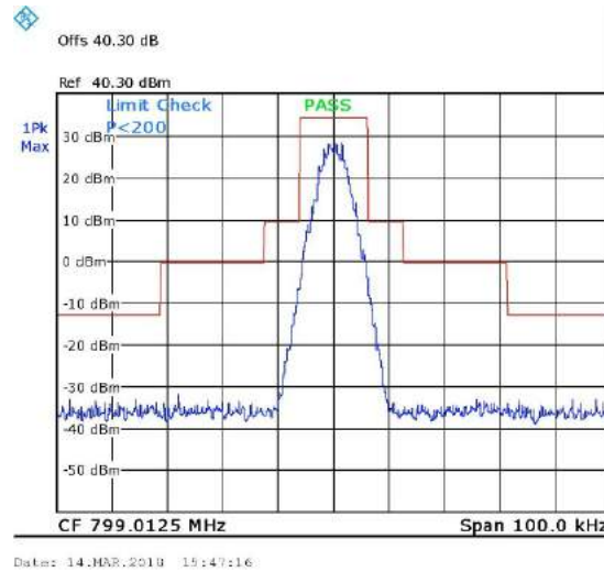
Figure 28. 799.0125MHz, Digital
