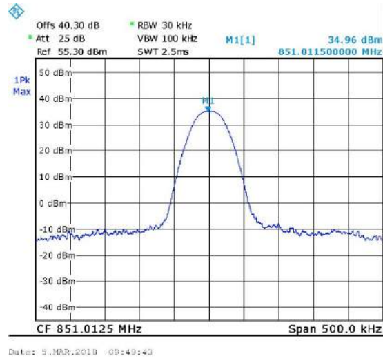
Figure 15. 851.0125MHz, Digital
