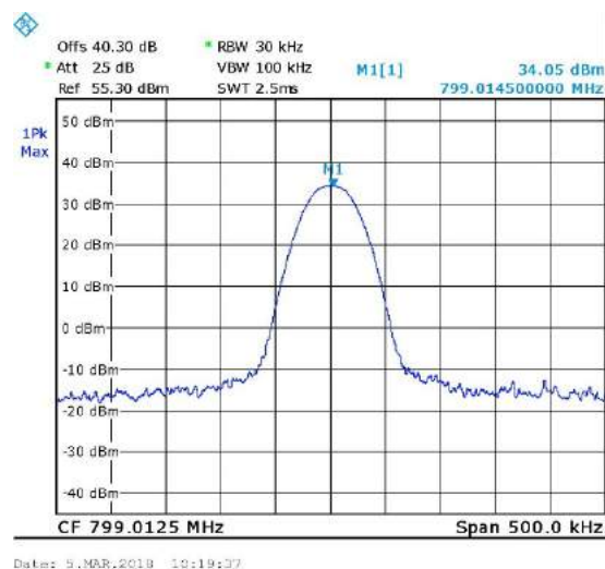
Figure 20. 799.0125MHz, TDMA
