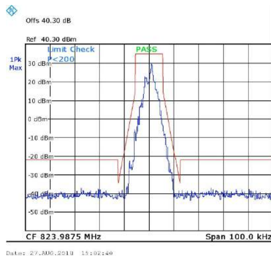
Figure 44. 823.9875MHz, Digital
