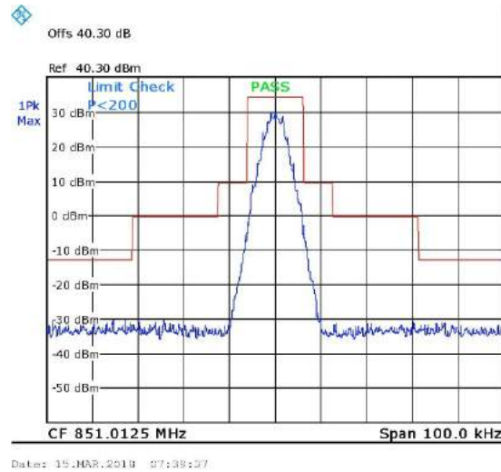
Figure 31. 851.0125MHz, Digital
