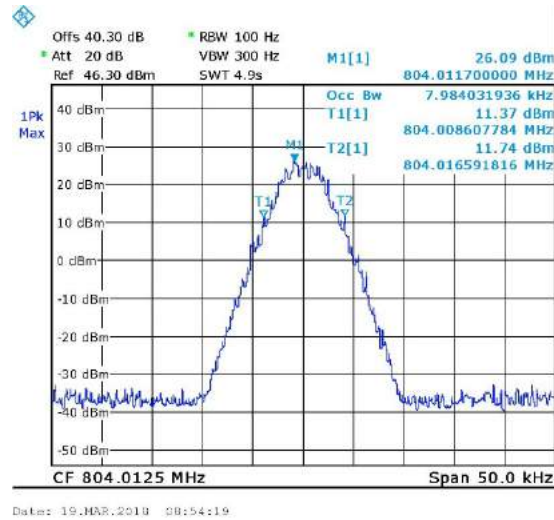
Figure 54. 99% Occupied BW, digital
