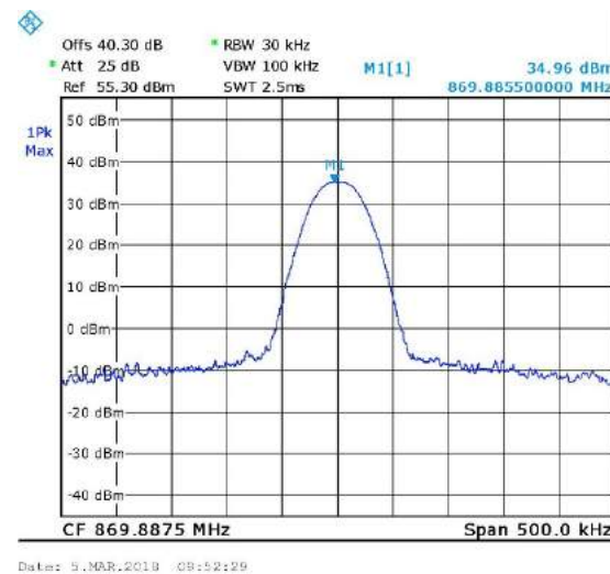
Figure 16. 869.8875MHz, Digital
