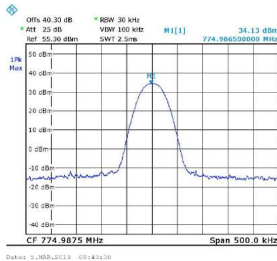
Figure 11. 774.9875MHz, Digital
