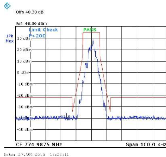
Figure 41. 774.9875MHz, Digital
