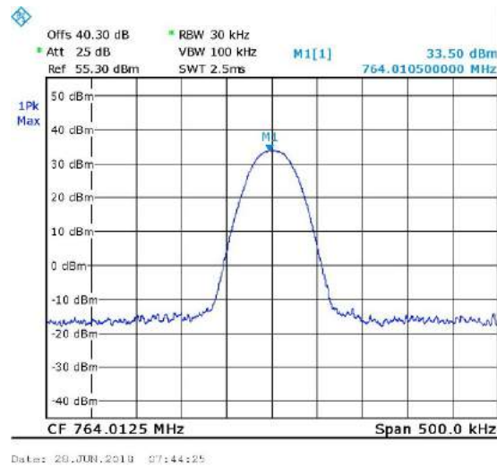
Figure 17. 764.0125MHz, TDMA
