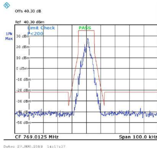
Figure 40. 769.0125MHz, Digital
