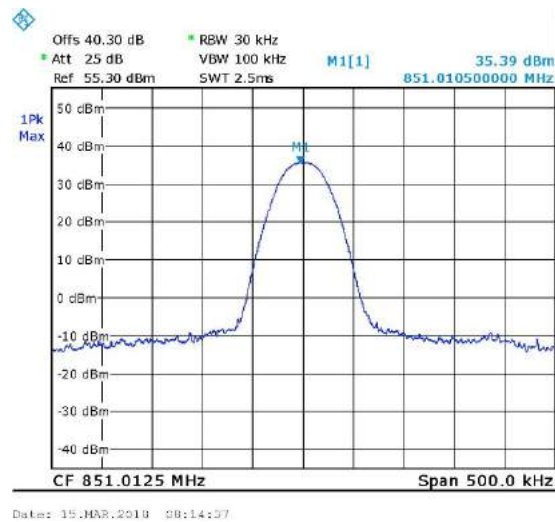
Figure 23. 851.0125MHz, TDMA
