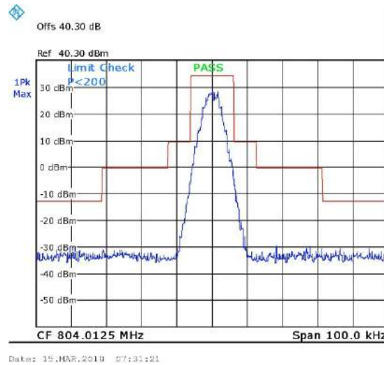
Figure 29. 804.0125MHz, Digital
