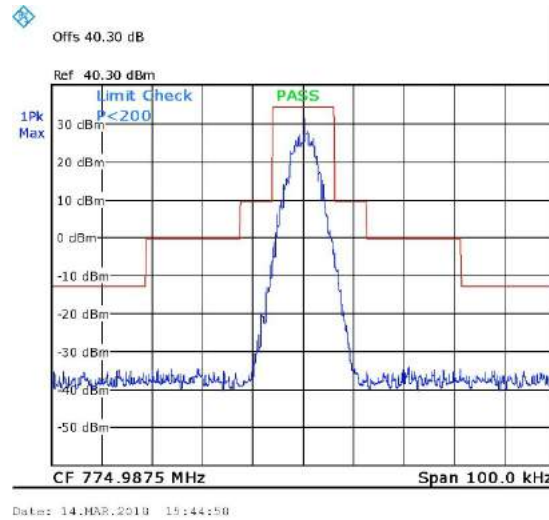
Figure 34. 774.9875MHz, TDMA
