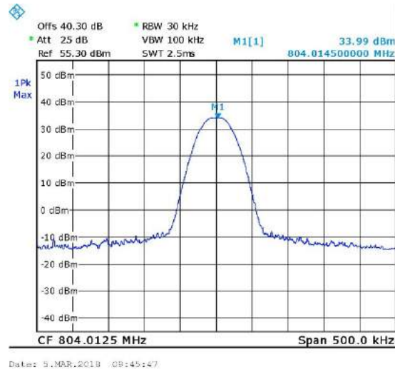
Figure 13. 804.0125MHz, Digital
