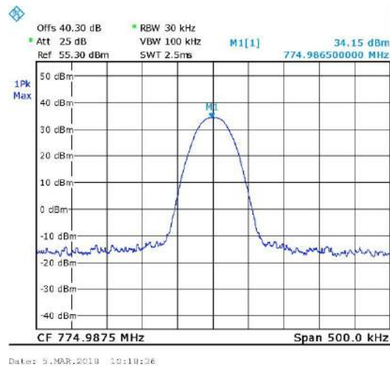
Figure 19. 774.9875MHz, TDMA
