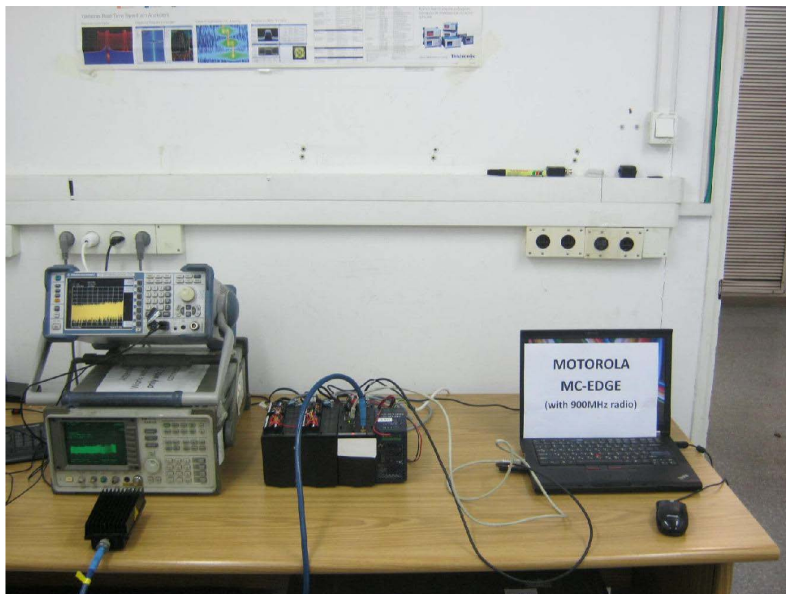
Figure 7 - 5 Conducted Emission Terminal Port Test
