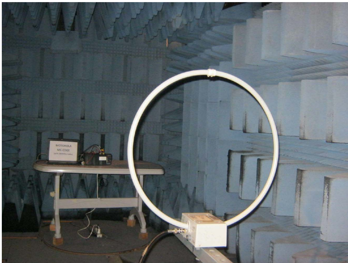
Figure 7 – 1 Radiated Emission Test 0.009-30MHz
