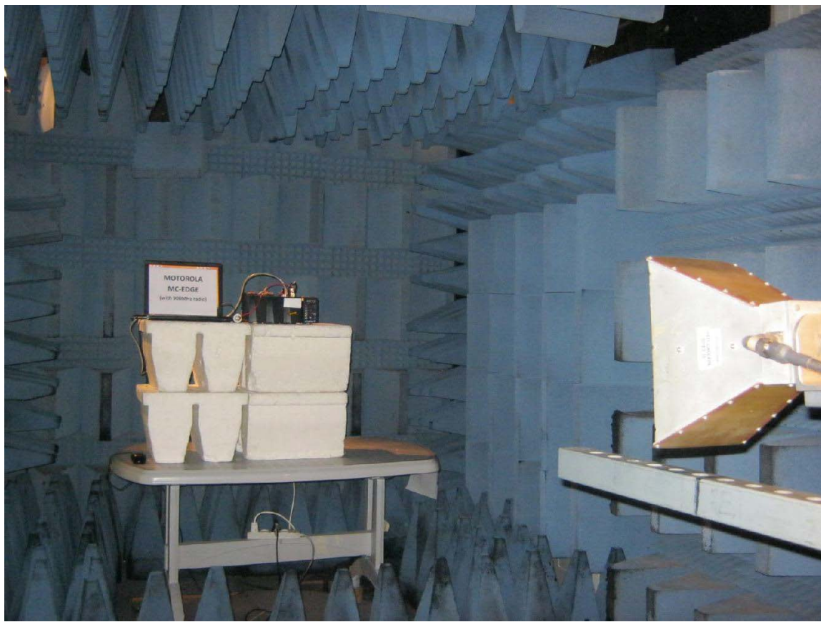
Figure 7 – 4 Radiated Emission Test, 1-10GHz
