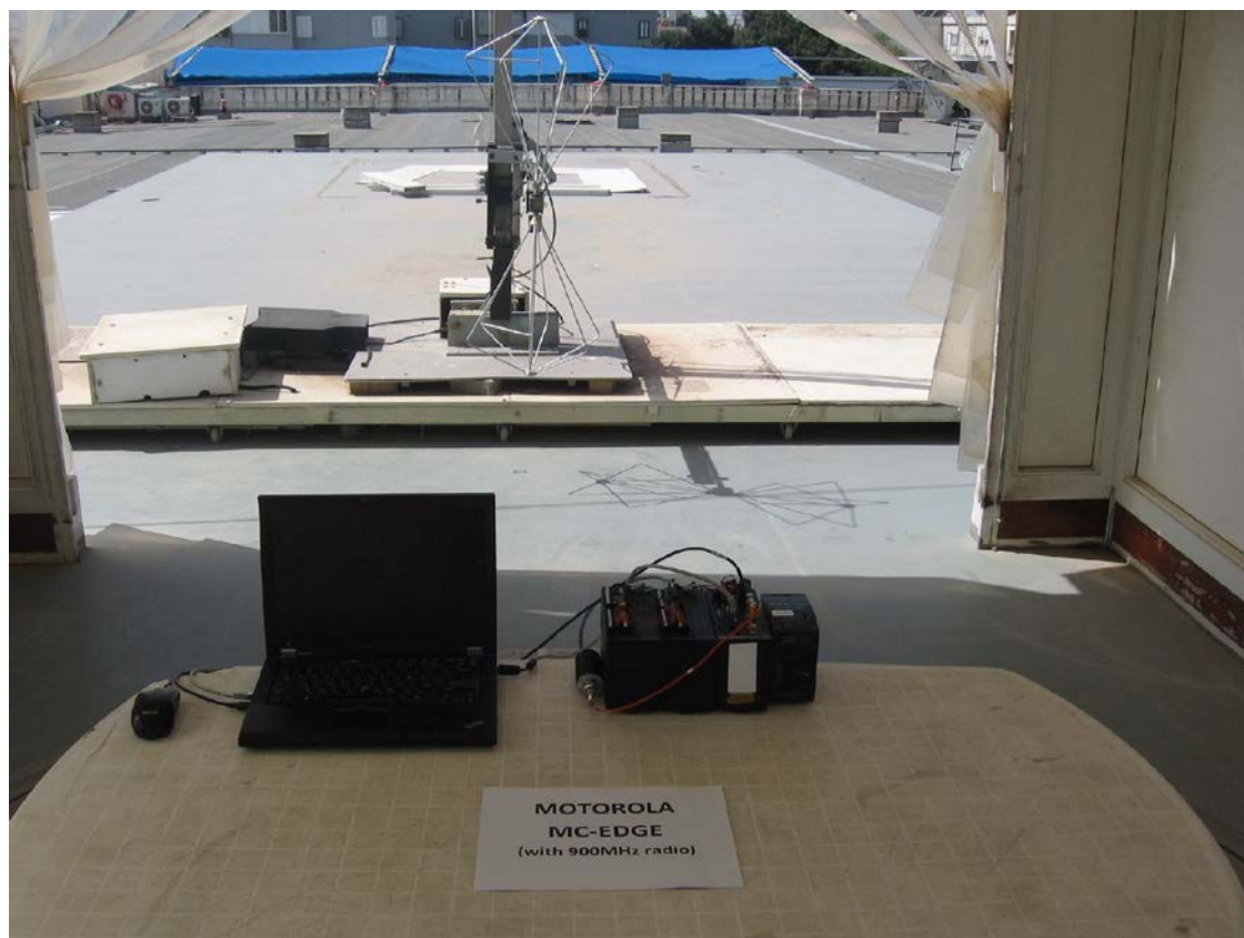
Figure 7 – 2 Radiated Emission Test, 30-200MHz
