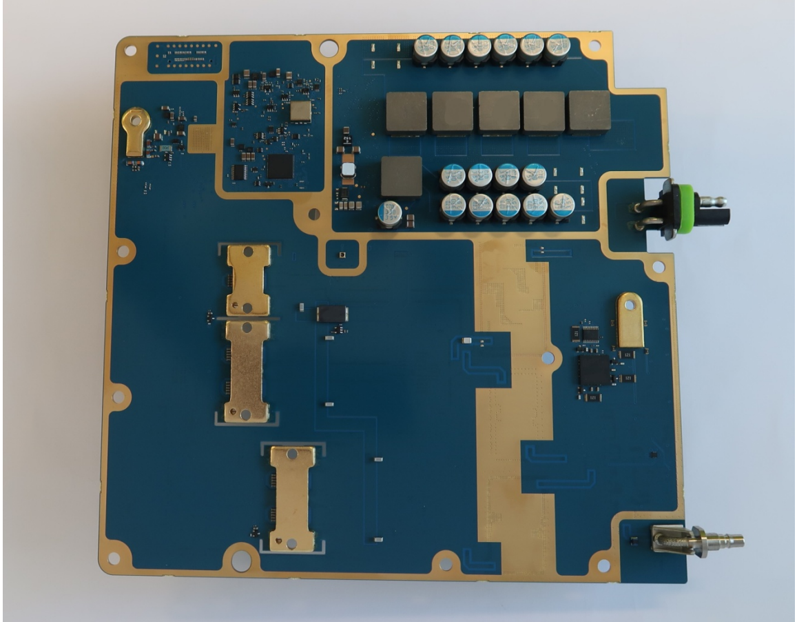
Exhibit 9B: Transmitter Board (Bottom)
