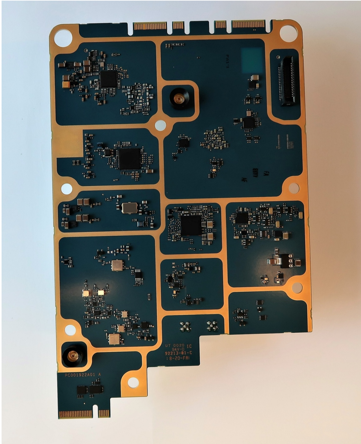
Exhibit 9E: Transceiver Board (Bottom)
