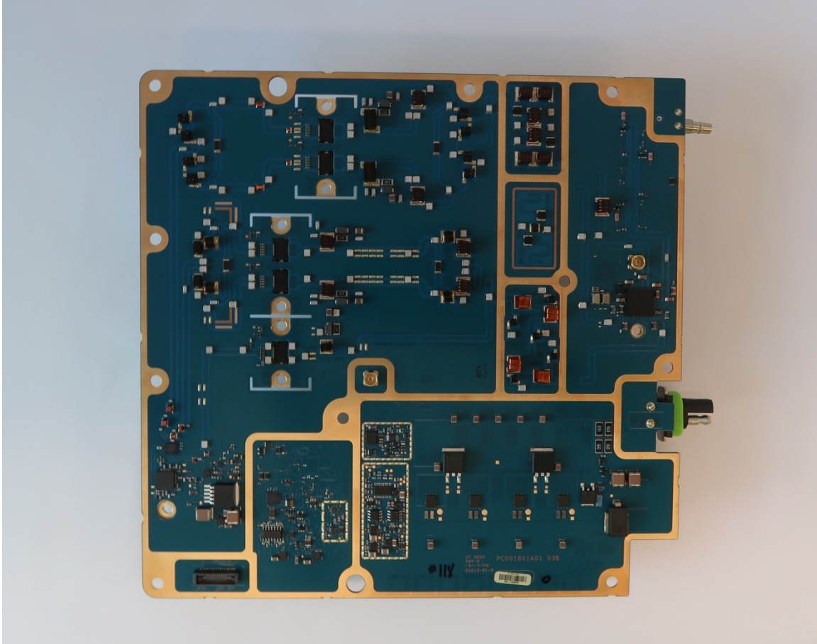
Exhibit 9A: Transmitter Board (Top)
