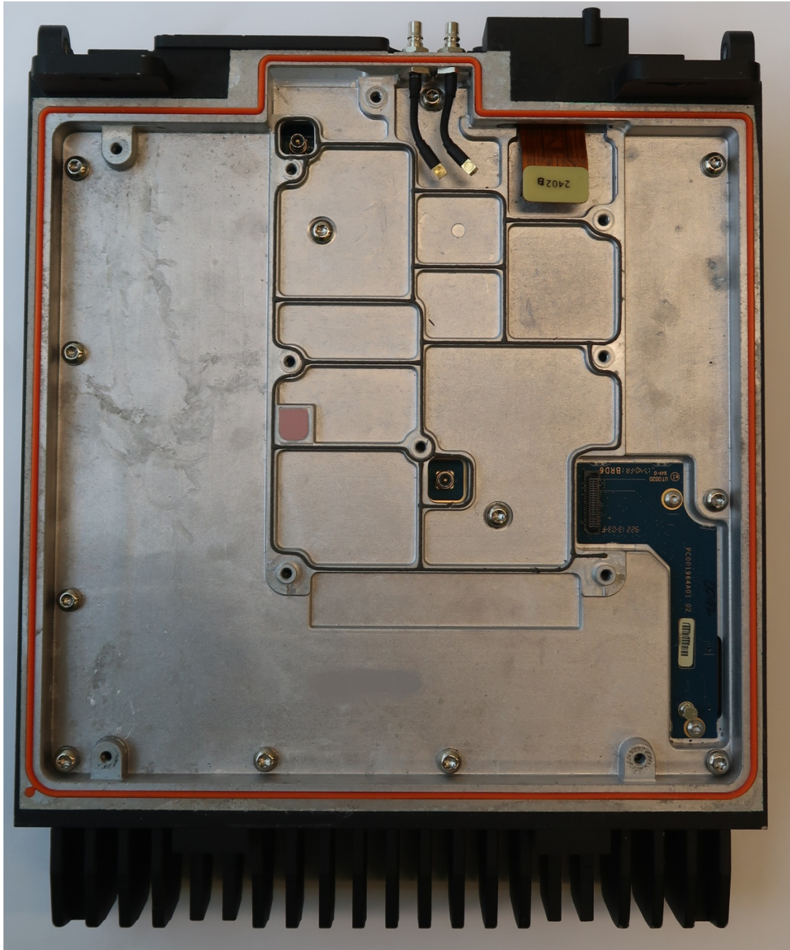
Exhibit 9E: Radio Assembly – Middle Chassis (Top)
