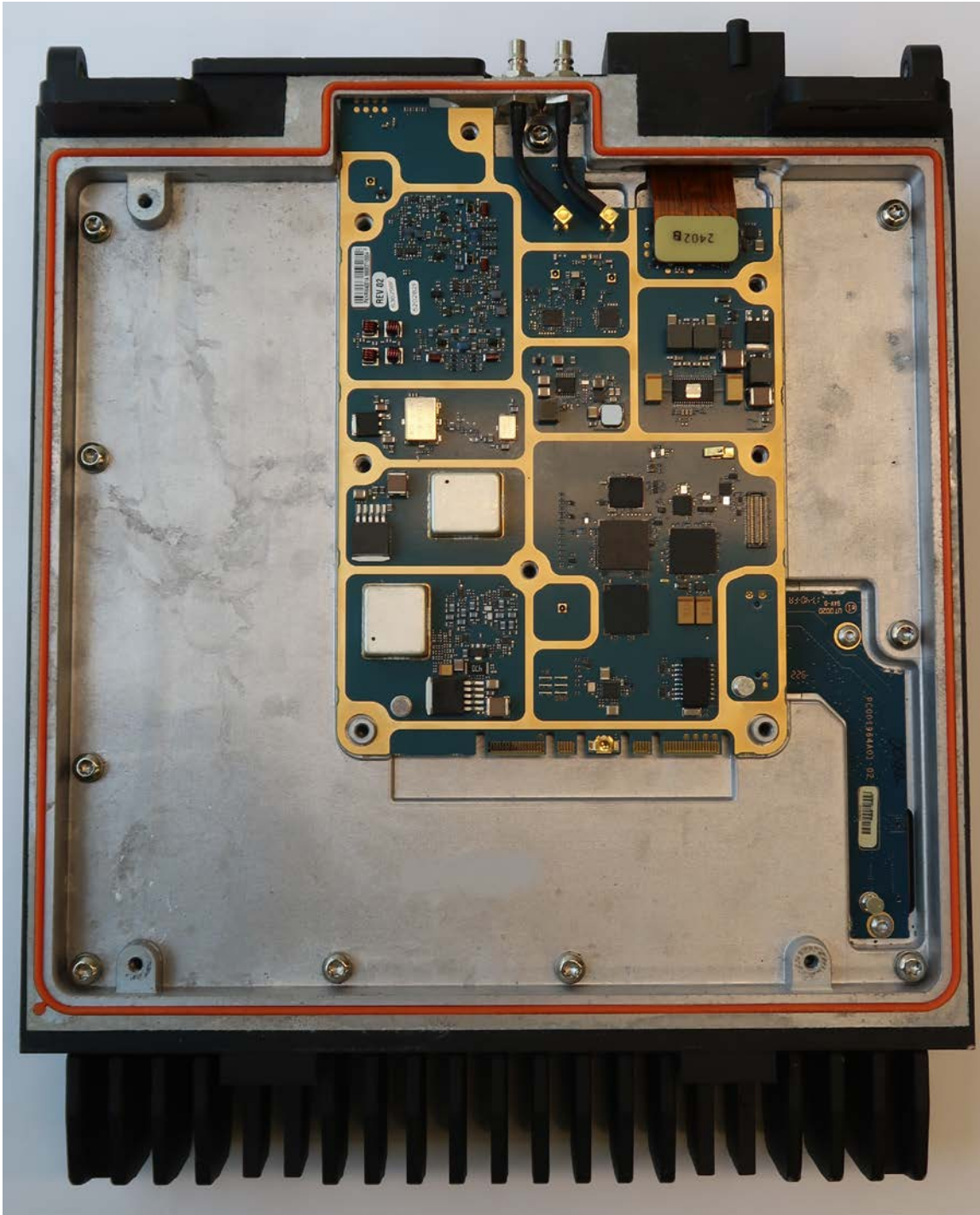
Exhibit 9F: Radio Assembly – Transceiver Board (Top)
