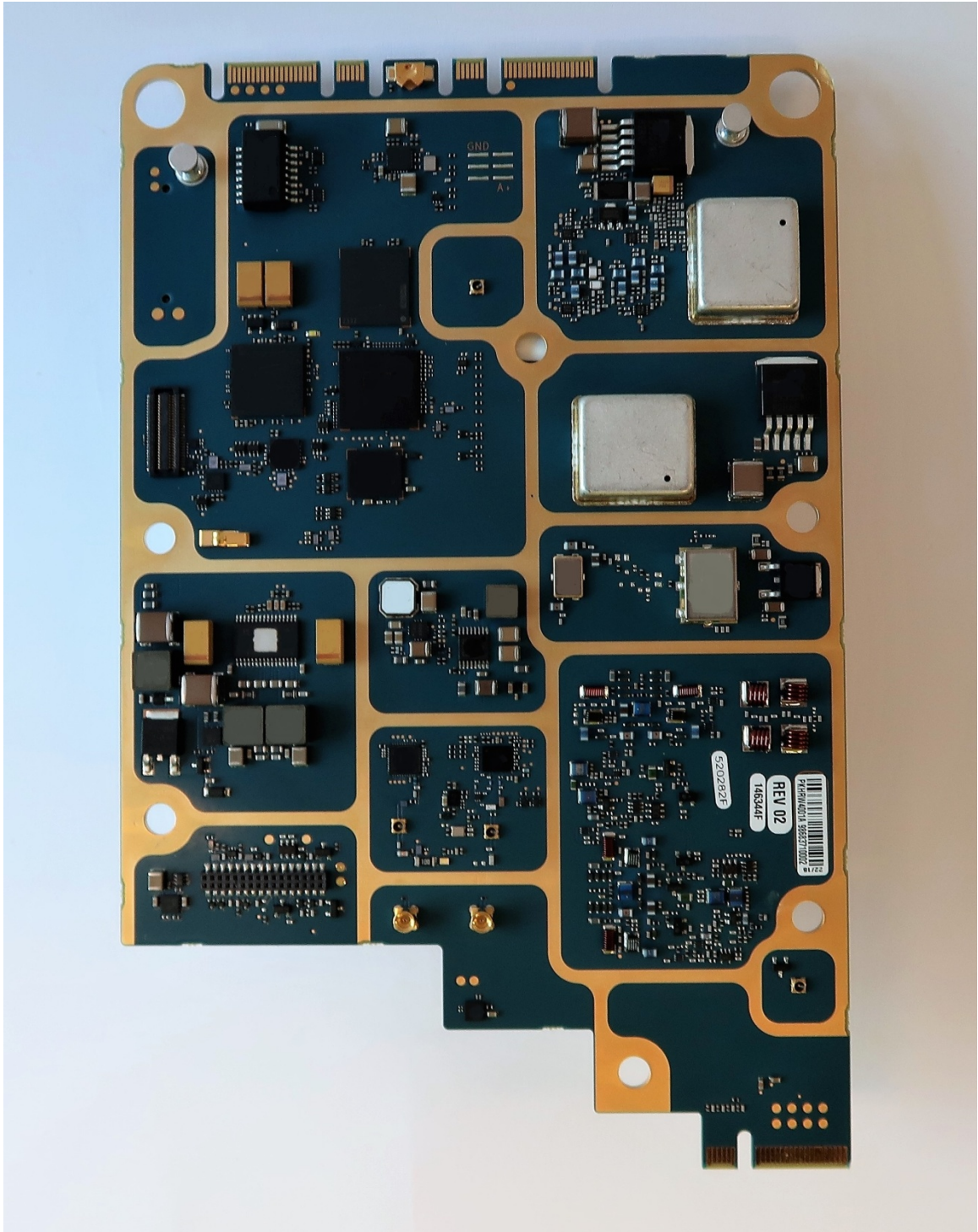
Exhibit 9C: Transceiver Board with Shields (Top)
