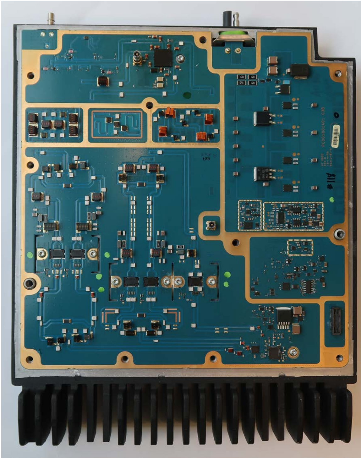
Exhibit 9D: Radio Assembly - Transmitter Board (Top)
