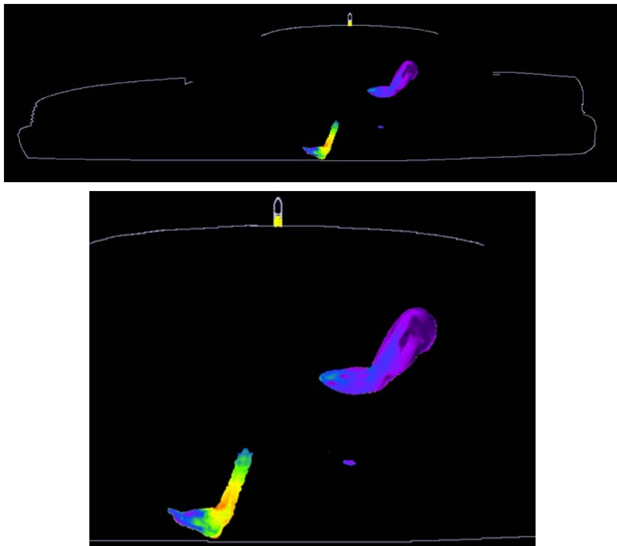
Figure 6. SAR distribution at 158.0125 MHz in the passenger model located on the side of the back seat, produced by the roof-mount AN000131A01 antenna. The contour plot is relative to the plane where the peak 1-g average SAR for this exposure condition occurs.
