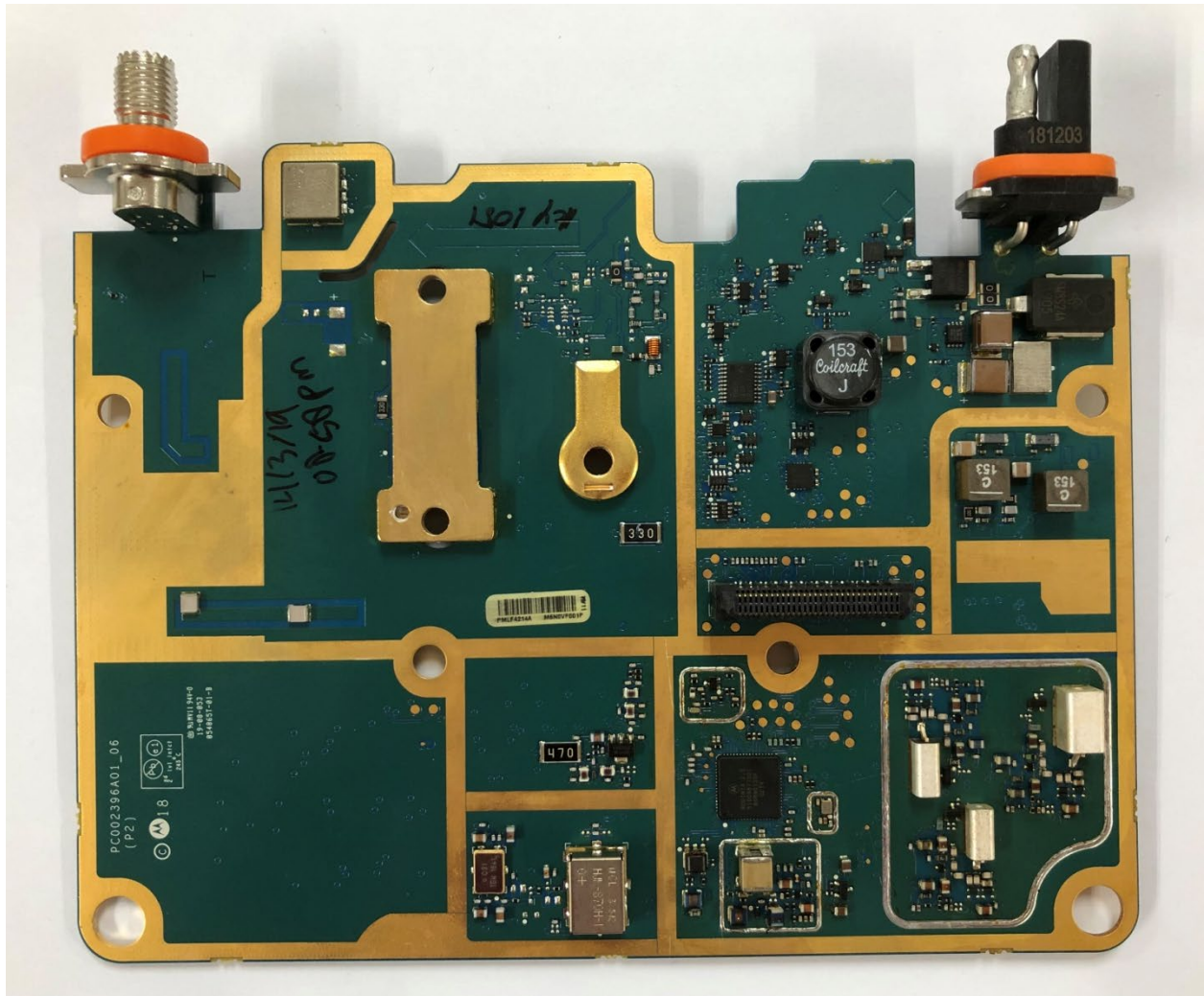
Exhibit 9B: RF Board without Shields (Top)
