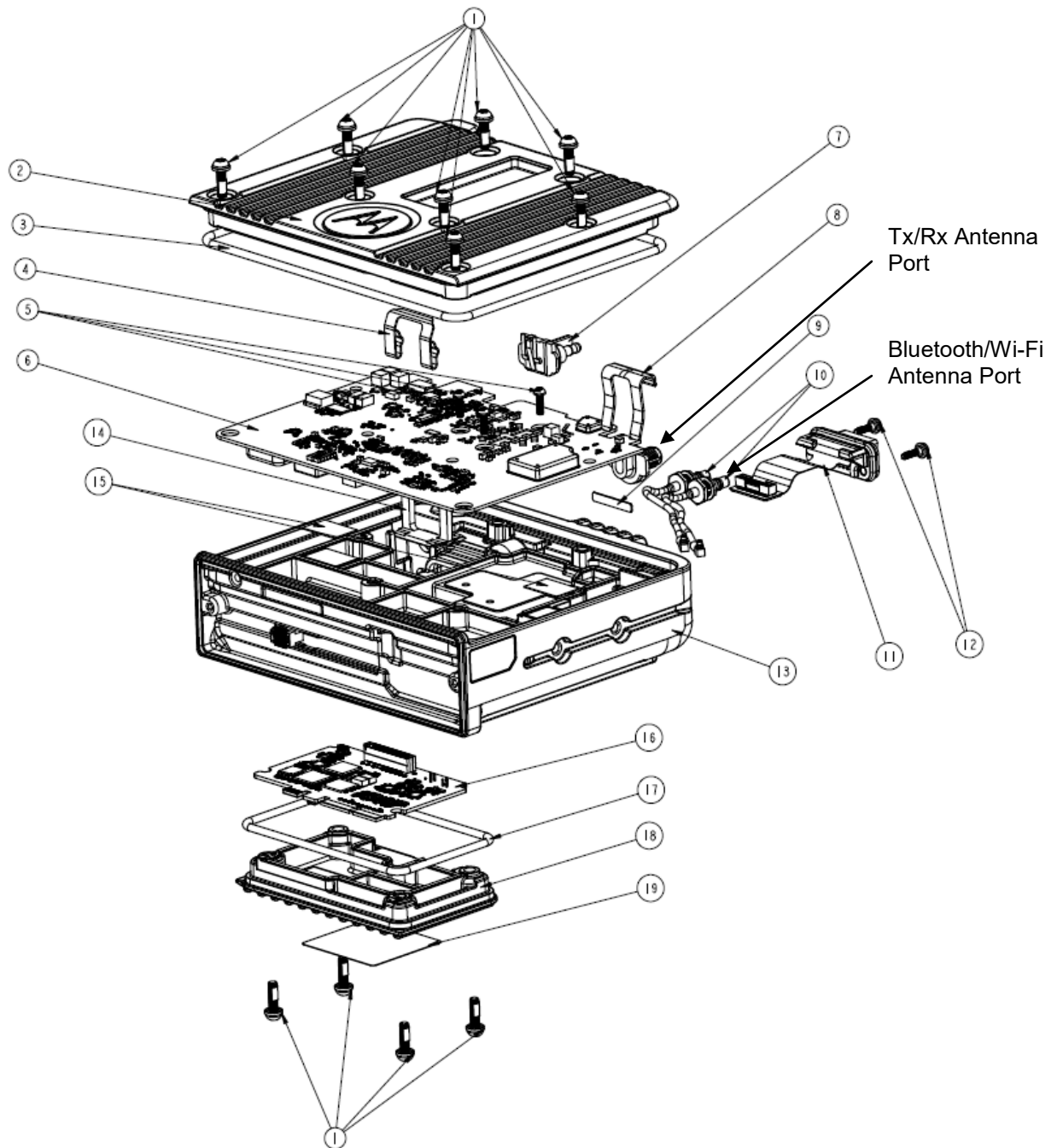
Exhibit 9I: Exploded View
