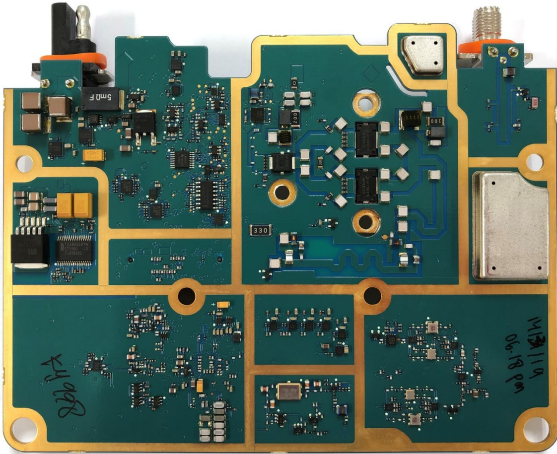
Exhibit 9C: RF Board with Shield (Bottom)
