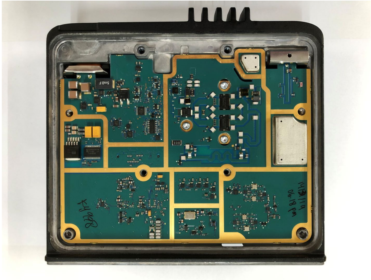
Exhibit 9E: Radio Assembly – RF Board (Top View)
