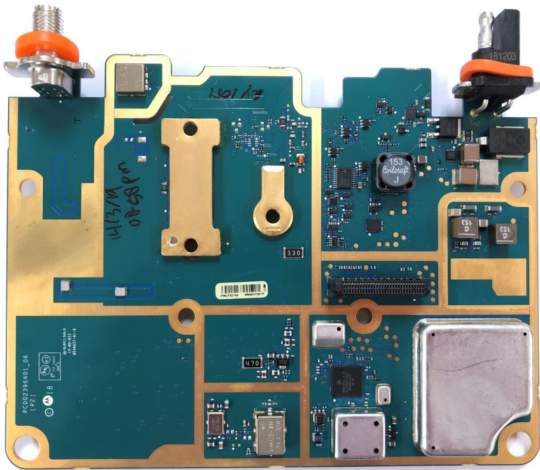
Exhibit 9A: RF Board with Shields (Top)
