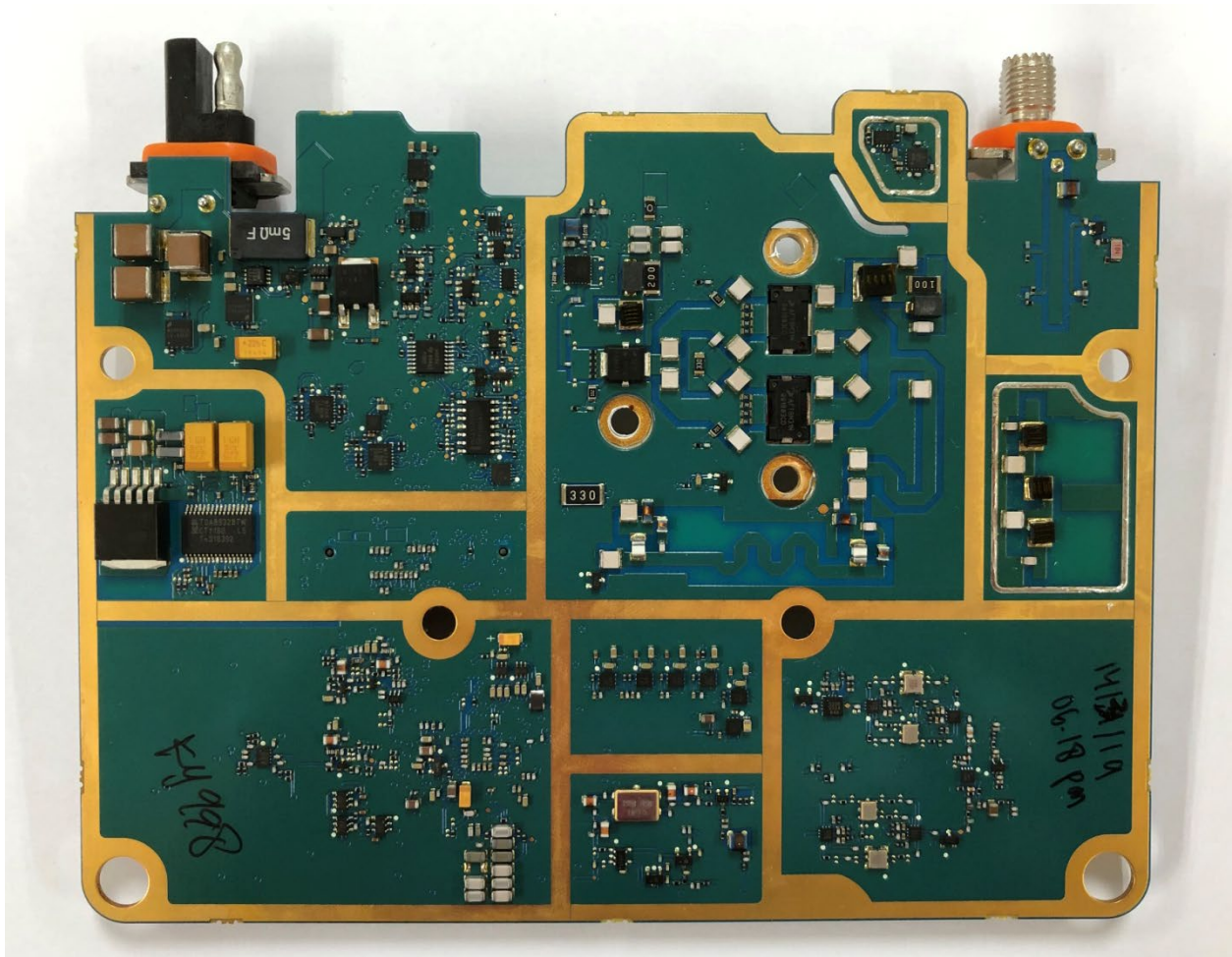
Exhibit 9D: RF Board without Shield (Bottom)
