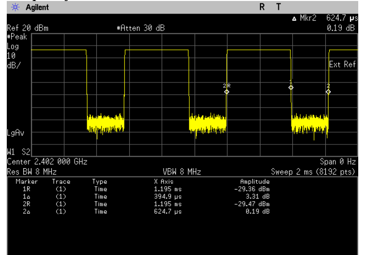
Duty Cycle
