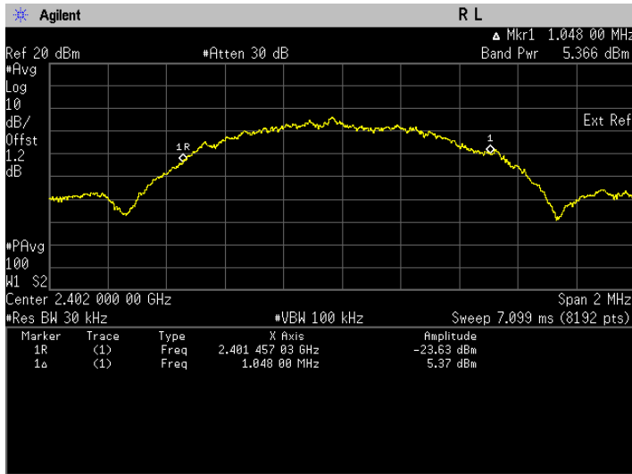
Frequency 2402 MHz
