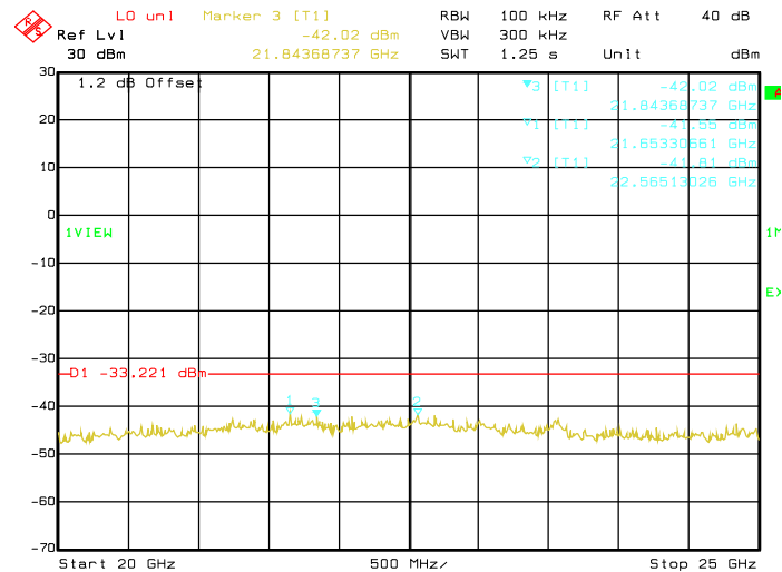
Date: 14.AUG.2019 03:12:04 Conducted Emissions. 802.11g, Frequency 2462 MHz Emission Level, 20 GHz -> 25 GHz
