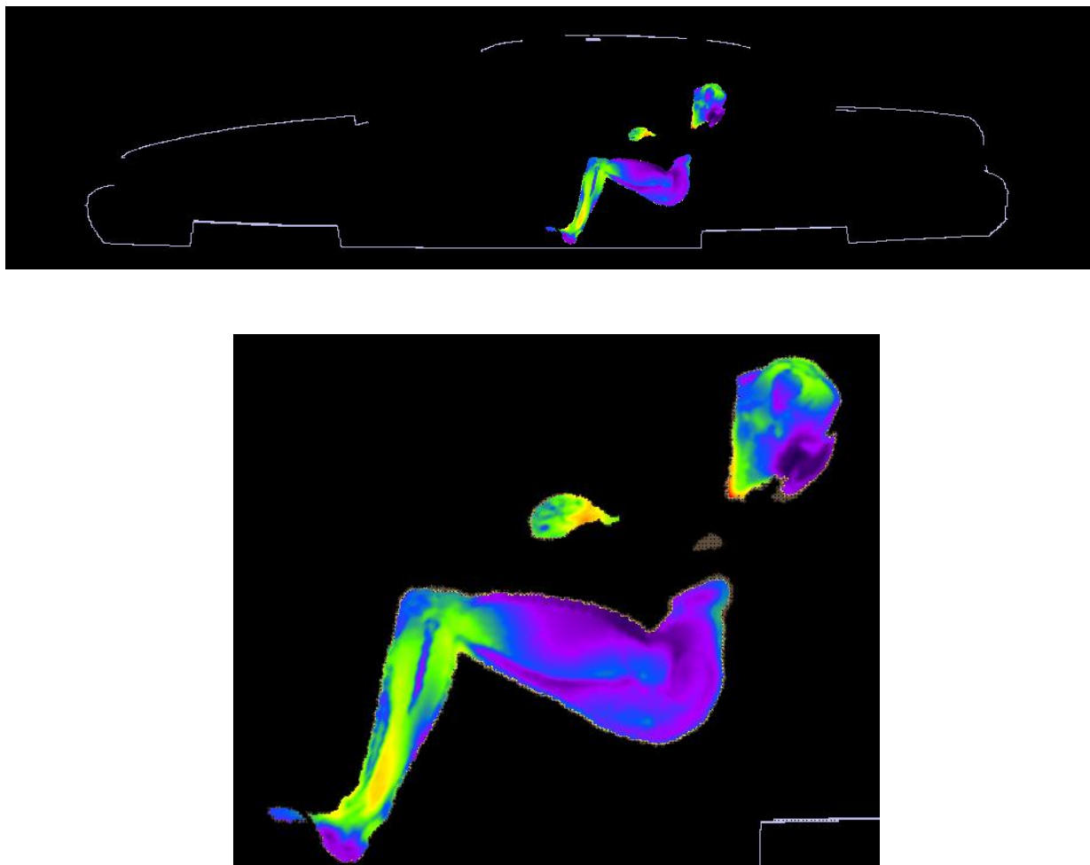
Figure 4. SAR distribution at 173.0125 MHz in the passenger model located on the side of the back seat, produced by the roof-mount HAD4022A antenna. The SAR distribution plot is relative to the plane where the peak 1-g average SAR for this exposure condition occurs.
