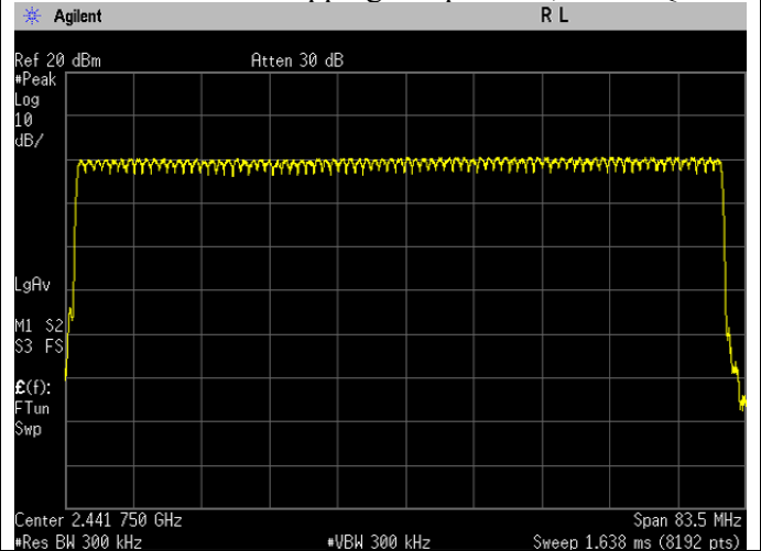
ii. Number of Hopping Frequencies, Pi/4 DQPSK
