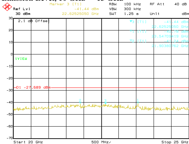
Conducted Emissions. 802.11b, Frequency 2437 MHz Emission Level, 20 GHz -> 25 GHz
