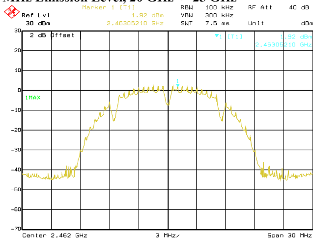
Conducted Emissions. 802.11b, Frequency 2462 MHz Reference Level
