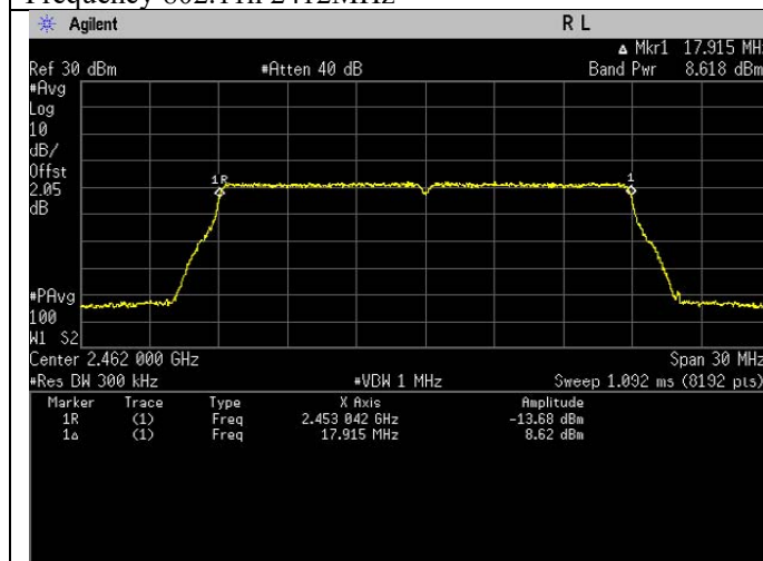
Frequency 802.11n 2462MHz
