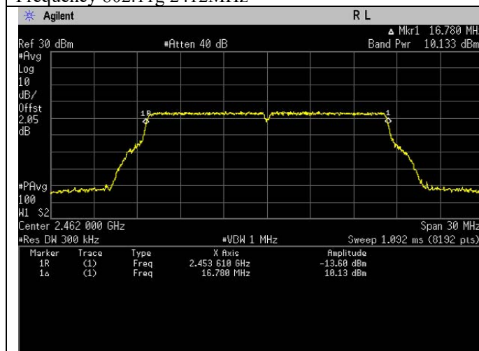
Frequency 802.11g 2462MHz
