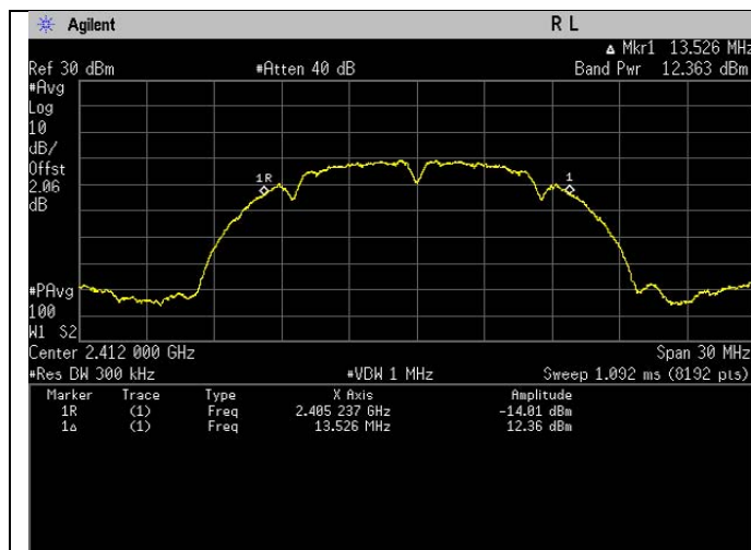
Frequency 802.11b 2412MHz
