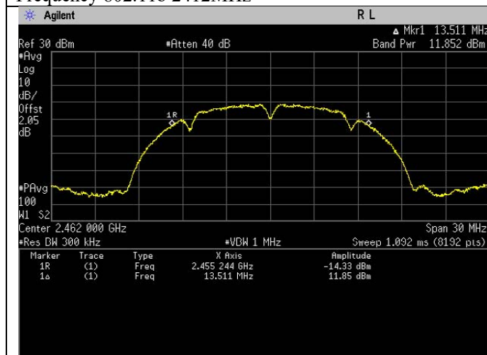
Frequency 802.11b 2462MHz
