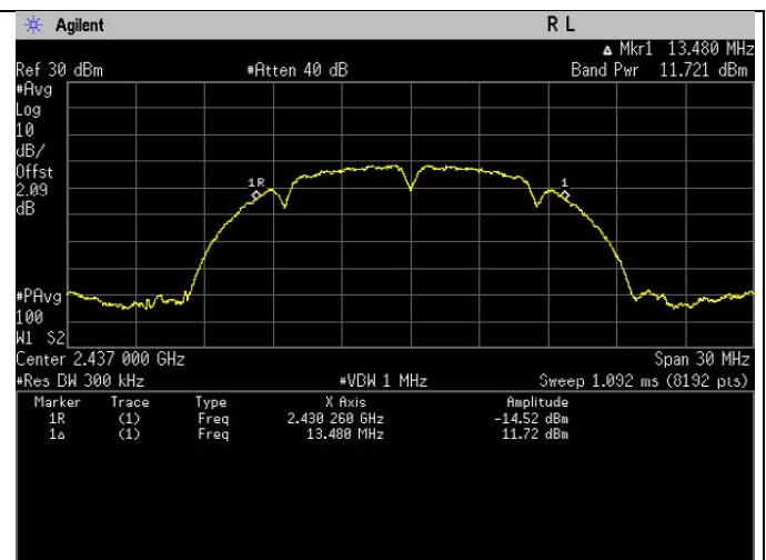
Frequency 802.11b 2437MHz
