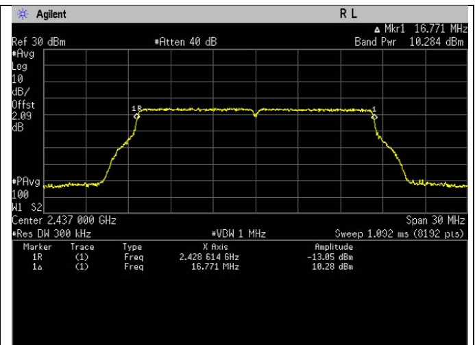
Frequency 802.11g 2437MHz
