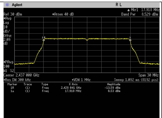
Frequency 802.11n 2437MHz
