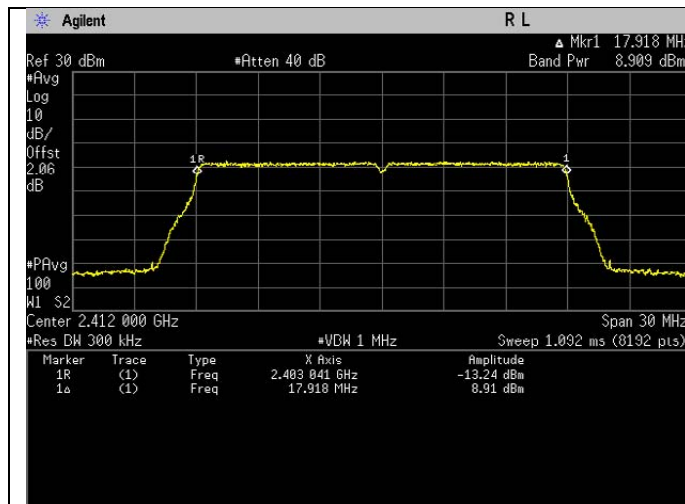
Frequency 802.11n 2412MHz
