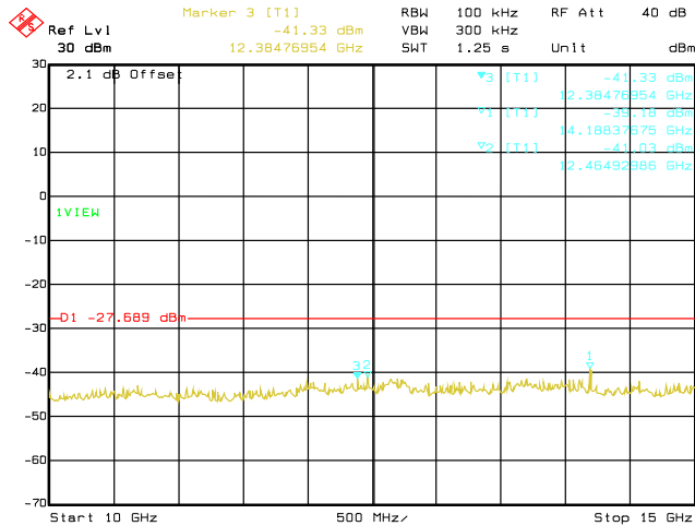
Conducted Emissions. 802.11b, Frequency 2437 MHz Emission Level, 10 GHz -> 15 GHz
