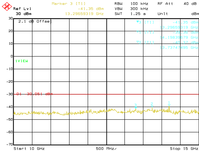
Conducted Emissions. 802.11g, Frequency 2412 MHz Emission Level, 10 GHz -> 15 GHz
