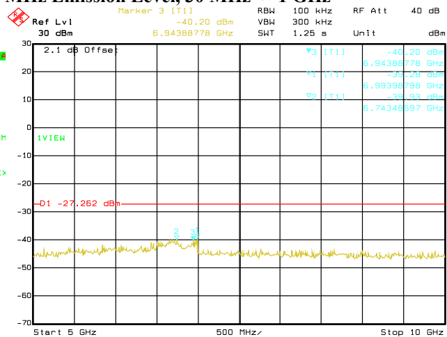
Conducted Emissions. 802.11b, Frequency 2412 MHz Emission Level, 5 GHz -> 10 GHz
