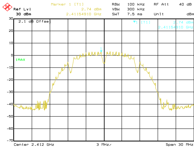
Conducted Emissions. 802.11b, Frequency 2412 MHz Reference Level
