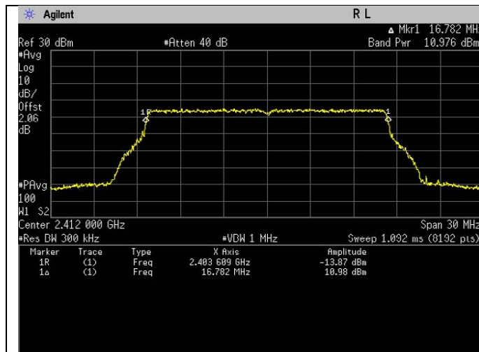
Frequency 802.11g 2412MHz
