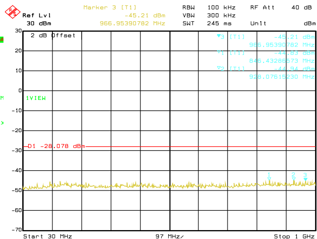
Conducted Emissions. 802.11b, Frequency 2462 MHz Emission Level, 30 MHz -> 1 GHz
