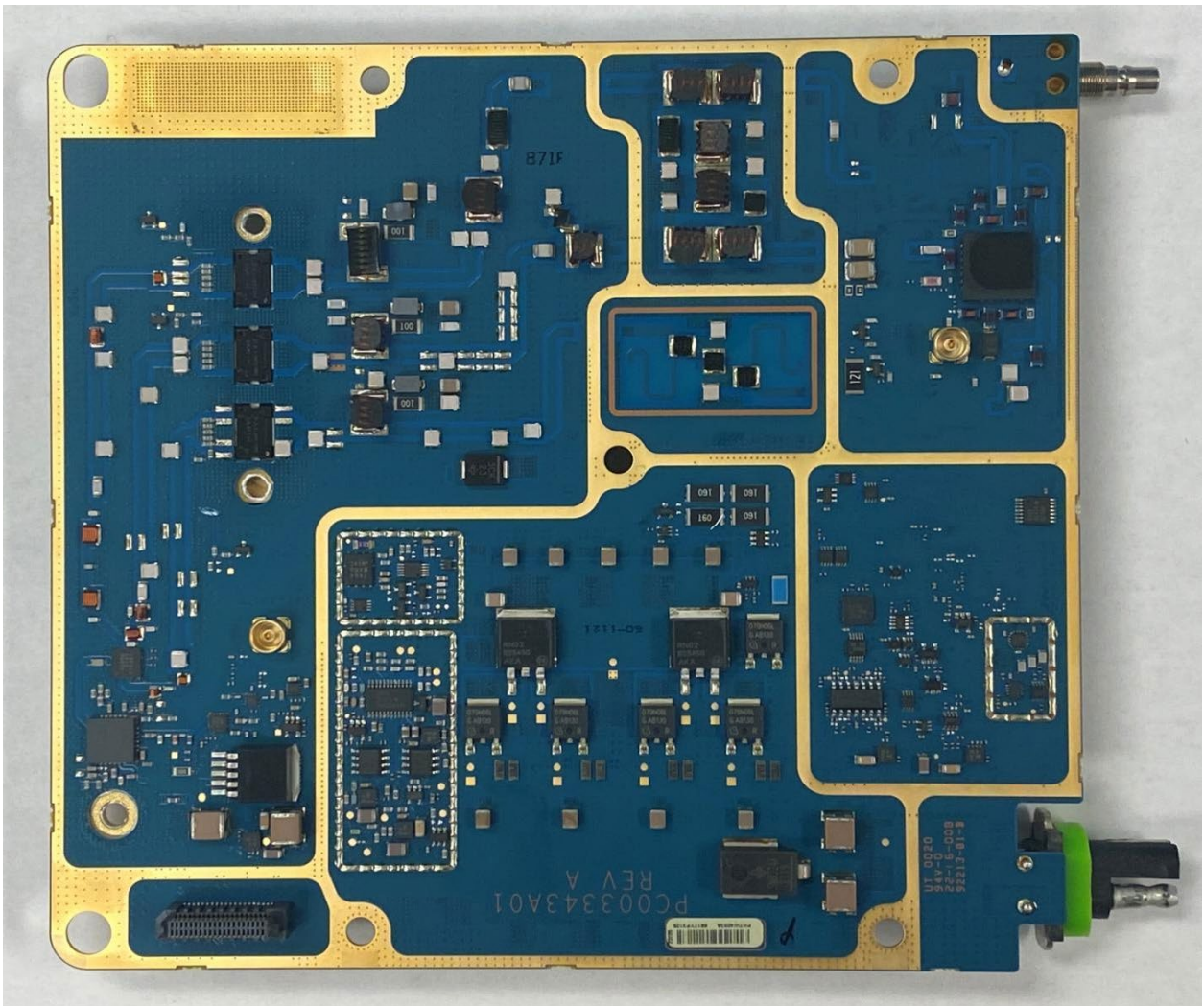
Exhibit 9A: Transmitter Board (Top)
