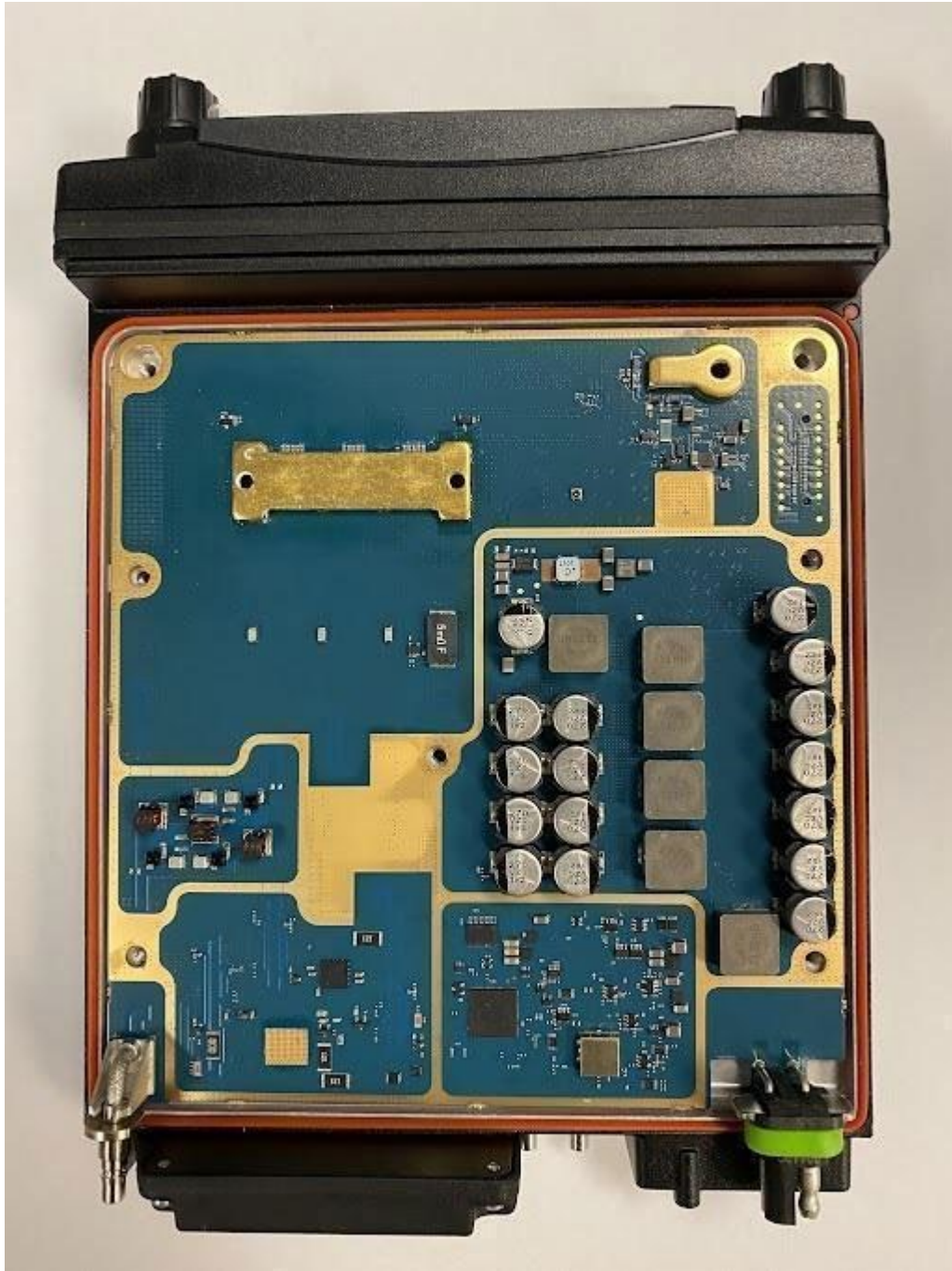
Exhibit 9F: Radio Assembly – Transmitter Board (Top) new
