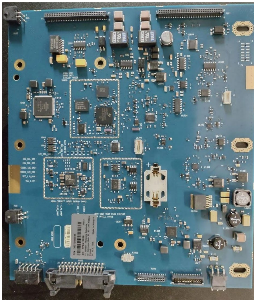
Exhibit 9M: Main board without shield (Top)
