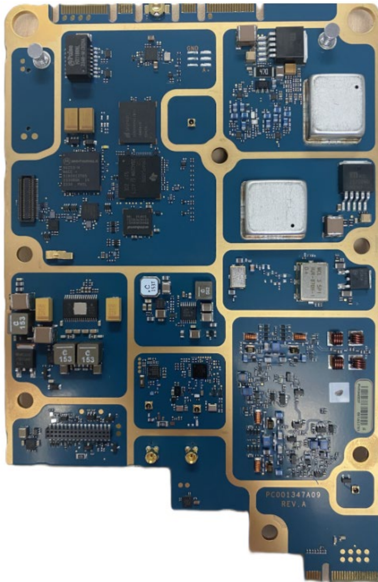
Exhibit 9C: Transceiver Board with Shields (Top)
