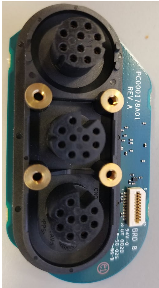
Exhibit 9J: TIB Assembly Bottom Side
