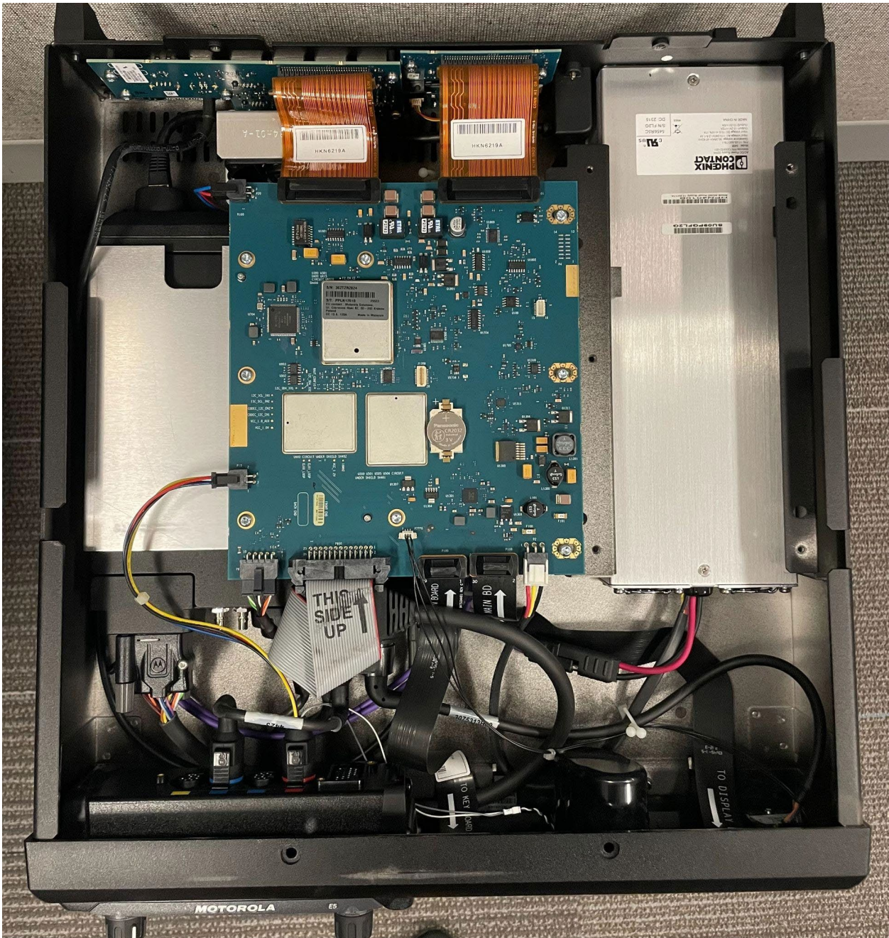
Exhibit 9K: Consolette (Top)
