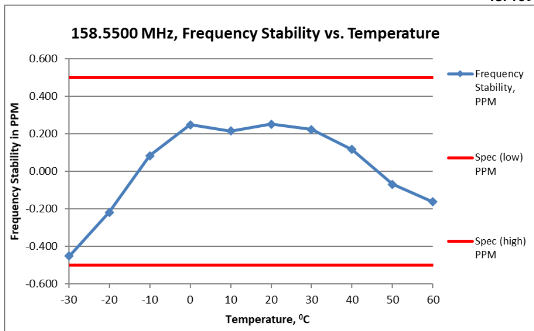
(ii) Frequency Stability VS temperature
