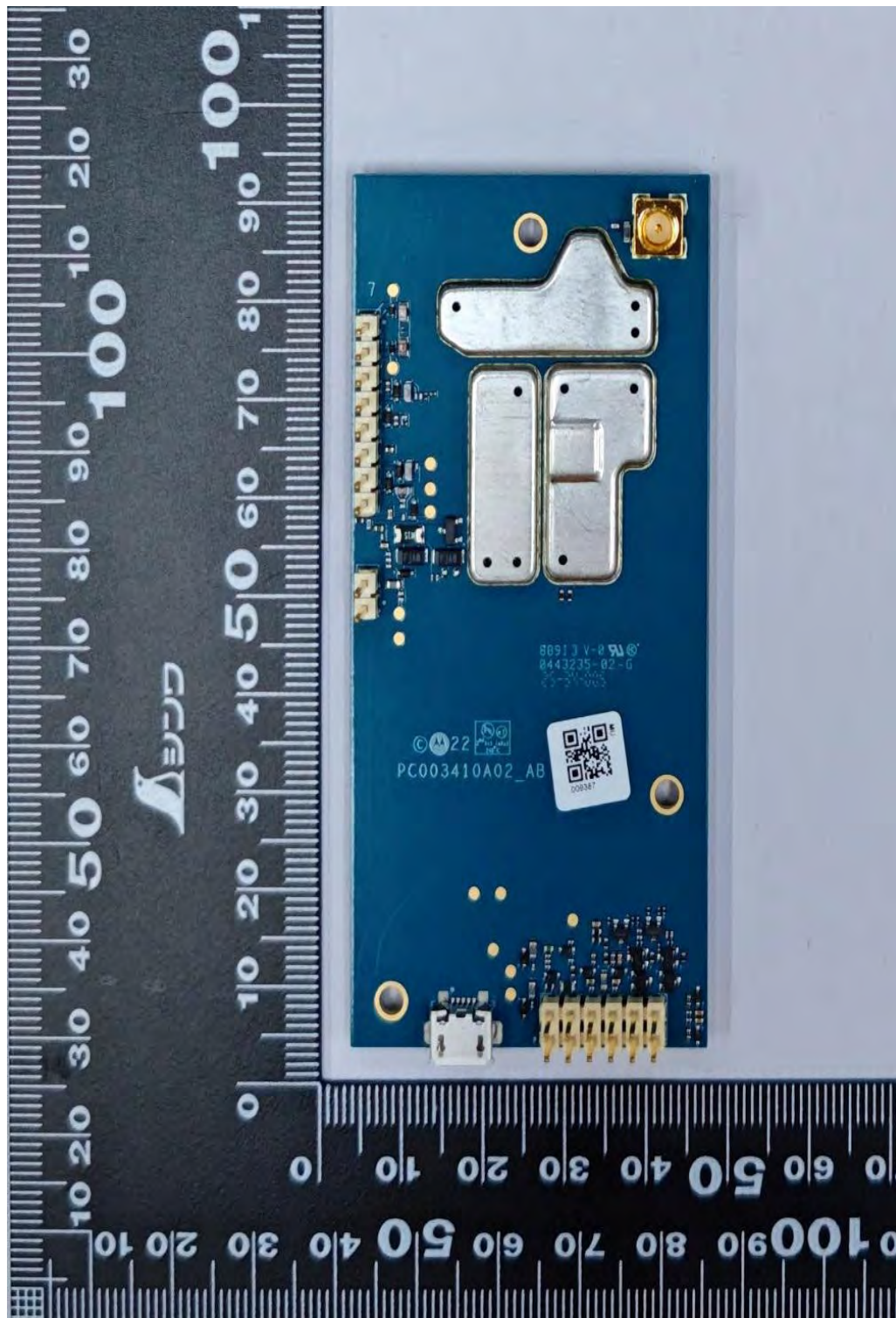
RF Board with Shields (Top) - CBS101NBKLBA (CB900D) CB900D 2-Way Call Box
