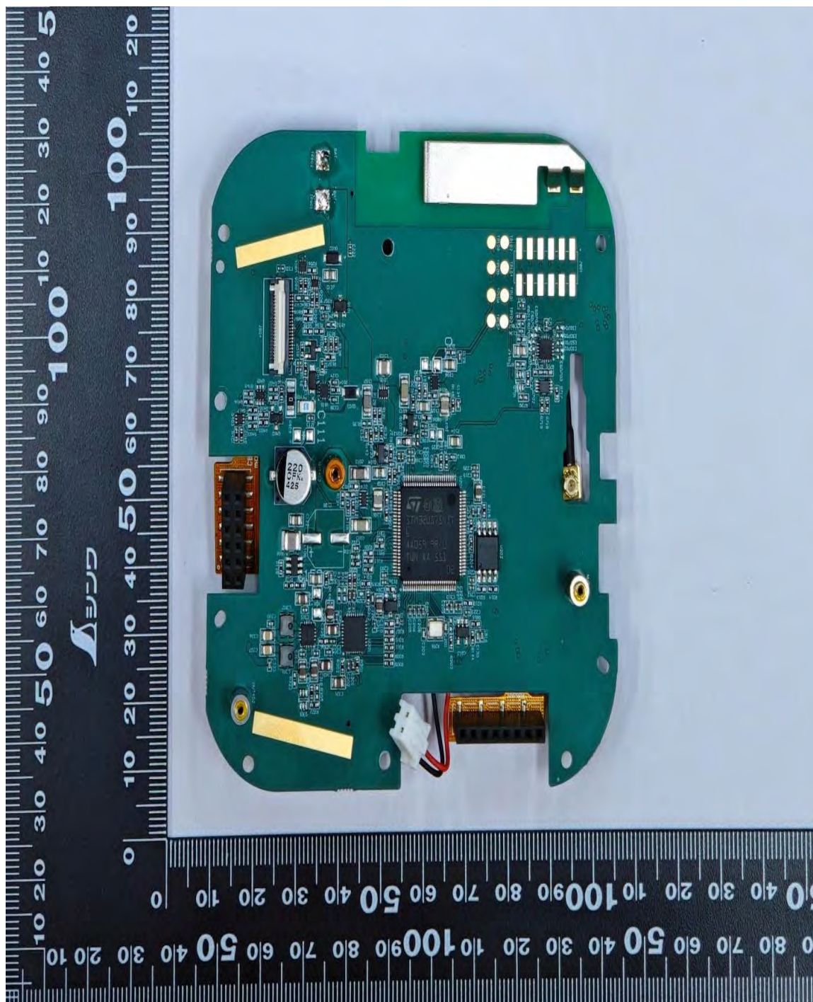
Main Board (Bottom) - BSS101NBKLBA (CB900D) CB900D Base Station
