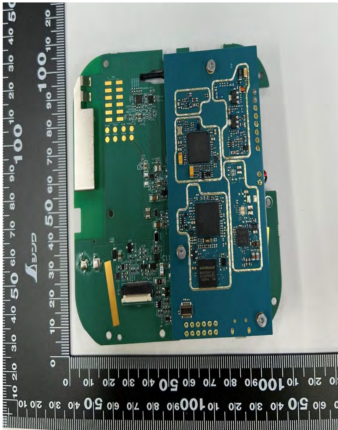
Main Board with RF Board (Bottom) - CBS101NBKLBA (CB900D) CB900D 1-Way Call Box
