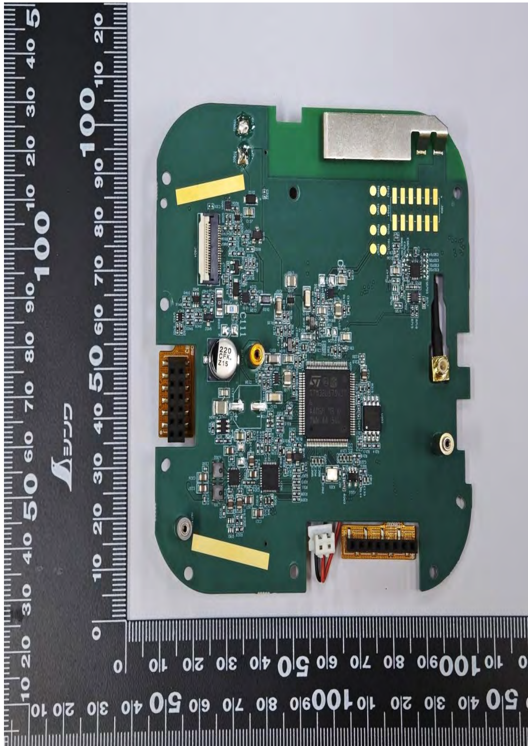
Main Board (Bottom) - CBS101NBKLBA (CB900D) CB900D 2-Way Call Box
