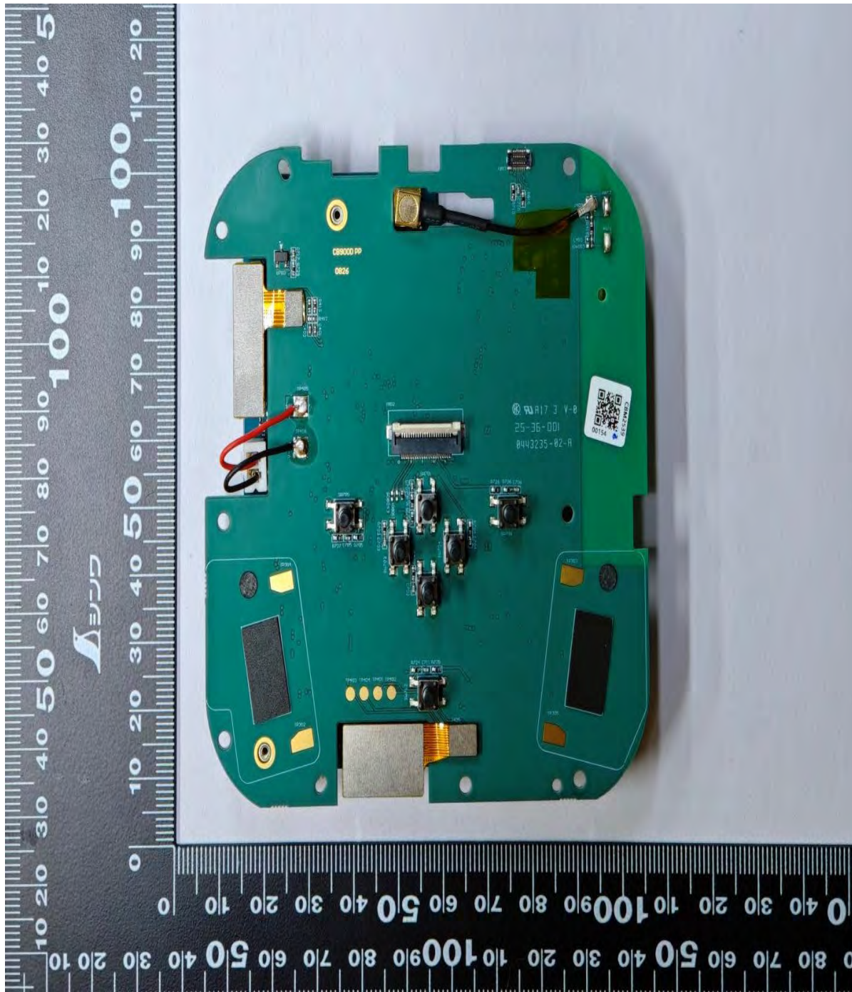
Main Board with RF Board (Top) - BSS101NBKLBA (CB900D) CB900D Base Station
