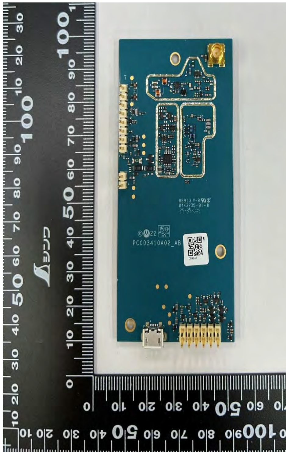
RF Board without Shields (Top) - CBS101NBKLBA (CB900D) CB900D 1-Way Call Box
