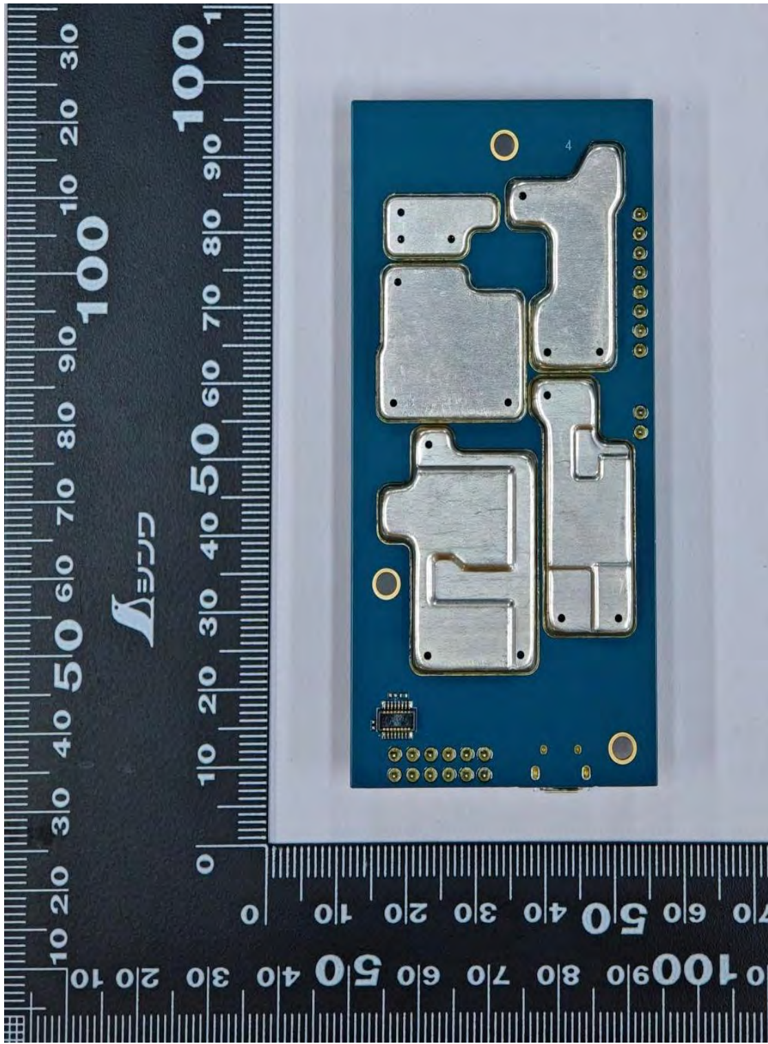
RF Board with Shields (Bottom) - BSS101NBKLBA (CB900D) CB900D Base Station
