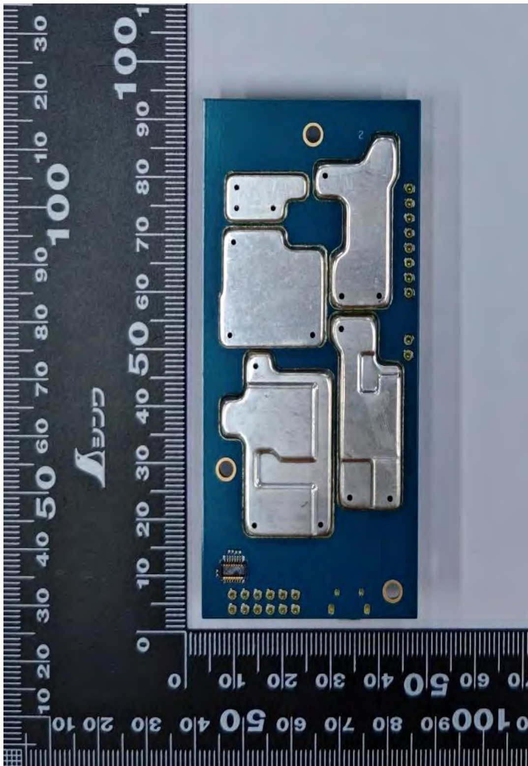
RF Board with Shields (Bottom) - CBS101NBKLBA (CB900D) CB900D 2-Way Call Box
