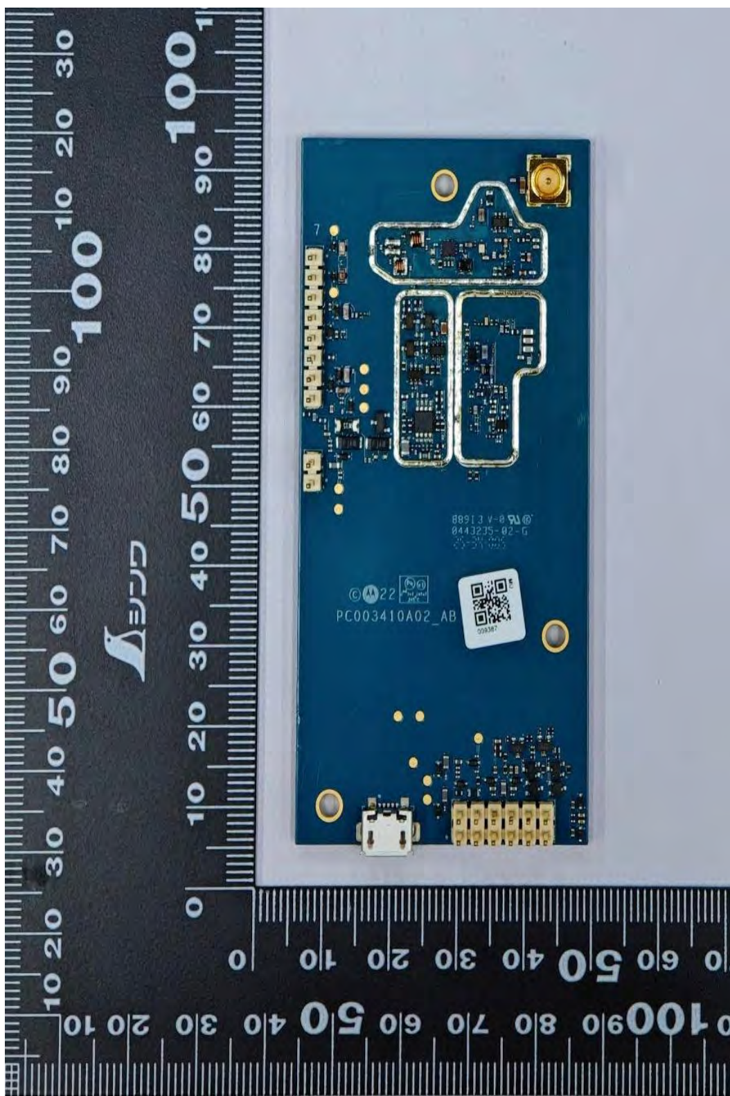
RF Board without Shields (Top) - CBS101NBKLBA (CB900D) CB900D 2-Way Call Box
