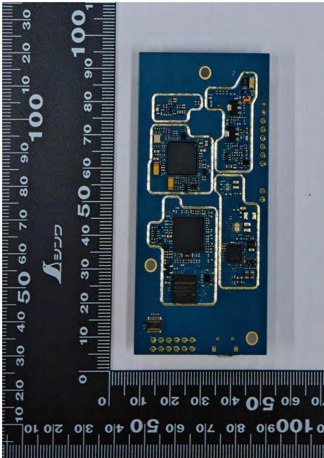
RF Board without Shields (Bottom) - BSS101NBKLBA (CB900D) CB900D Base Station
