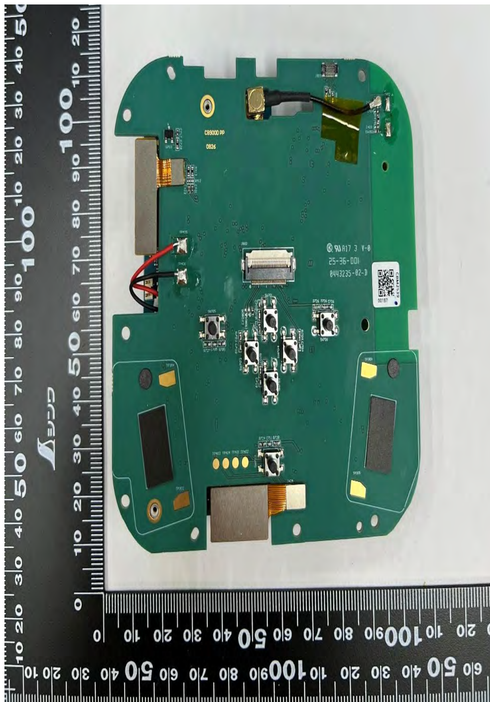
Main Board with RF Board (Top) - CBS101NBKLBA (CB900D) CB900D 1-Way Call Box
