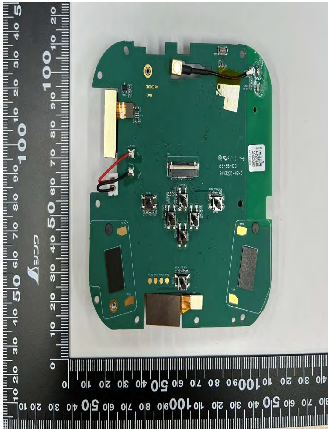
Main Board (Top) - CBS101NBKLBA (CB900D) CB900D 1-Way Call Box
