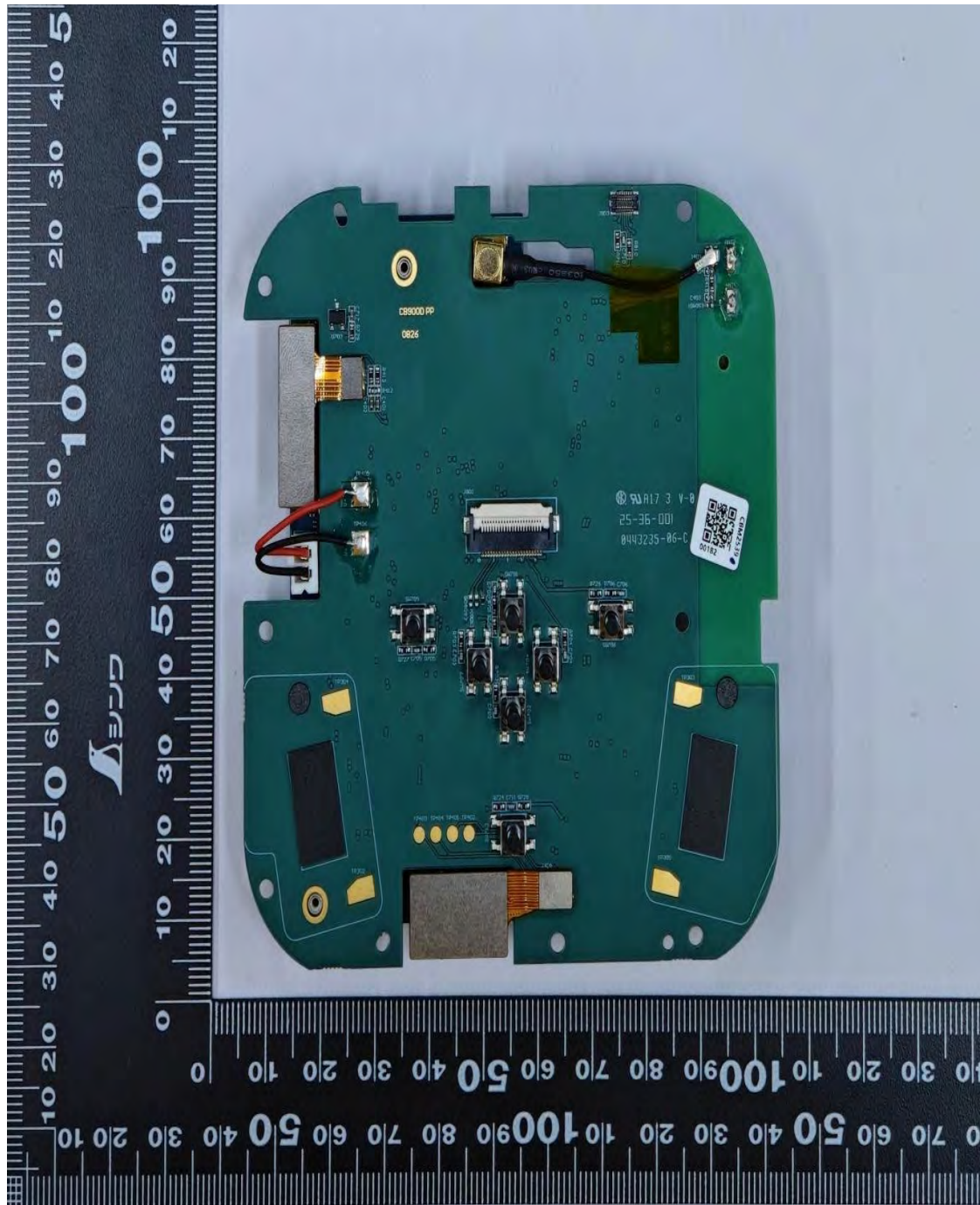
Main Board with RF Board (Top) - CBS101NBKLBA (CB900D) CB900D 2-Way Call Box
