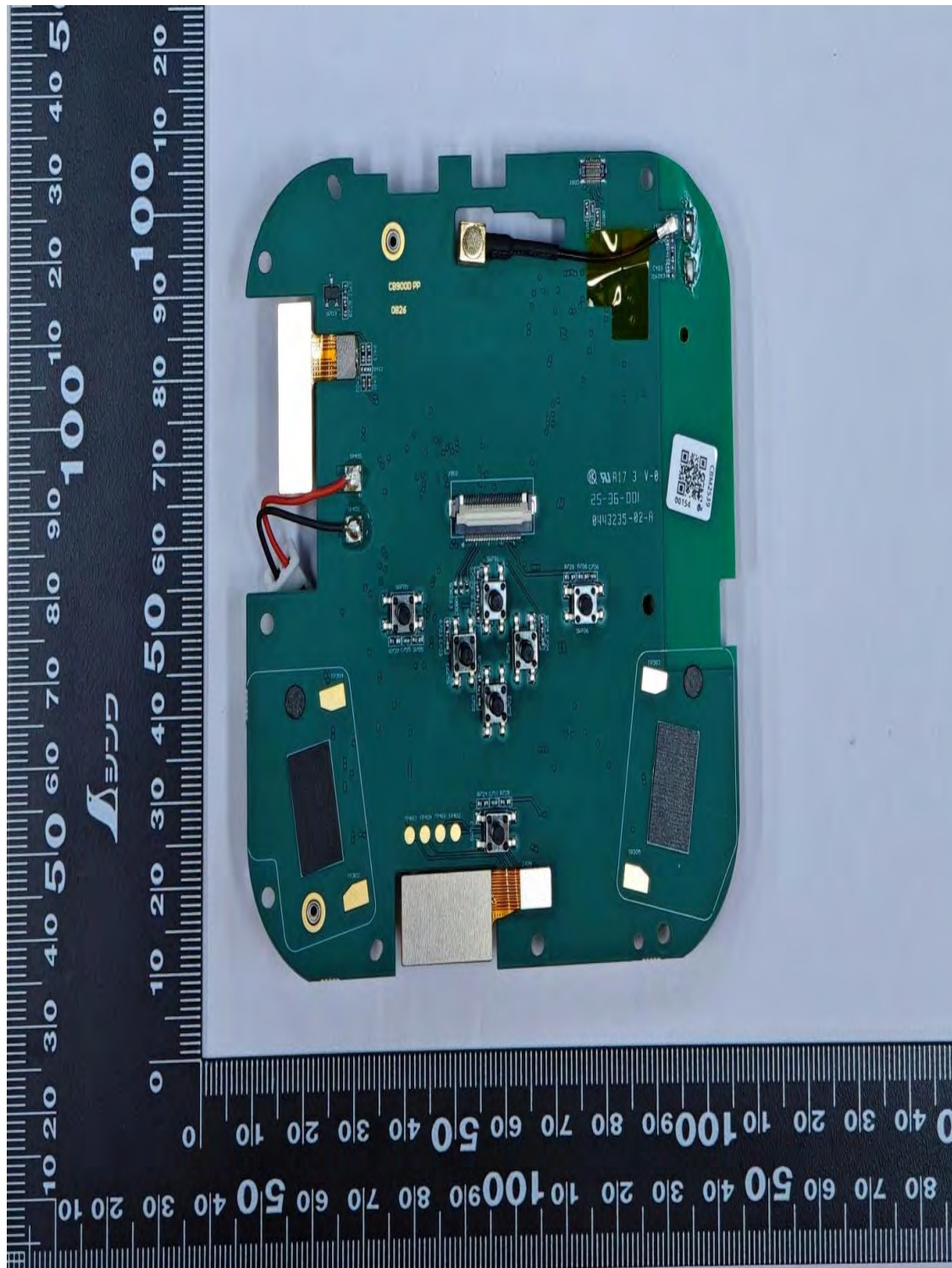
Main Board (Top) - BSS101NBKLBA (CB900D) CB900D Base Station
