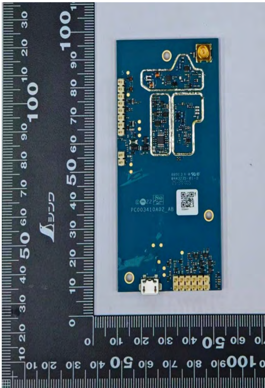
RF Board without Shields (Top) - BSS101NBKLBA (CB900D) CB900D Base Station
