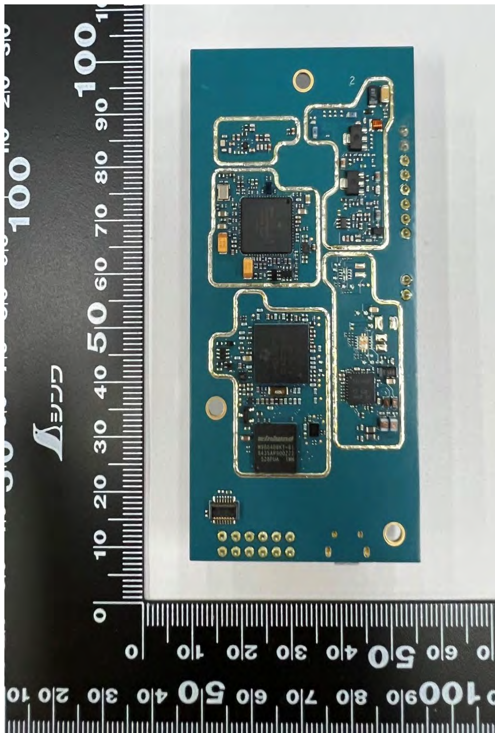
RF Board without Shields (Bottom) - CBS101NBKLBA (CB900D) CB900D 1-Way Call Box
