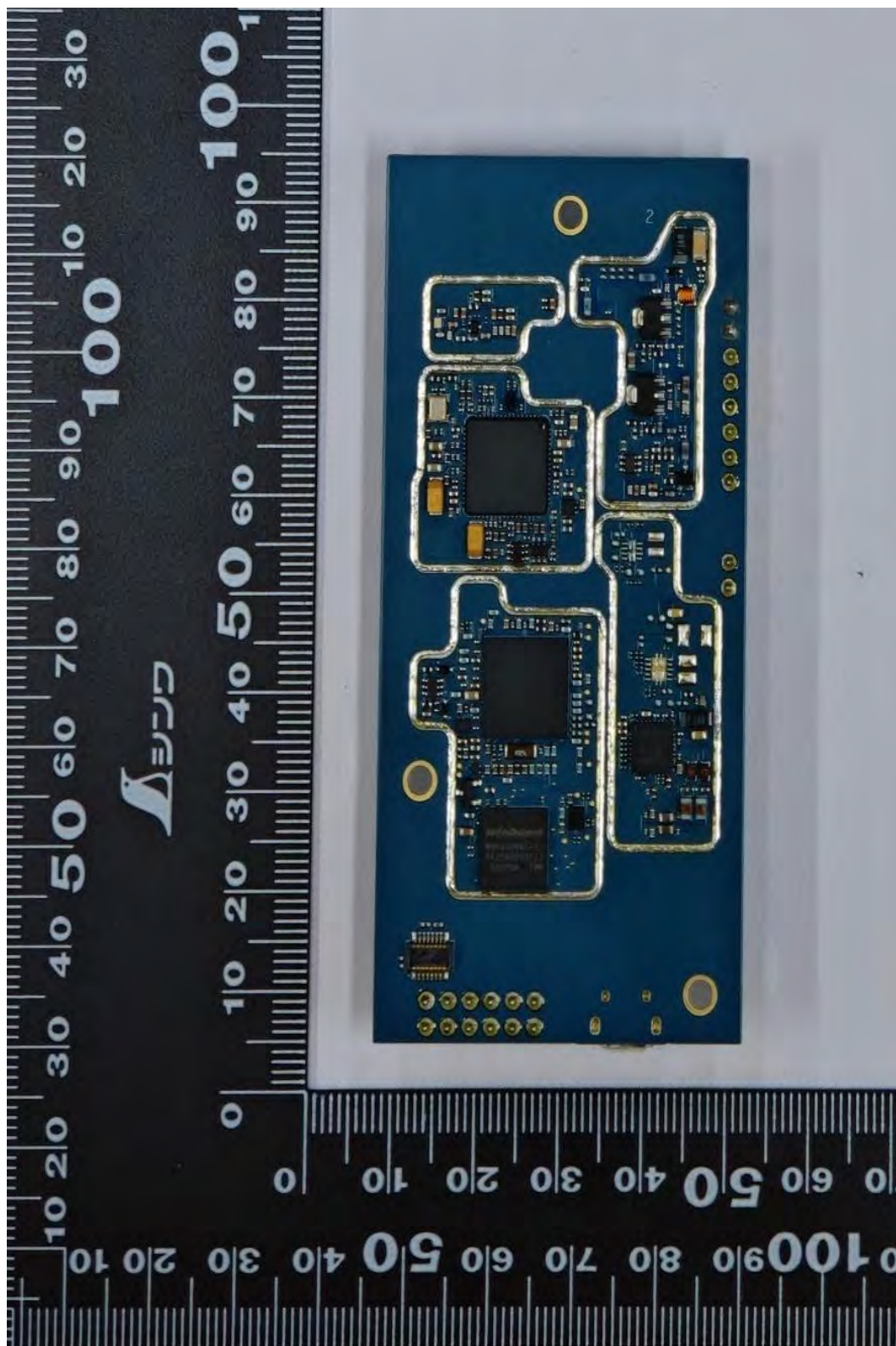
RF Board without Shields (Bottom) - CBS101NBKLBA (CB900D) CB900D 2-Way Call Box
