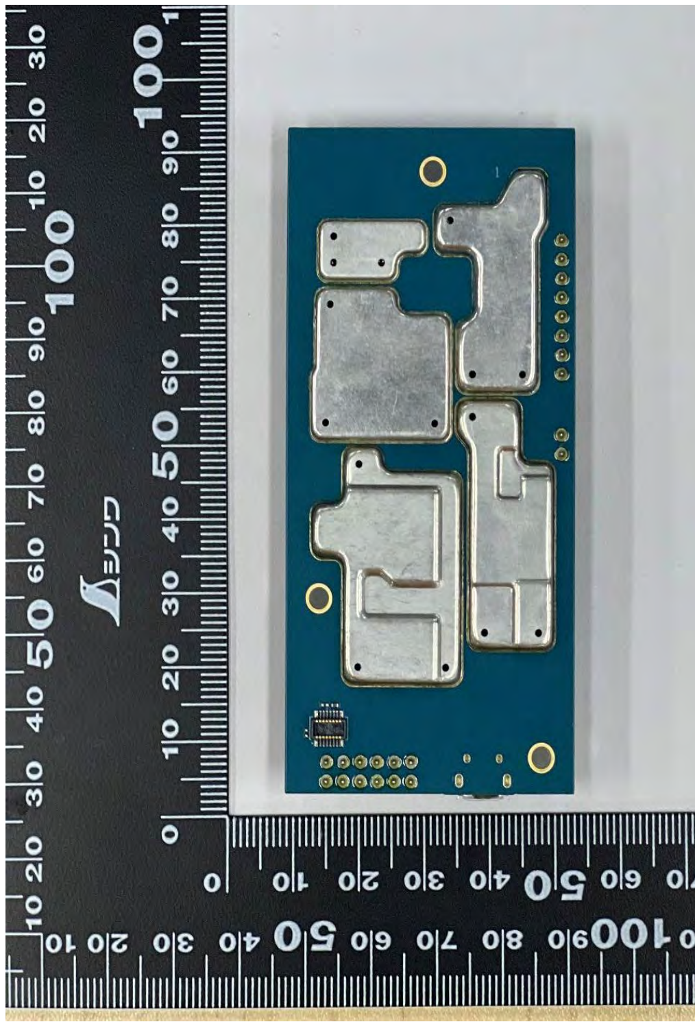
RF Board with Shields (Bottom) - CBS101NBKLBA (CB900D) CB900D 1-Way Call Box
