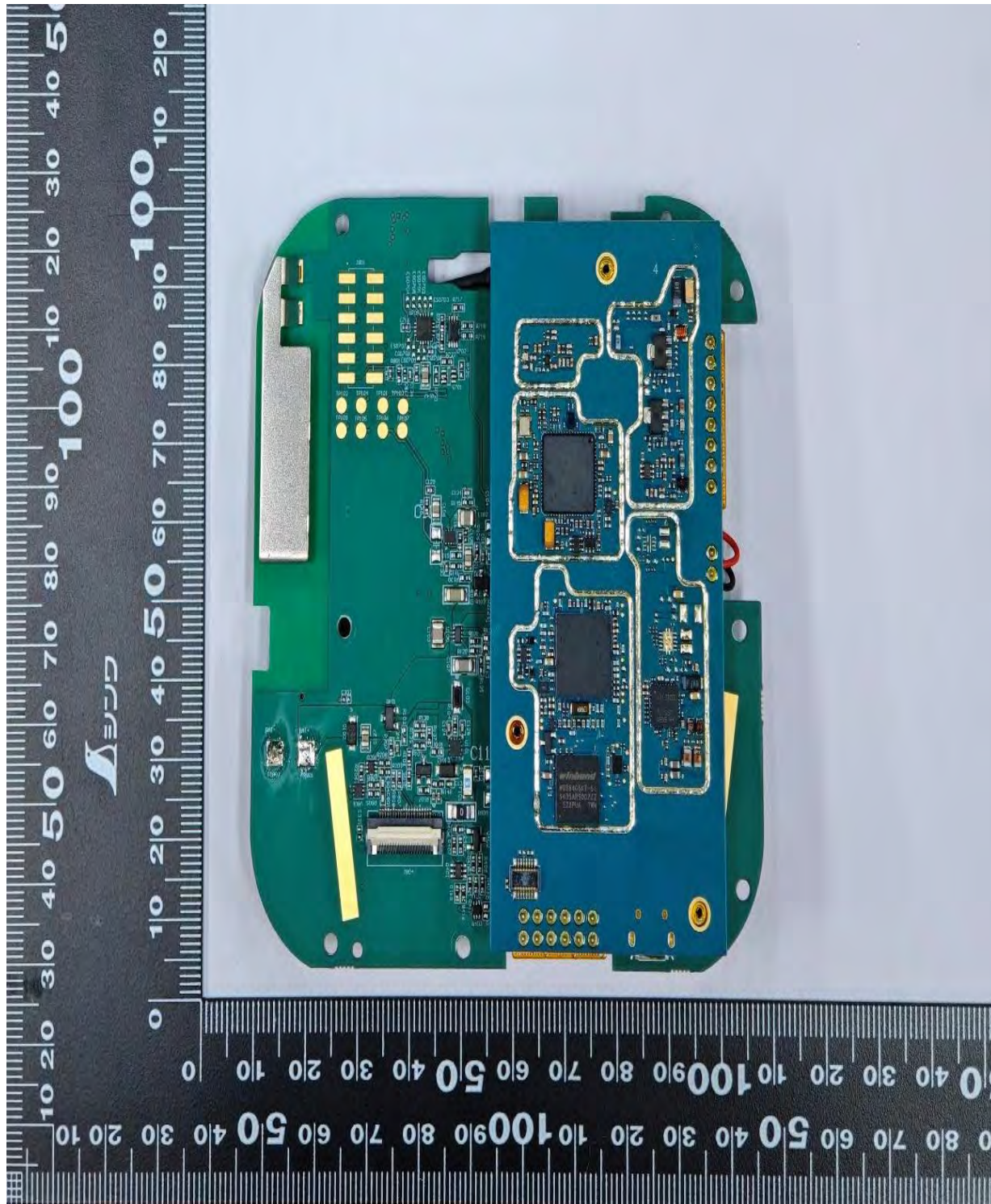
Main Board with RF Board (Bottom) - BSS101NBKLBA (CB900D) CB900D Base Station
