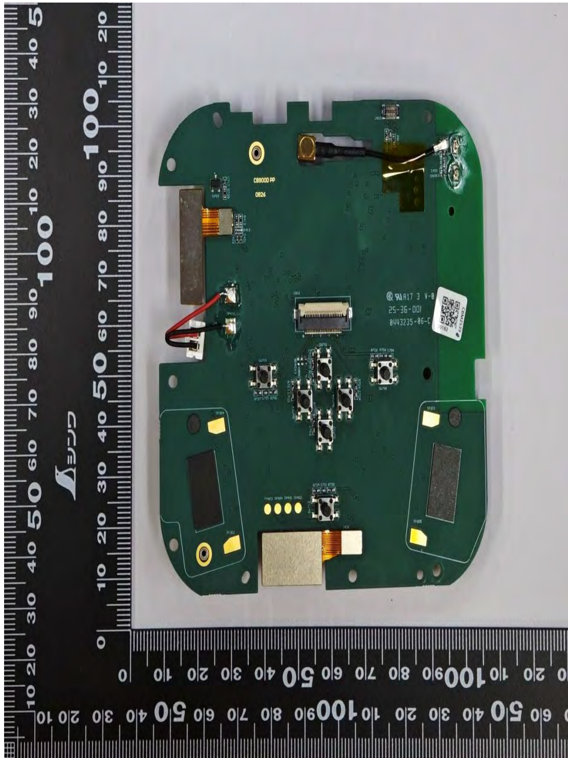
Main Board (Top) - CBS101NBKLBA (CB900D) CB900D 2-Way Call Box
