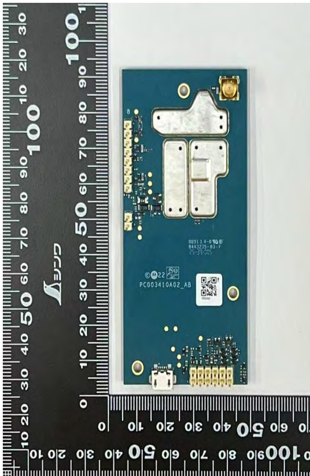
RF Board with Shields (Top) - CBS101NBKLBA (CB900D) CB900D 1-Way Call Box
