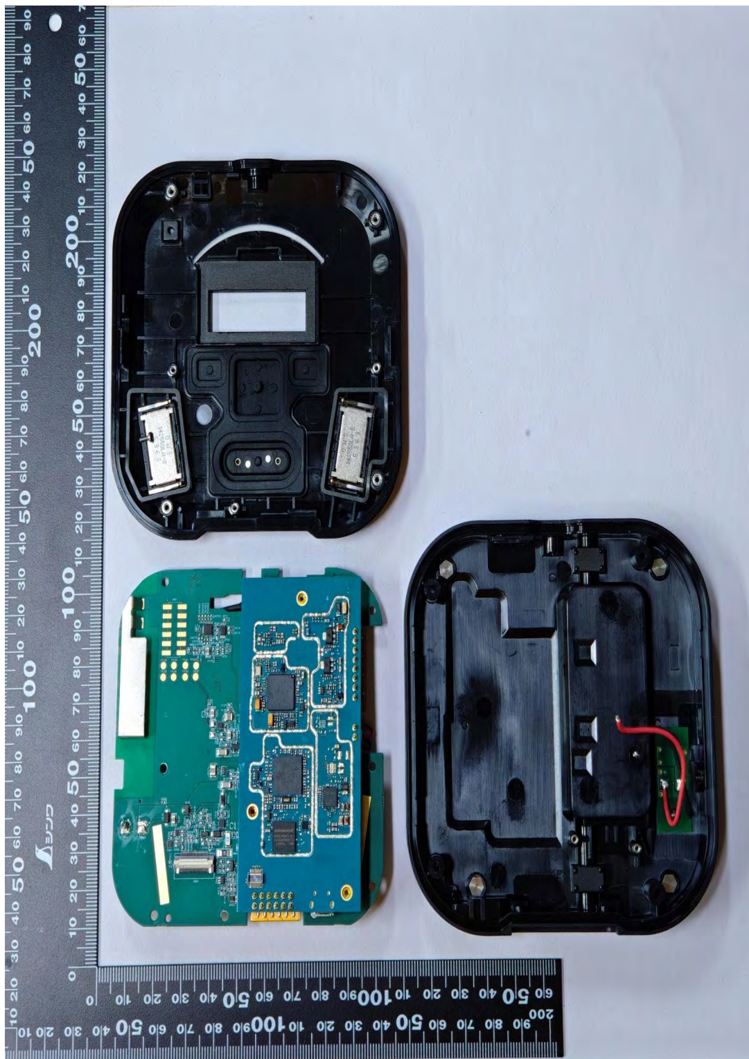
RF Board with Chassis and Housing (Back Side) - BSS101NBKLBA (CB900D) CB900D Base Station
