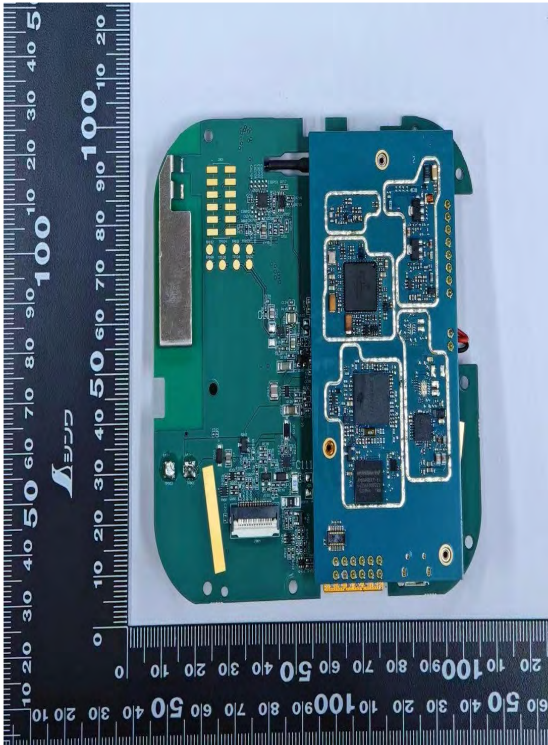
Main Board with RF Board (Bottom) - CBS101NBKLBA (CB900D) CB900D 2-Way Call Box
