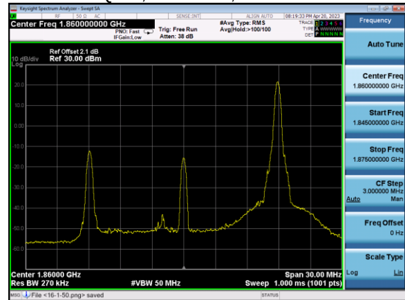
16 QAM, 1 RB size, 99 RB offset
