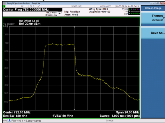
16 QAM, 25 RB size, 49 RB offset
