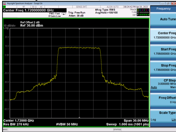
QPSK, 100 RB size, 0 RB offset
