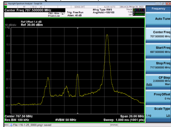
16 QAM, 1 RB size, 49 RB offset
