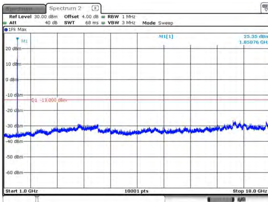
B25_CH26047_1.4M_1RB2_16-QAM_Above 1G
