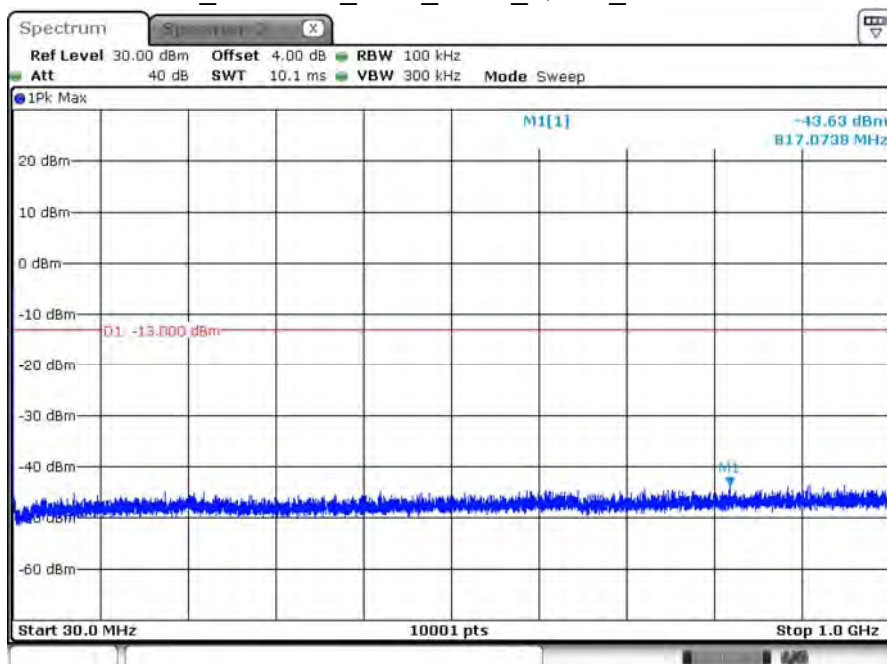
B25_CH26683_1.4M_1RB2_QPSK_Below 1G
