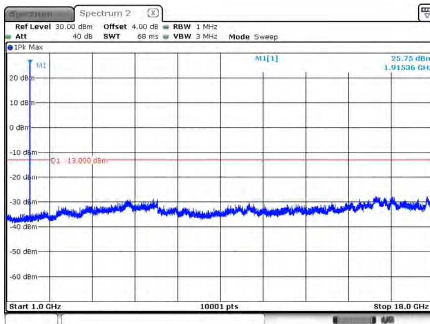
B25_CH26683_1.4M_1RB2_QPSK_Above 1G
