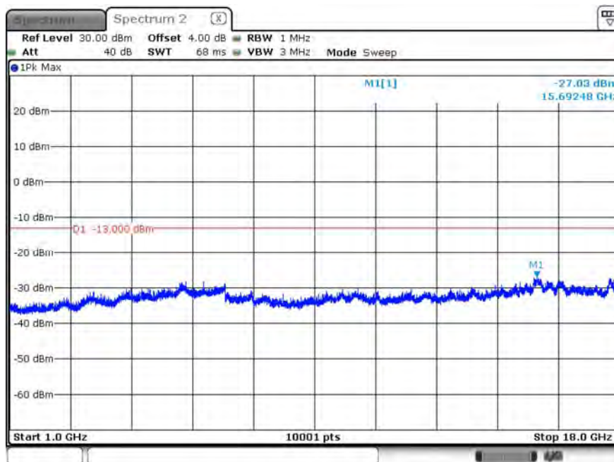
B26_CH26797_1.4M_1RB2_16-QAM_Above 1G (Part 22)
