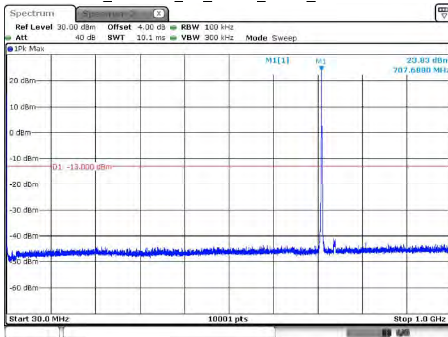
B12_CH23095_5M_1RB12_QPSK_Below 1G
