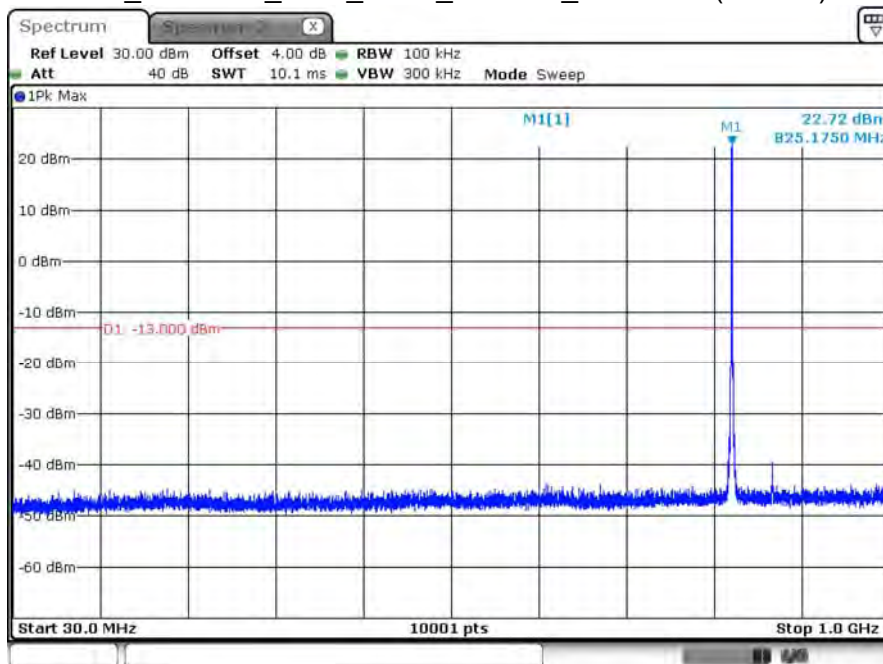
B26_CH26797_1.4M_1RB2_16-QAM_Below 1G (Part 22)
