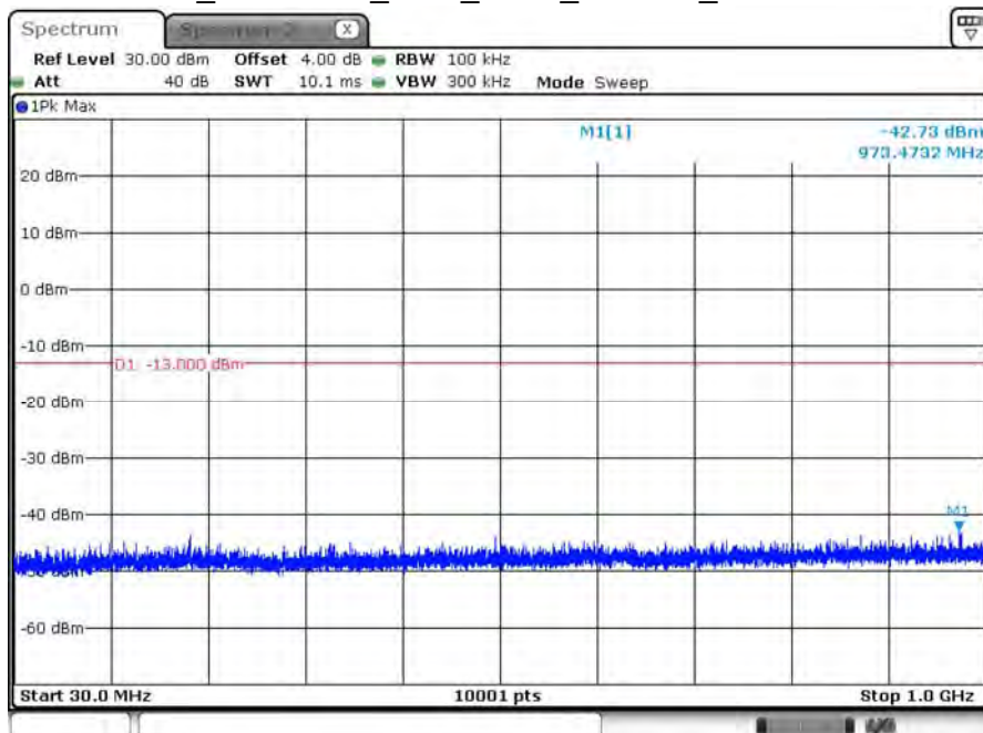
B66_CH131979_1.4M_1RB2_16-QAM_Below 1G
