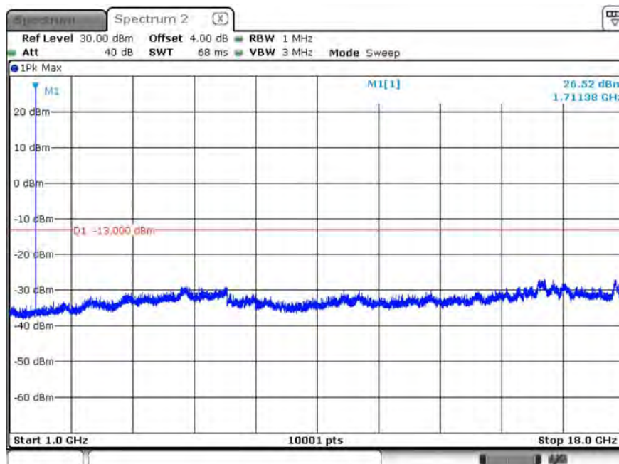
B66_CH131979_1.4M_1RB2_16-QAM_Above 1G
