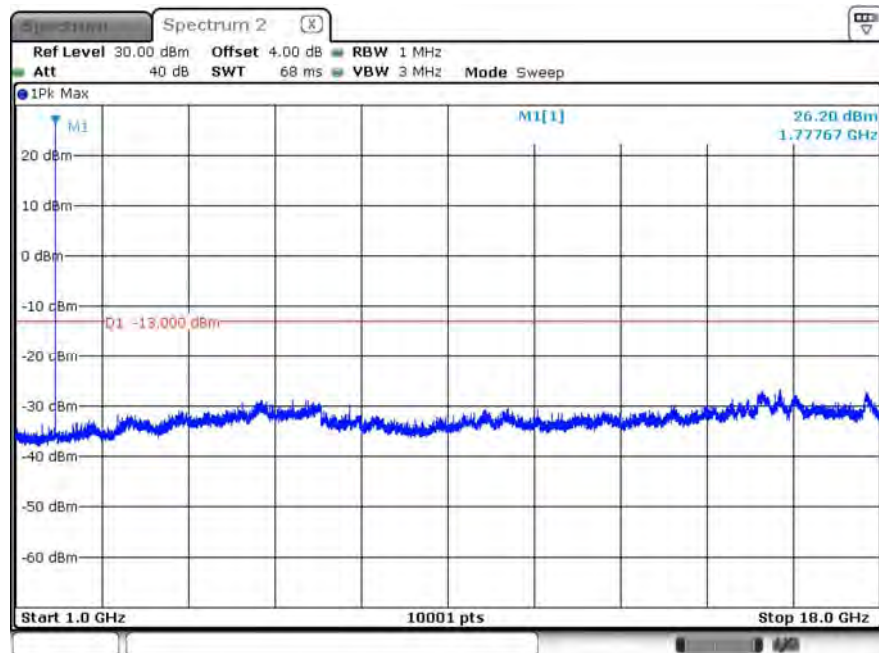
B66_CH132647_5M_1RB12_16-QAM_Above 1G
