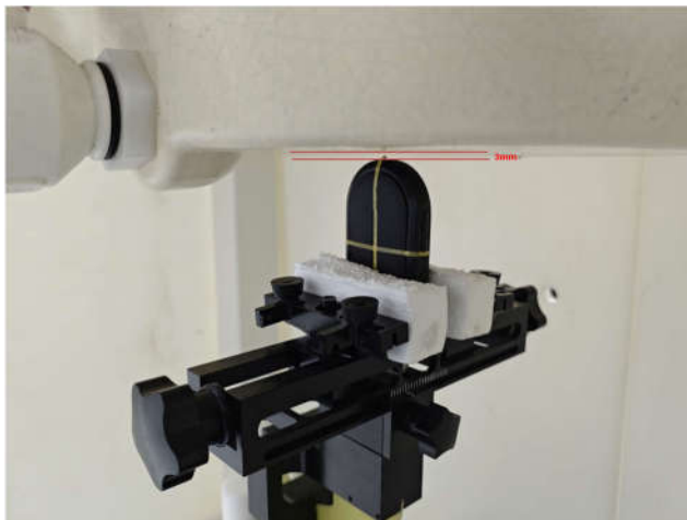
Bottom Side, Test Separation 3 mm(Sensor off)
