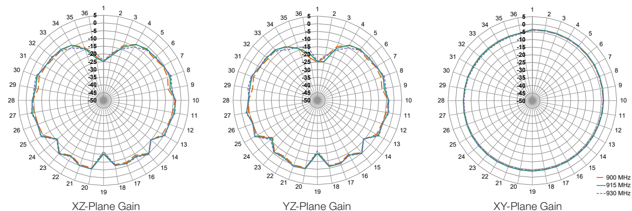
Figure 16. Radiation Patterns for ANT-915-NUB-ccc Antenna in Free Space
