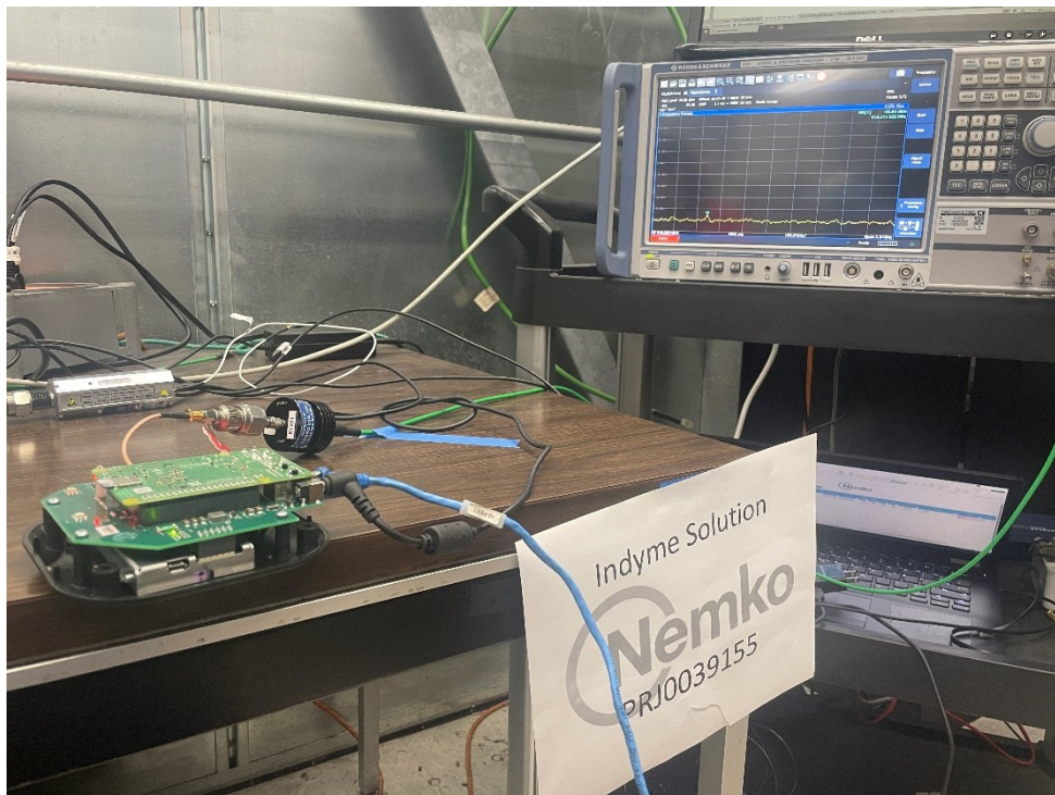
Figure 11 – Test setup: antenna conducted port.
