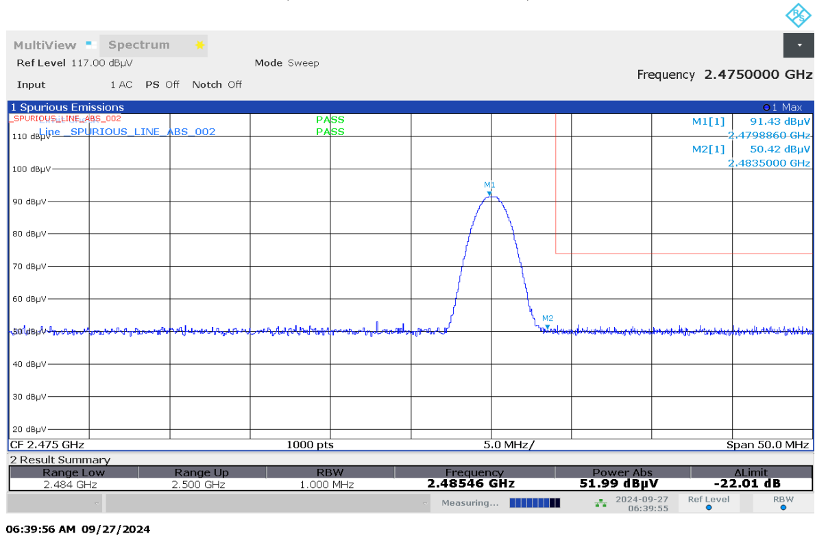
Restricted Band Edge (High Channel, Vertical, Peak) graphical screen shot
