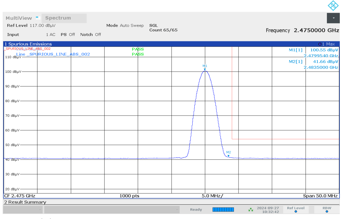
Restricted Band Edge (High Channel, Horizontal, Average) graphical screen shot
