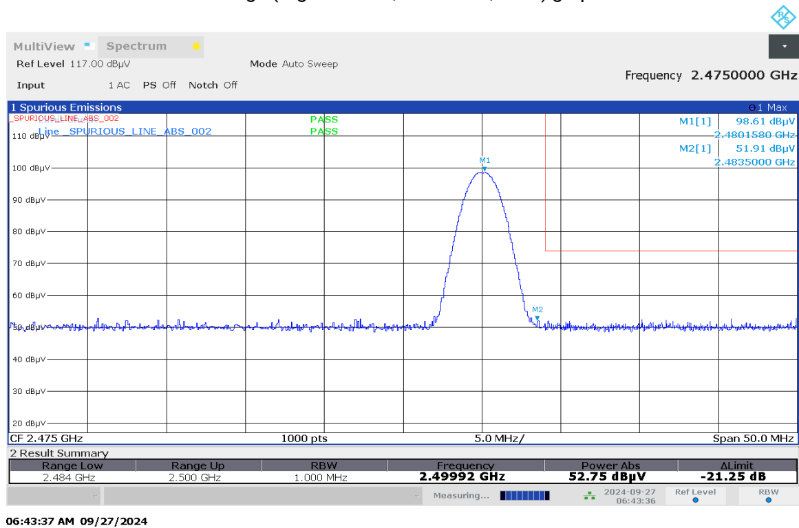
Restricted Band Edge (High Channel, Horizontal, Peak) graphical screen shot
