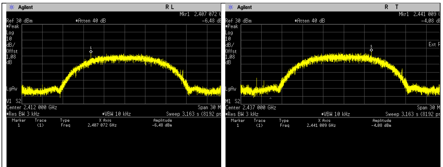
Maximum Power Spectral Density. 802.11b Frequency 2412 MHz
