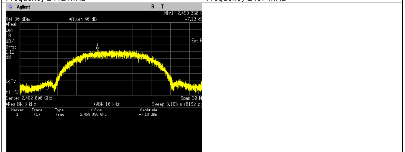
Maximum Power Spectral Density. 802.11b Frequency 2462 MHz
