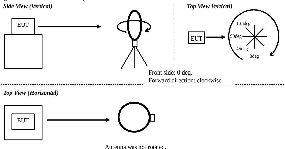
Figure 2. Antenna angle
