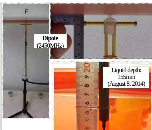
Test setup for the system performance check
