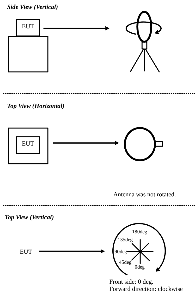
Figure 2: Direction of the Loop Antenna
