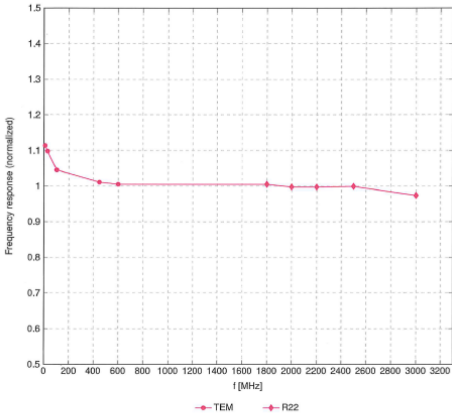
Frequency Response of E-Field (TEM-Cell:ff1110 EXX, Waveguide:R22)
