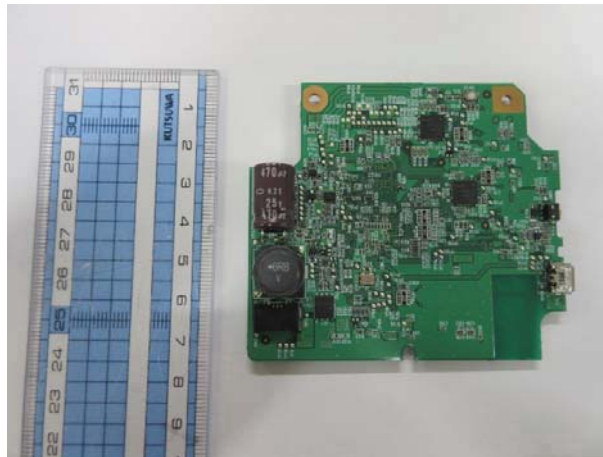
MAIN PCB (WLAN MODULE) – Bottom side –
