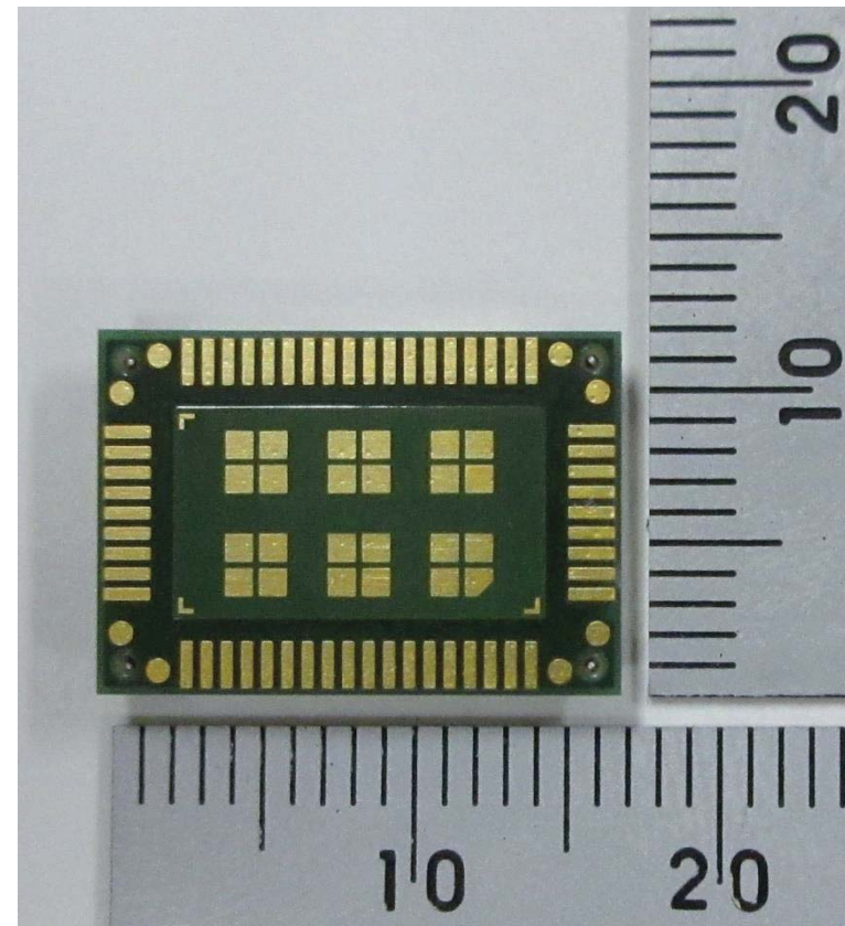
Bottom view
