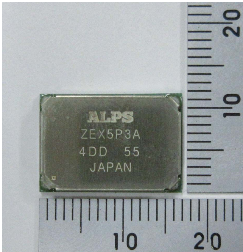
Top view
