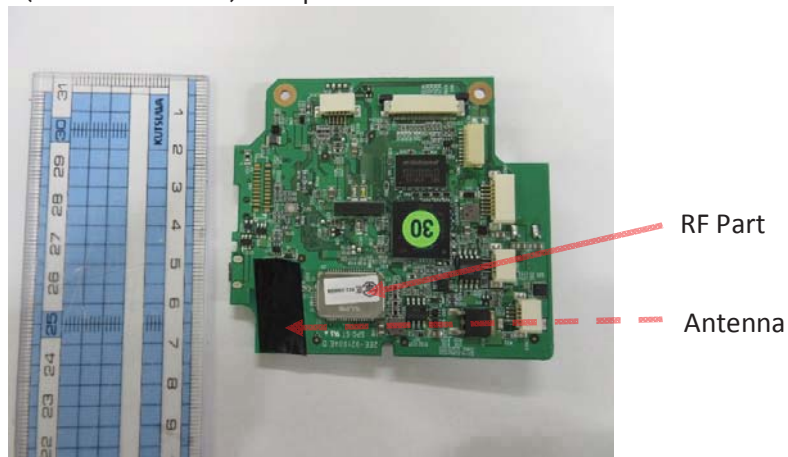
MAIN PCB (WLAN MODULE) – Top side –
