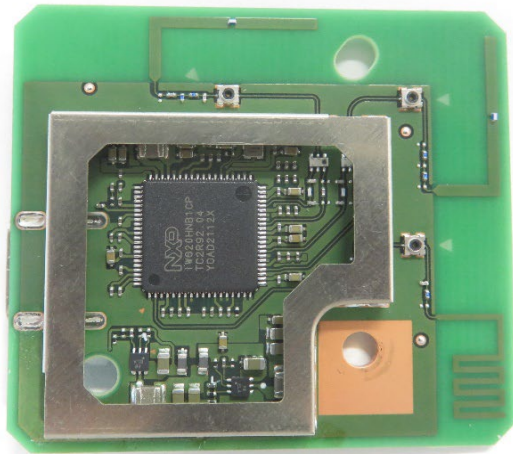
Top side View with Shield Cover (Open)
