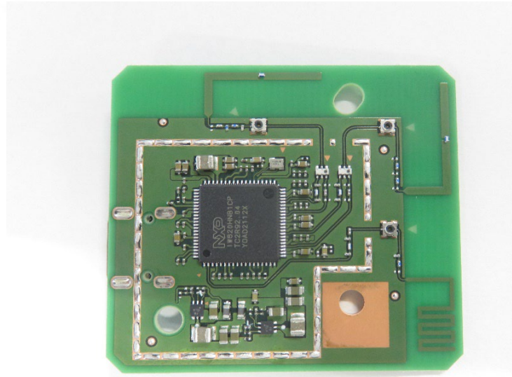
Top side View without Shield Cover
