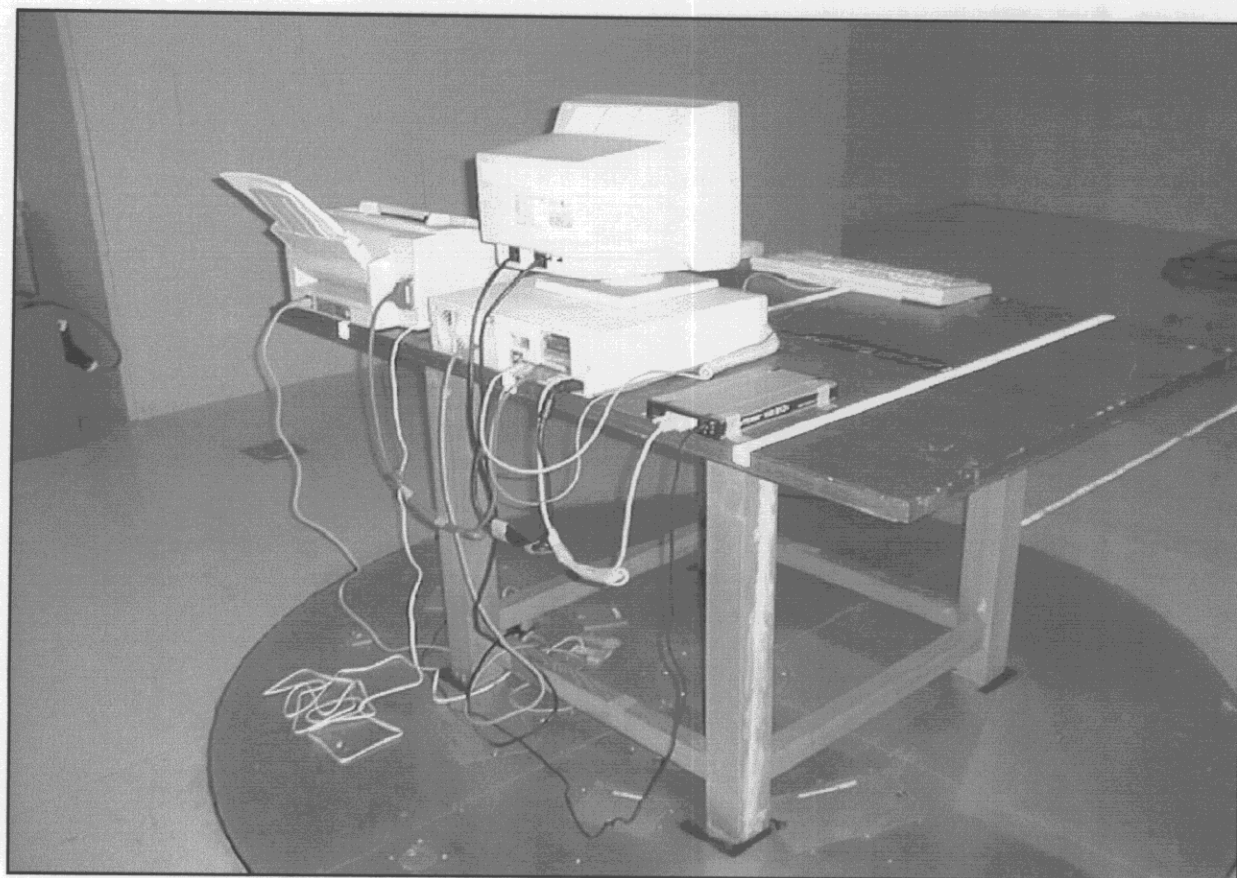
背面(放射ノイズ測定時) Rear View (Radiation)
