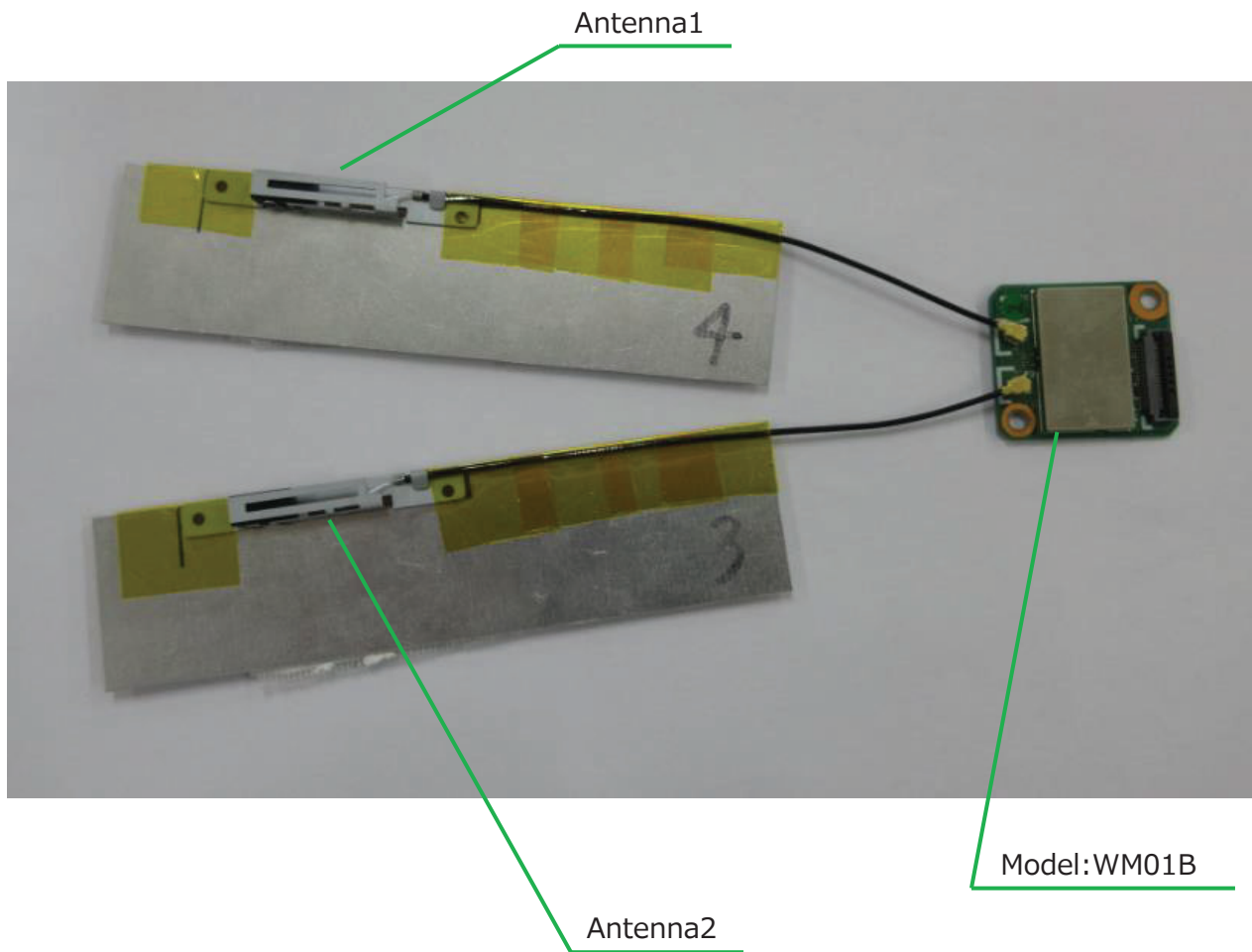
Connection photo of WM01B and antenna (antenna 1, antenna 2)
