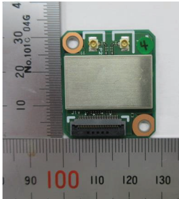
Front (with shielding case)
