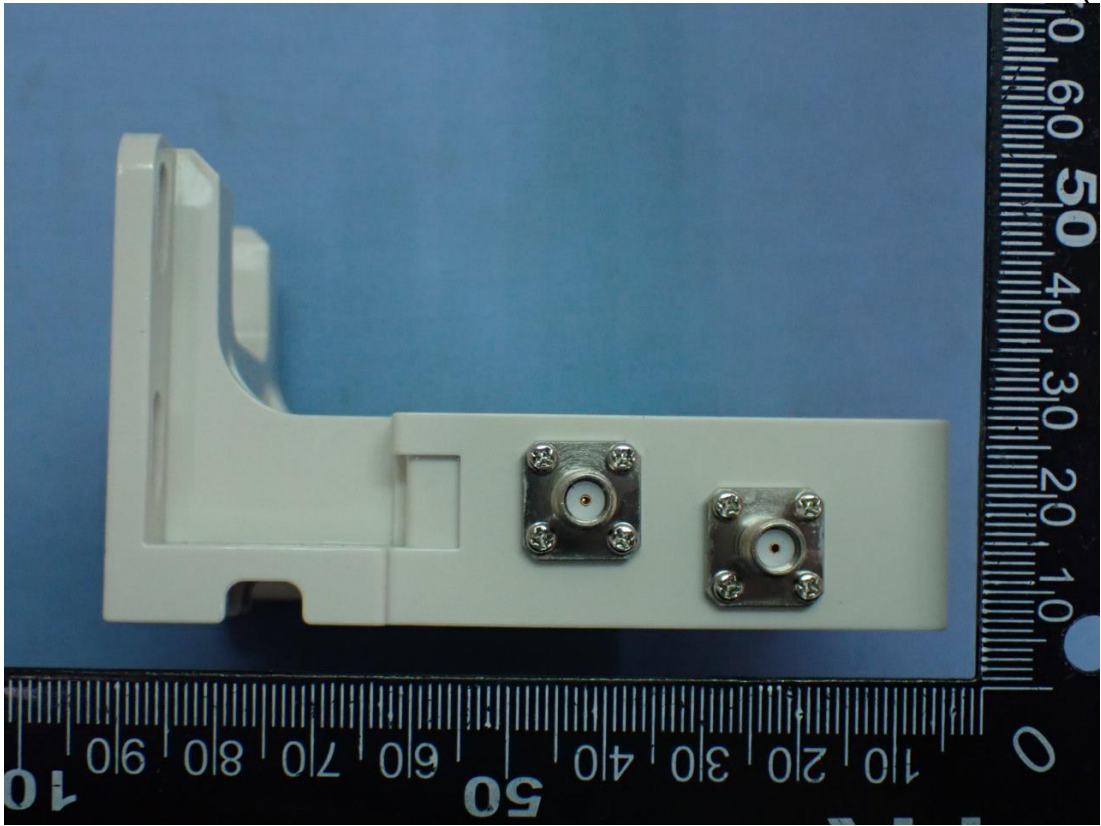
Figure 15 Antenna#2 (Side View)
