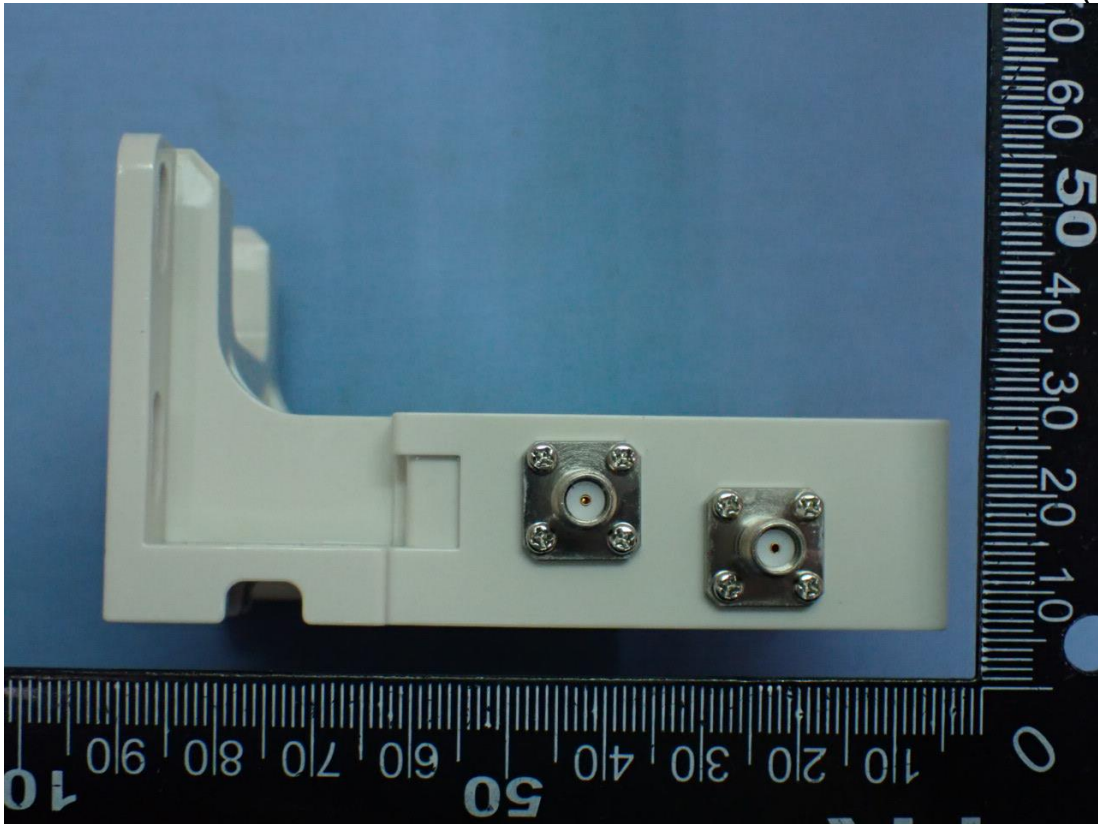
Figure 9 Antenna#1 (Side View)
