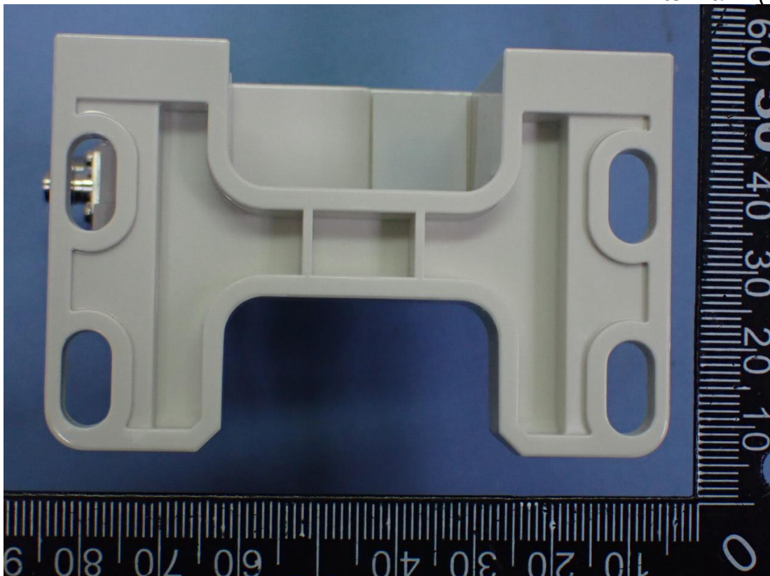
Figure 18 Antenna#2 (Side View)
