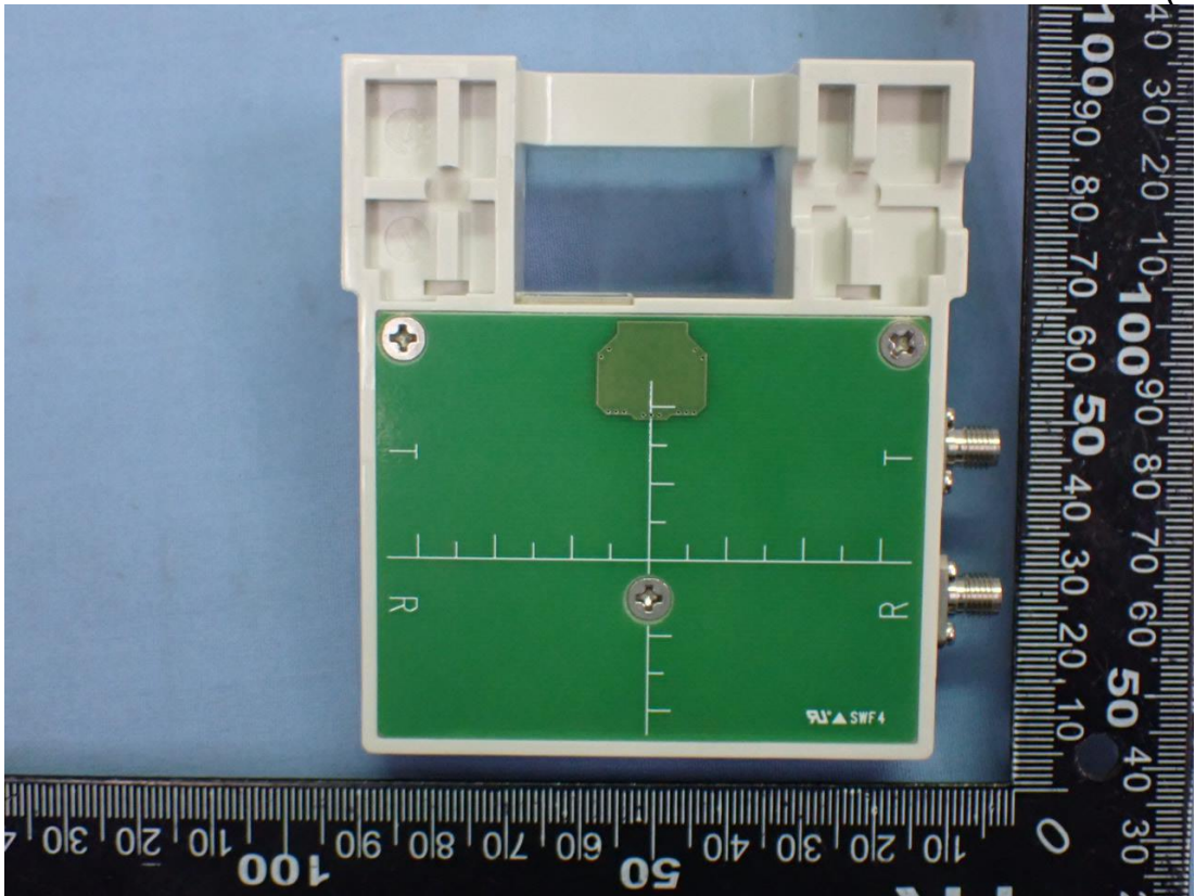
Figure 14 Antenna#2 (Back View)
