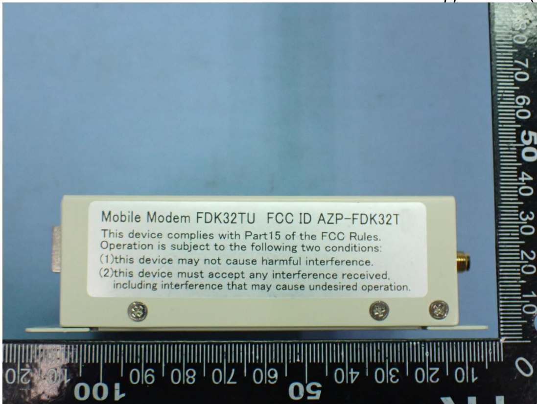
Figure 3 General Appearance (Side View)
