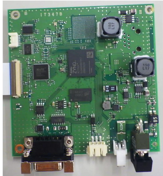
RF board Bside
