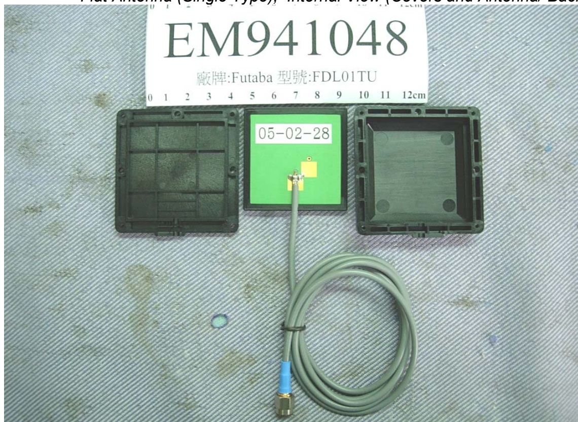
Figure 16 Flat Antenna (Single Type), Internal View (Covers and Antenna/ Back View)
