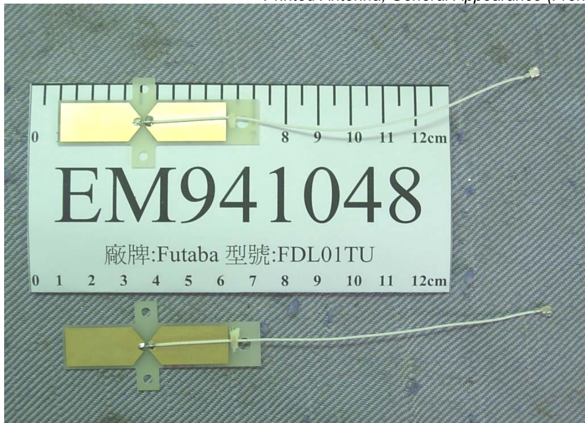
Printed Antenna, General Appearance (Front View)
