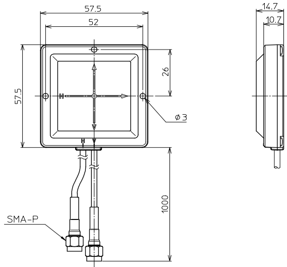
5 Flat antenna(double type) FAA01EJ010 (Part Number:1M38A09201) 2.14dBi
