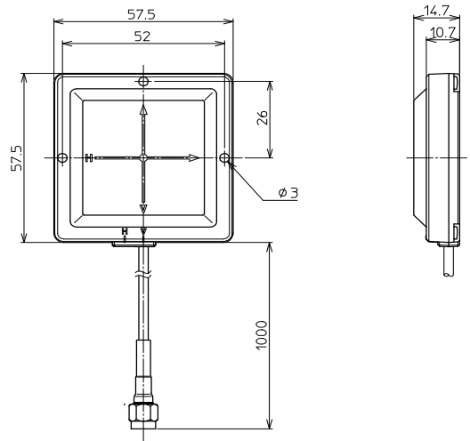
4 Flat antenna(single type) FAA02EJ010 (Part Number:1M38A09202) 2.14dBi
