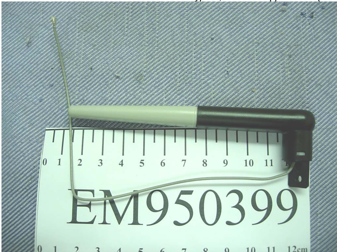
Figure 13 Antenna Type B, General Appearance (Side View)
