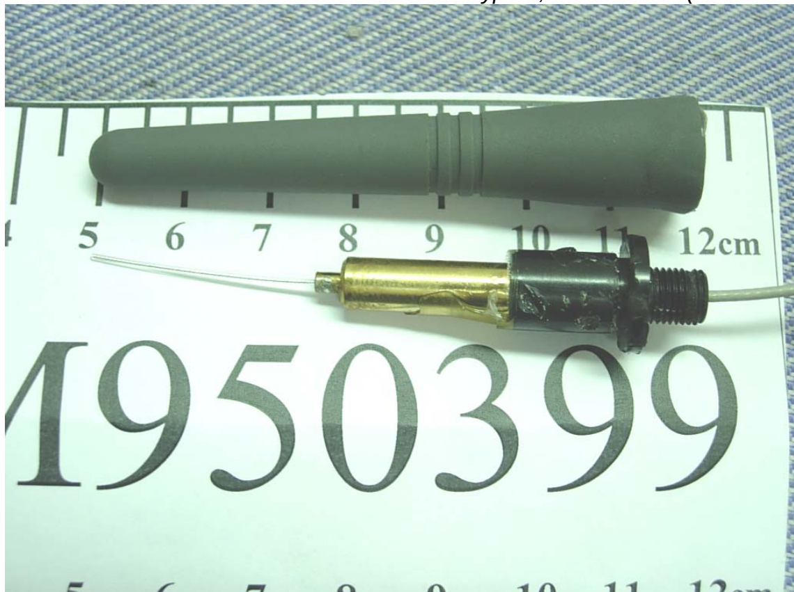
Figure 12 Antenna Type A, Internal View (Cover Removed)
