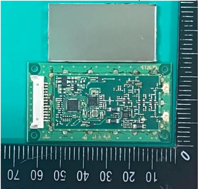
Figure 5 Internal View (Removed Cover)
