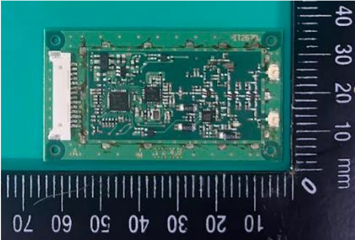
Figure 6 Internal View
