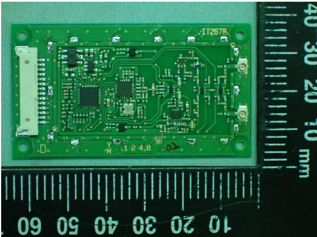
Figure 5 Internal View
