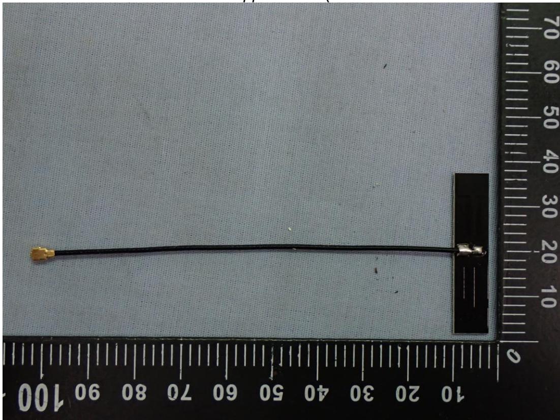
Figure 9 General Appearance (STDANTEMD-013 Antenna/Front View)
