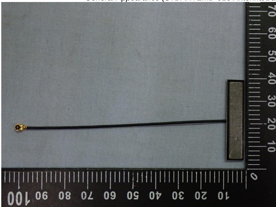
Figure 12 General Appearance (STDANTEMD-013 Antenna/Back View)
