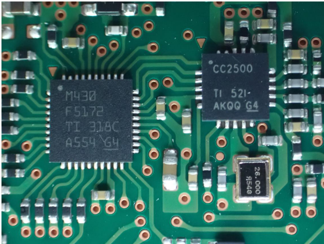
Figure 19 Internal View (Chip)
